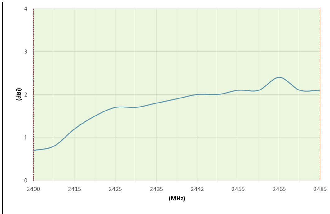
c) Peak Gain (dBi)
