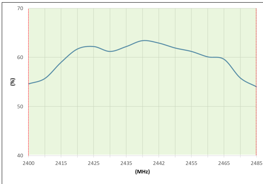
c) Efficiency (%)
