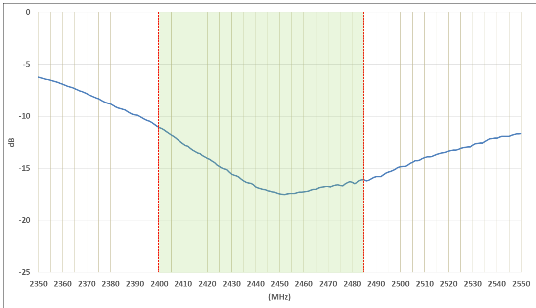
a) Return loss (dB)
