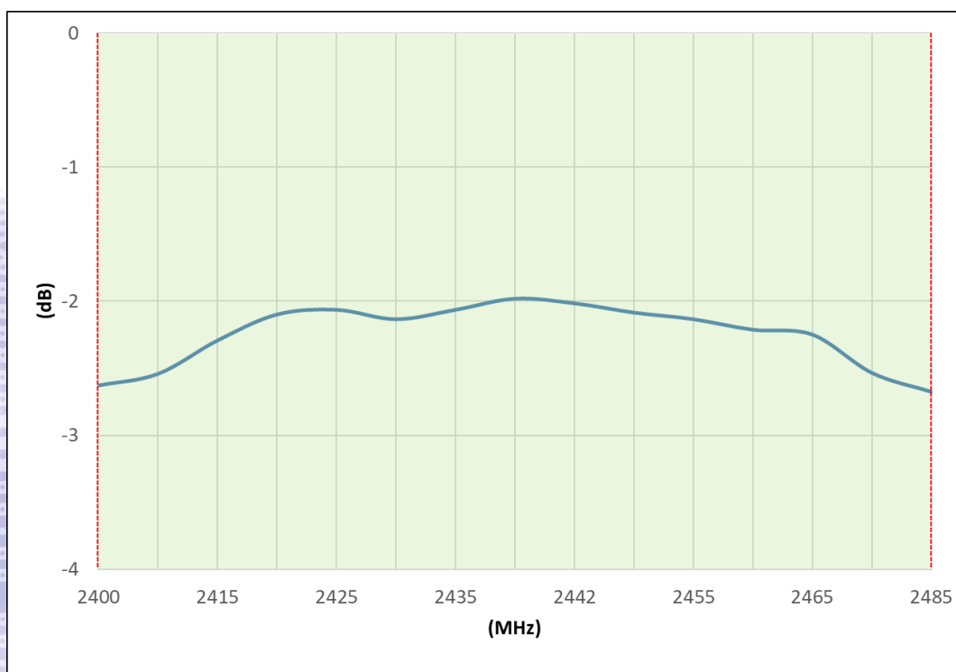
b) Average Gain (dB)
