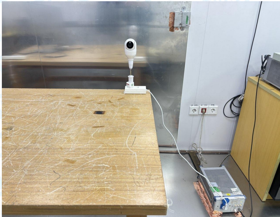
Photo of Setup for Conducted Emission
