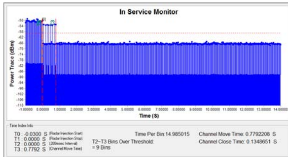
Central Frequency: 5610 MHz
