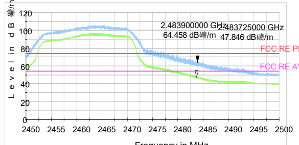
802.11n HT20 -Channel 11 Peak+ Average
