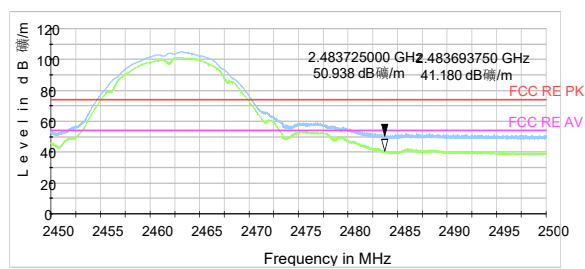
802.11b-Channel 11 Peak+ Average
