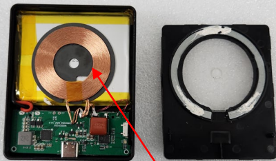
Coil Antenna
