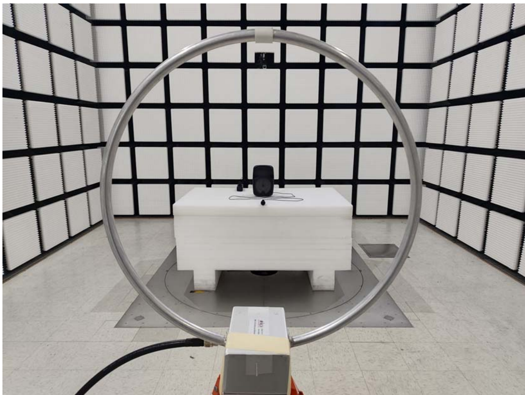
Radiated Emission Below 1GHz View Parallel
