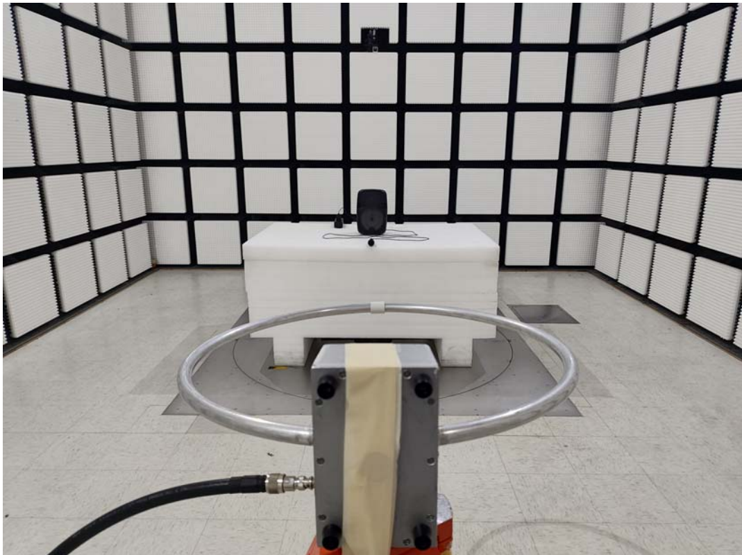
Radiated Emission Below 1GHz View Ground-parallel
