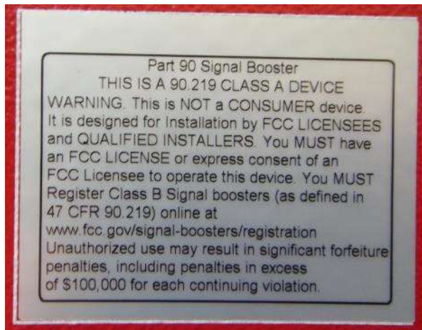
Figure 7: Labels view
