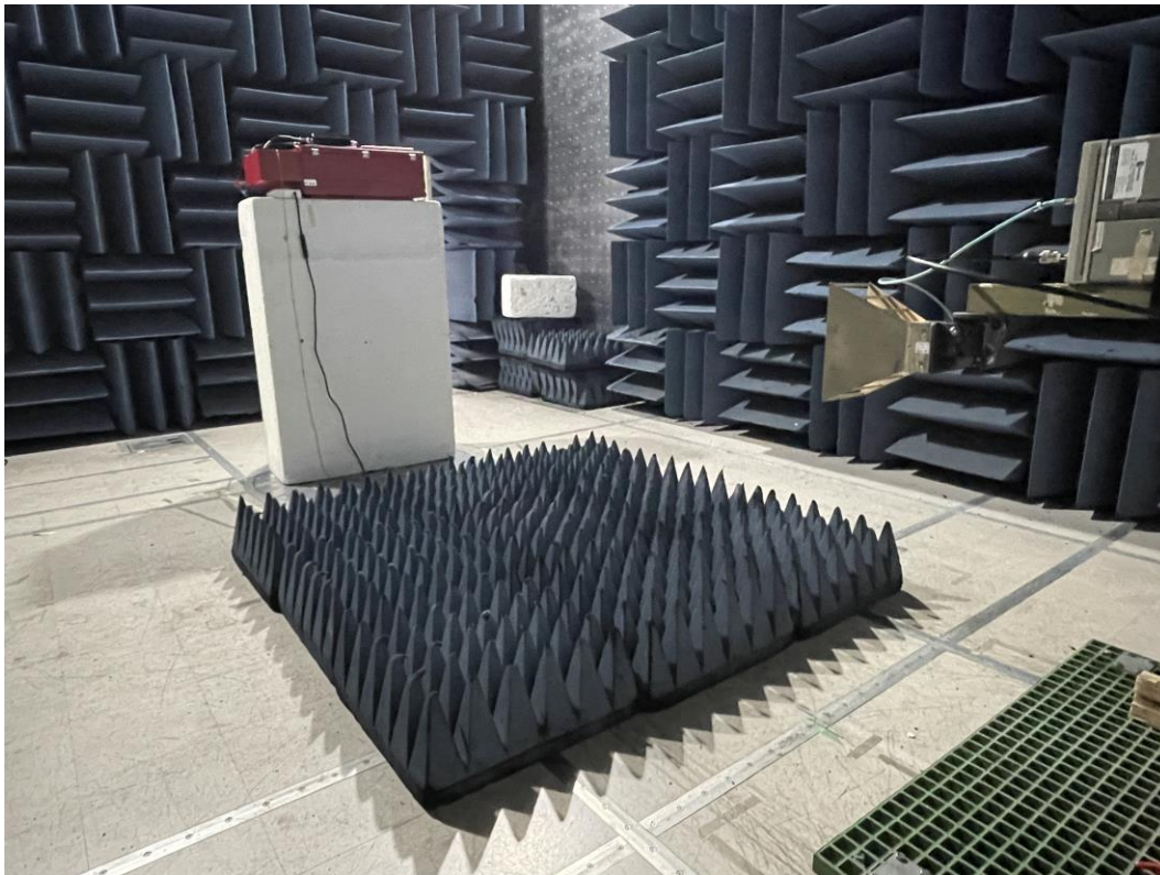
Figure 4. Radiated Emissions Test Setup (Above 1 GHz)
