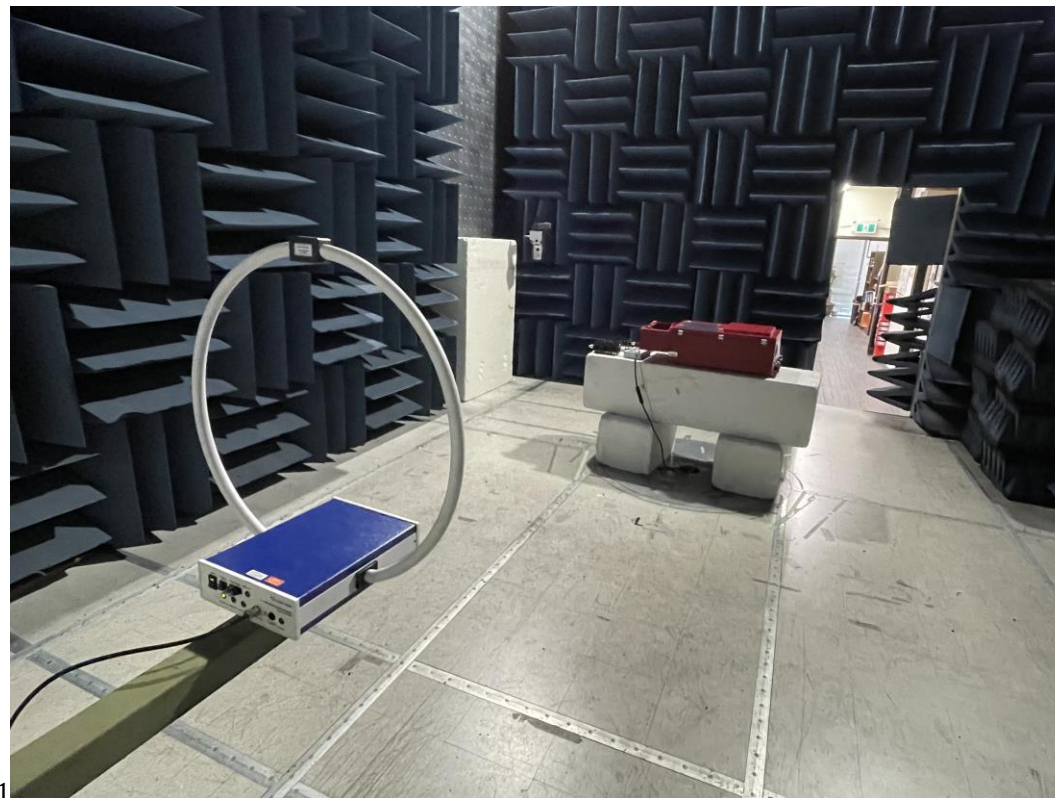
Figure 2. Radiated Emissions Test Setup (Below 30 MHz)
