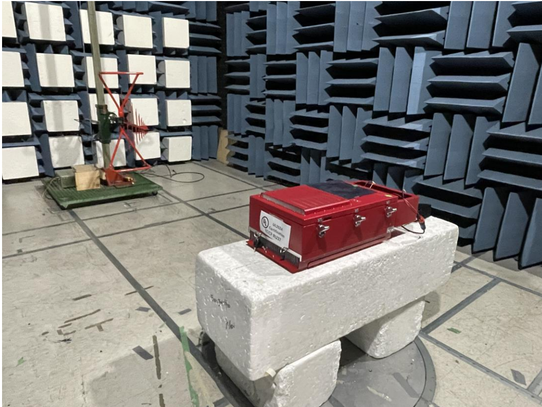
Figure 3. Radiated Emissions Test Setup (30 MHz to 1 GHz)
