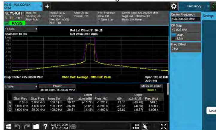
415PS CQPSK Signal at 425MHz
