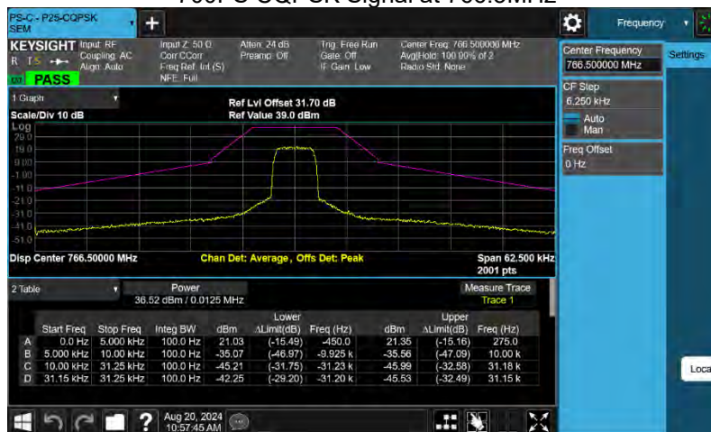
700PS CQPSK Signal at 766.5MHz
