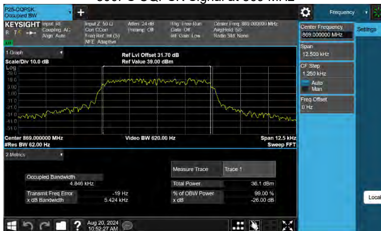
800PS CQPSK Signal at 869 MHz
