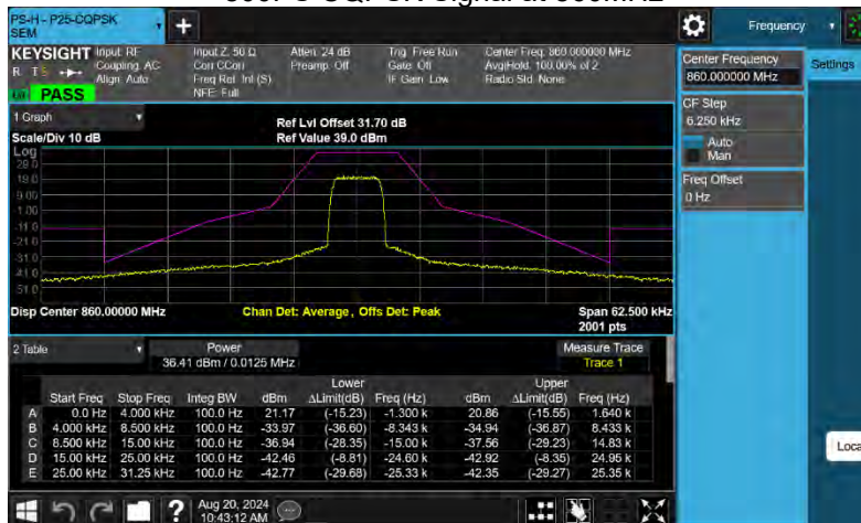
800PS CQPSK Signal at 860MHz
