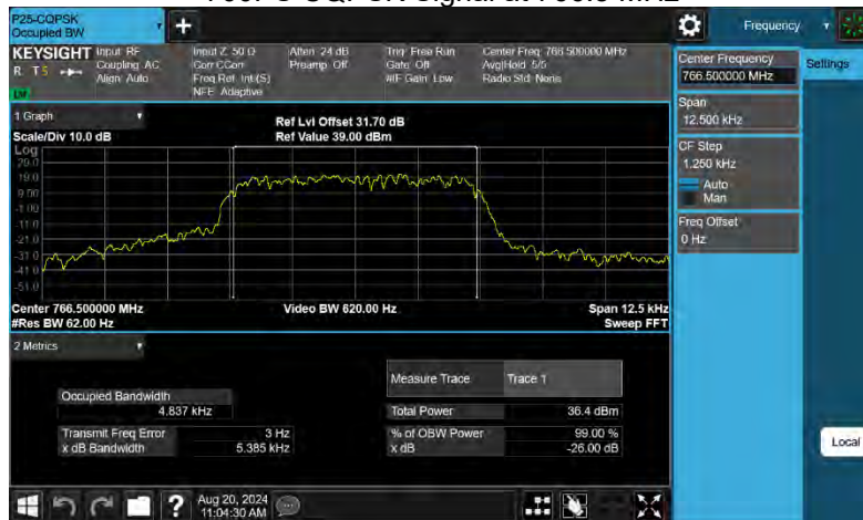
700PS CQPSK Signal at 766.5 MHz
