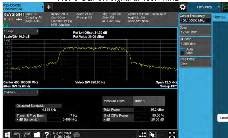
415PS CQPSK Signal at 406.1 MHz
