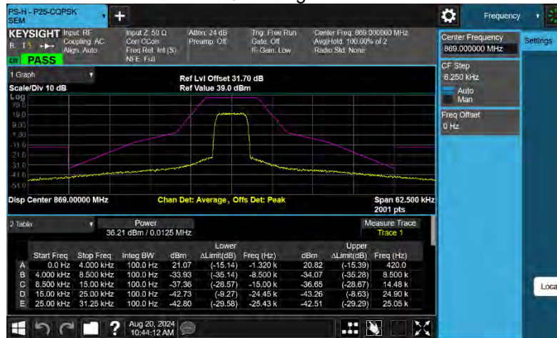
800PS CQPSK Signal at 869MHz
