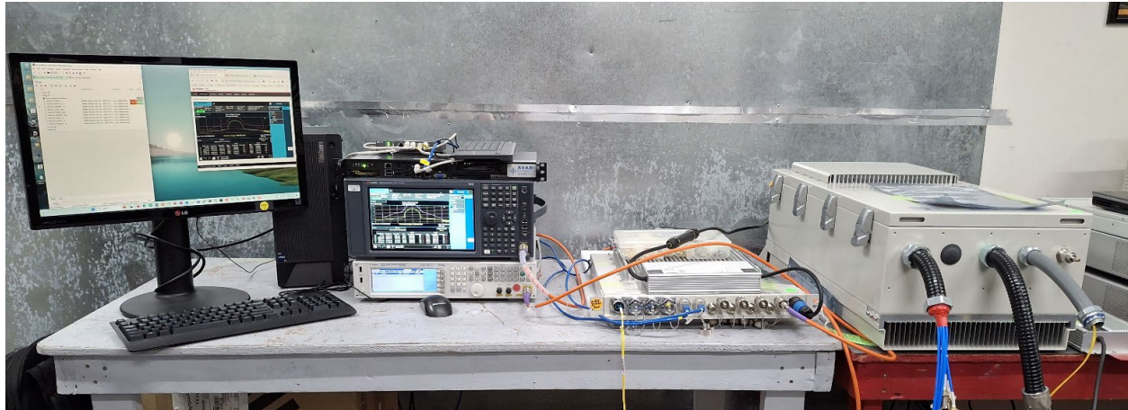
Figure 1: Conductive Emissions Test Setup
