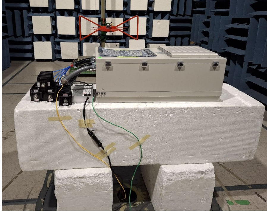
Figure 3: Radiated Emissions (30 MHz- 1GHz) Emissions Test Setup
