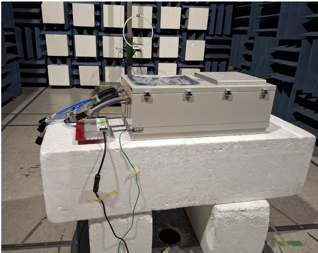
Figure 2: Radiated Emissions (Below 30 MHz) Emissions Test Setup
