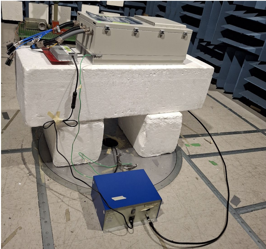
Figure 5: Conducted Test Setup – EUT
