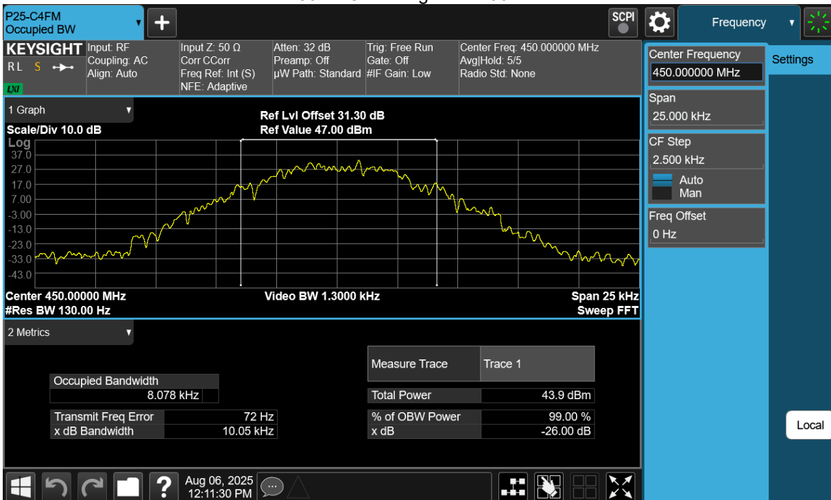
450PS C4FM Signal at 450 MHz
