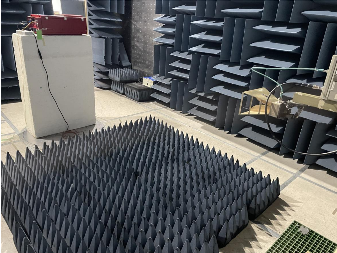
Figure 4: Radiated Emissions Test Setup above 1 GHz
