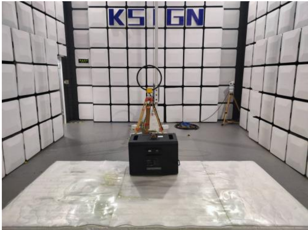
Emissions in restricted frequency bands (below 30MHz)
