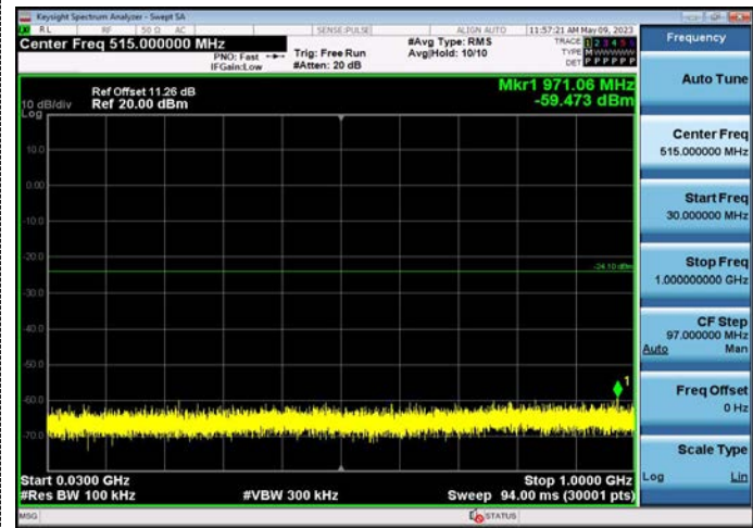
30MHz-1GHz
