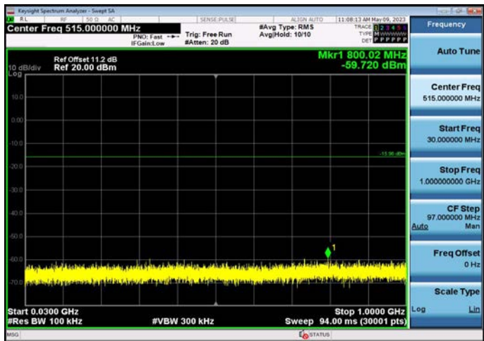
30MHz-1GHz
