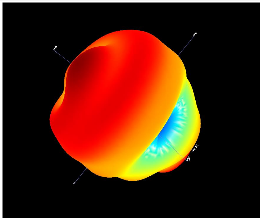
B1.3 3D Pattern for 440MHz
