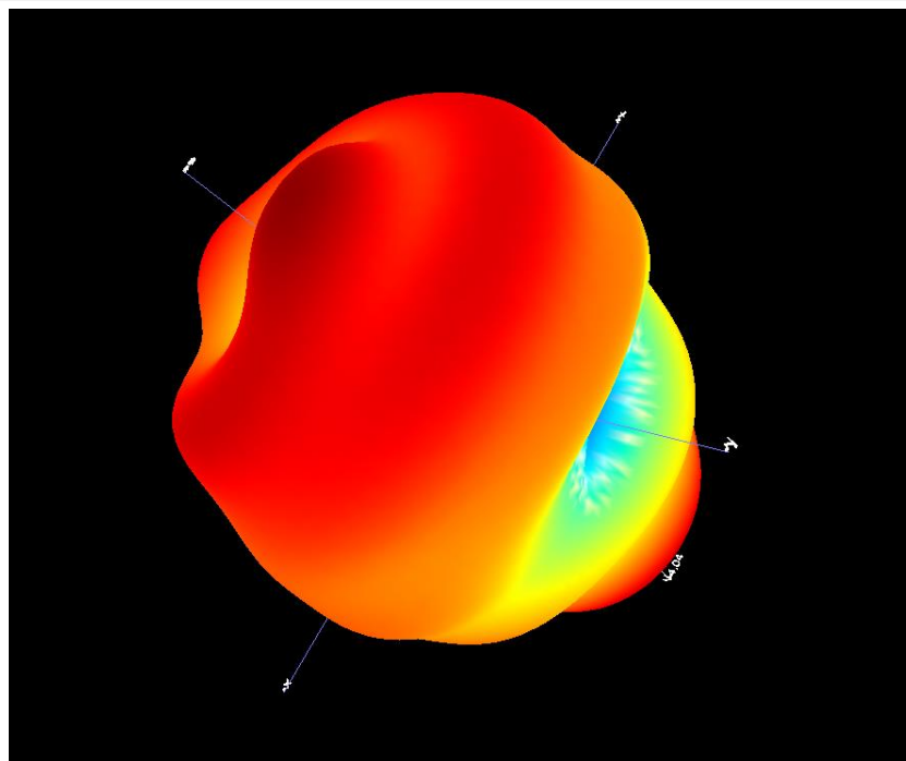
B1.2 3D Pattern for 435MHz
