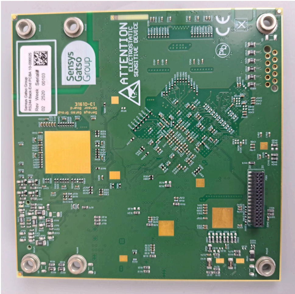
10-000025-02 back
