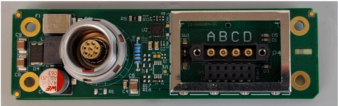
10-000026-01 back
