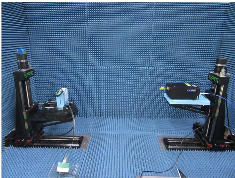
Photograph 7: Set-up photo for Radiated Spurious Emission, 110GHz - 140GHz
