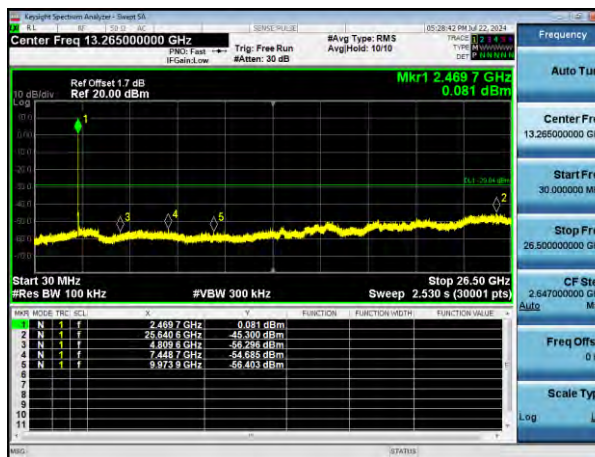
Spurious Emissions
