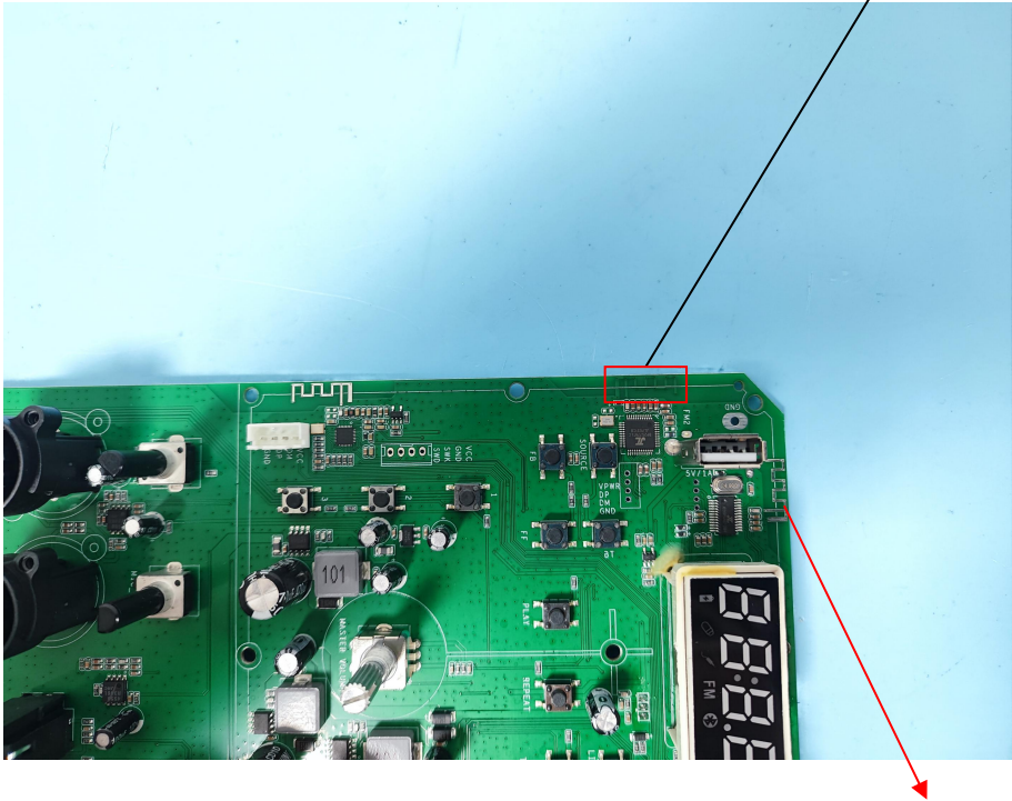
Antenna location(EDR Antenna 2)
