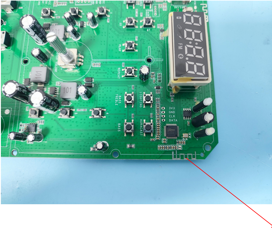
Antenna location(BLE Antenna)
