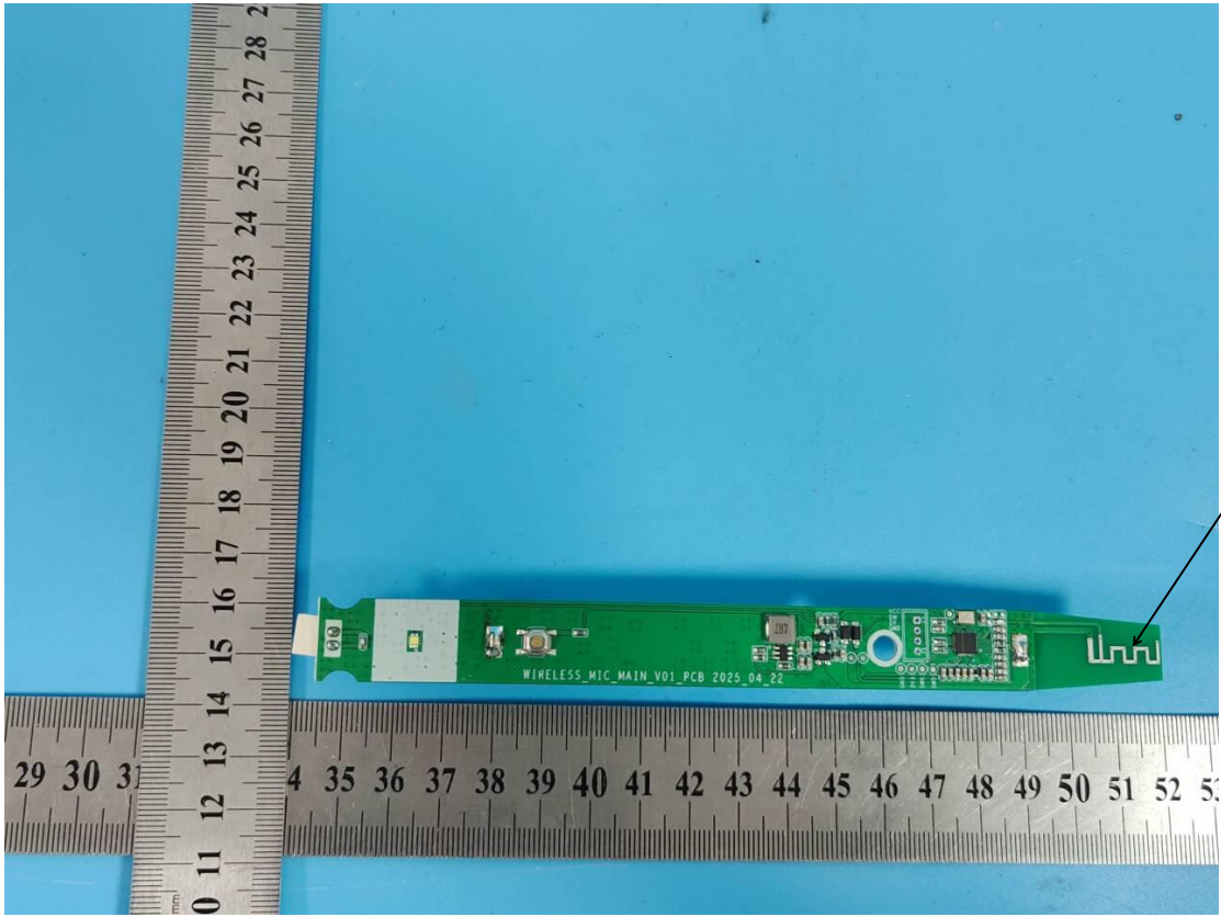
INTERNAL PHOTO OF SAMPLE PCB
