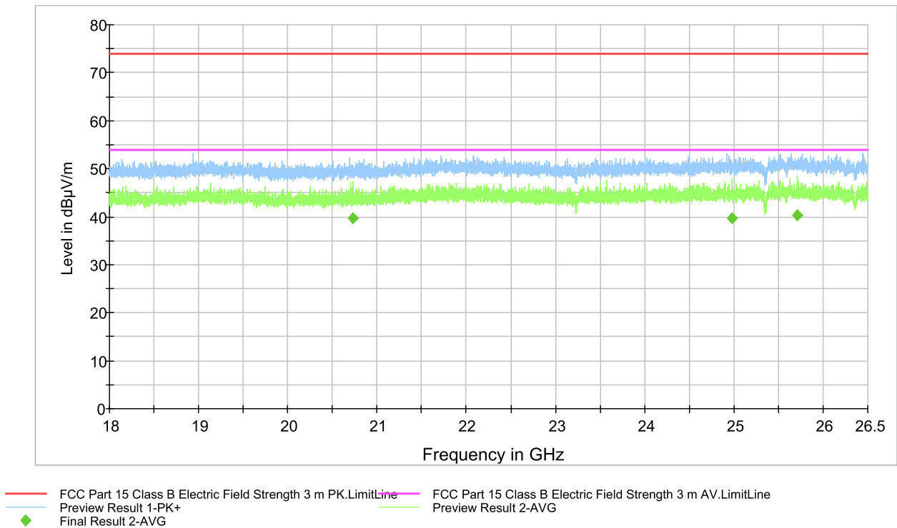
Figure 13. Measured curve with peak- and average detector. Channel LOW.
