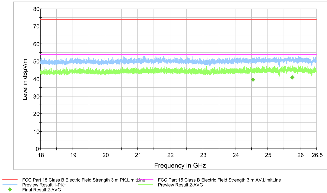
Figure 35. Measured curve with peak-and average detector.
