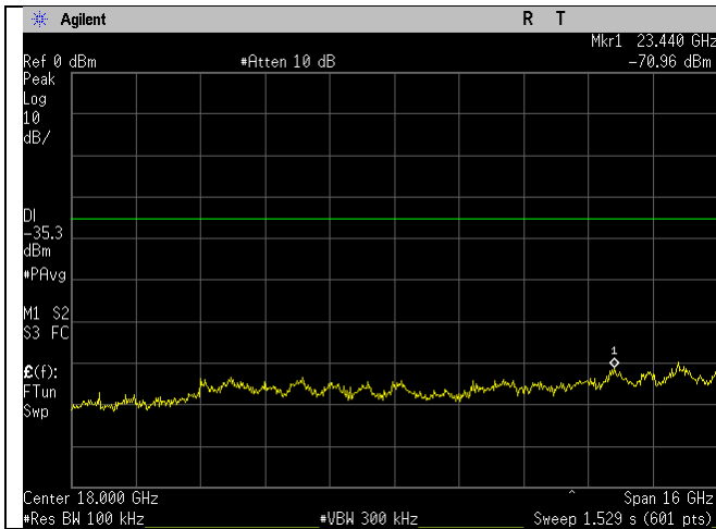
2462MHz_g-mode_10-26GHz
