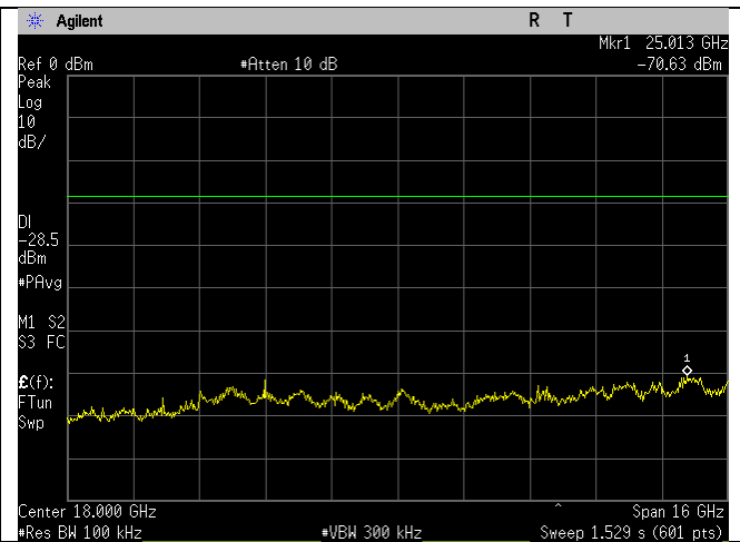
2462MHz_b-mode_10-26GHz
