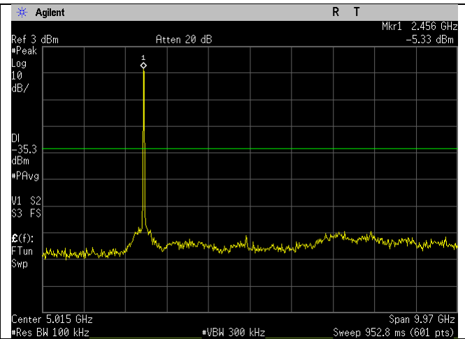
2462MHz_g-mode_30MHz-10GHz
