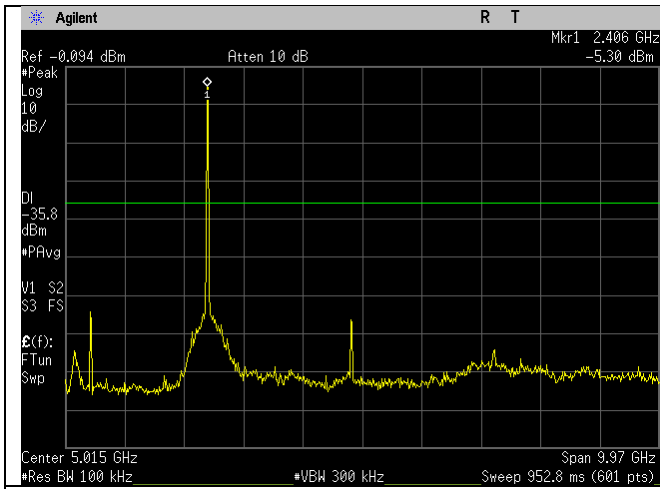
2412MHz_g-mode_30MHz-10GHz
