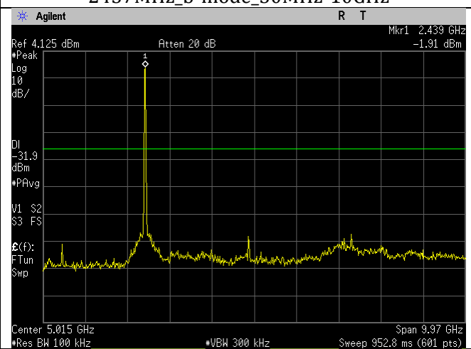
2437MHz_g-mode_30MHz-10GHz
