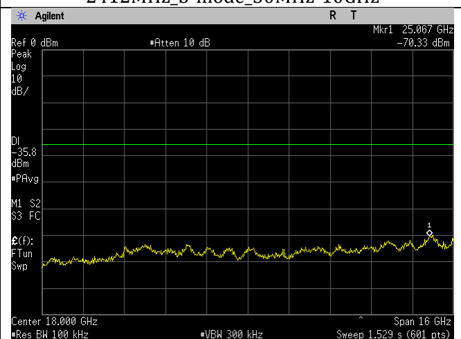
2412MHz_g-mode_10-26GHz
