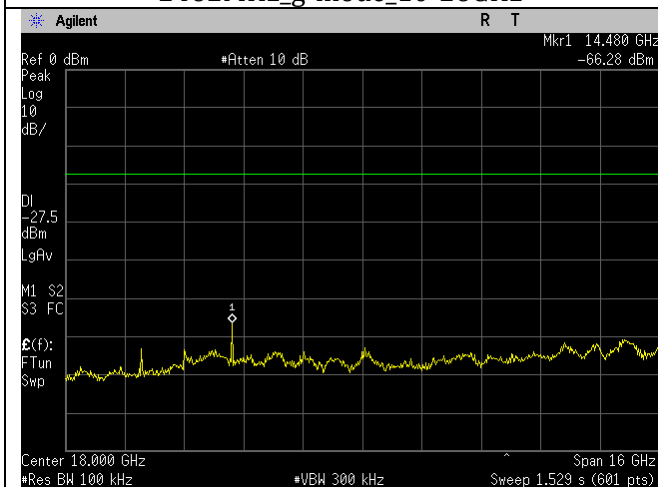
2412MHz_b-mode_10-26GHz
