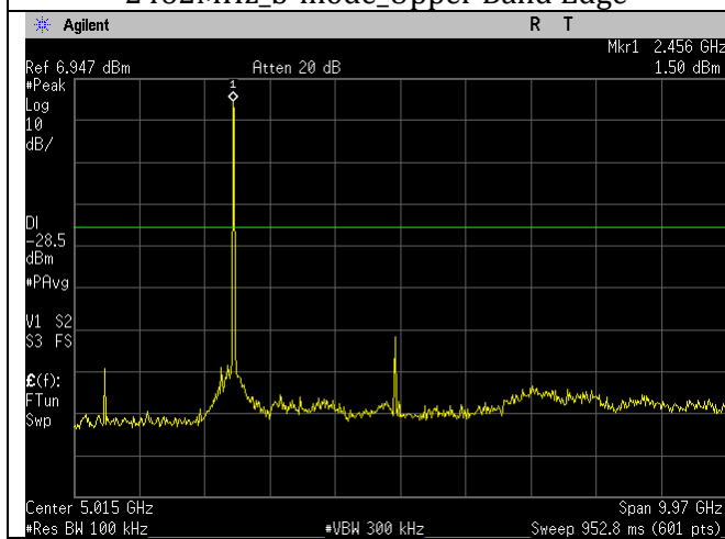
2462MHz_b-mode_30MHz-10GHz
