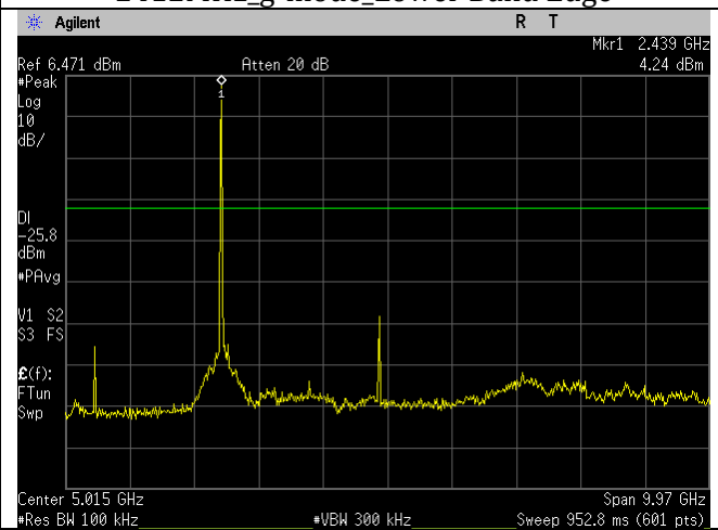
2437MHz_b-mode_30MHz-10GHz
