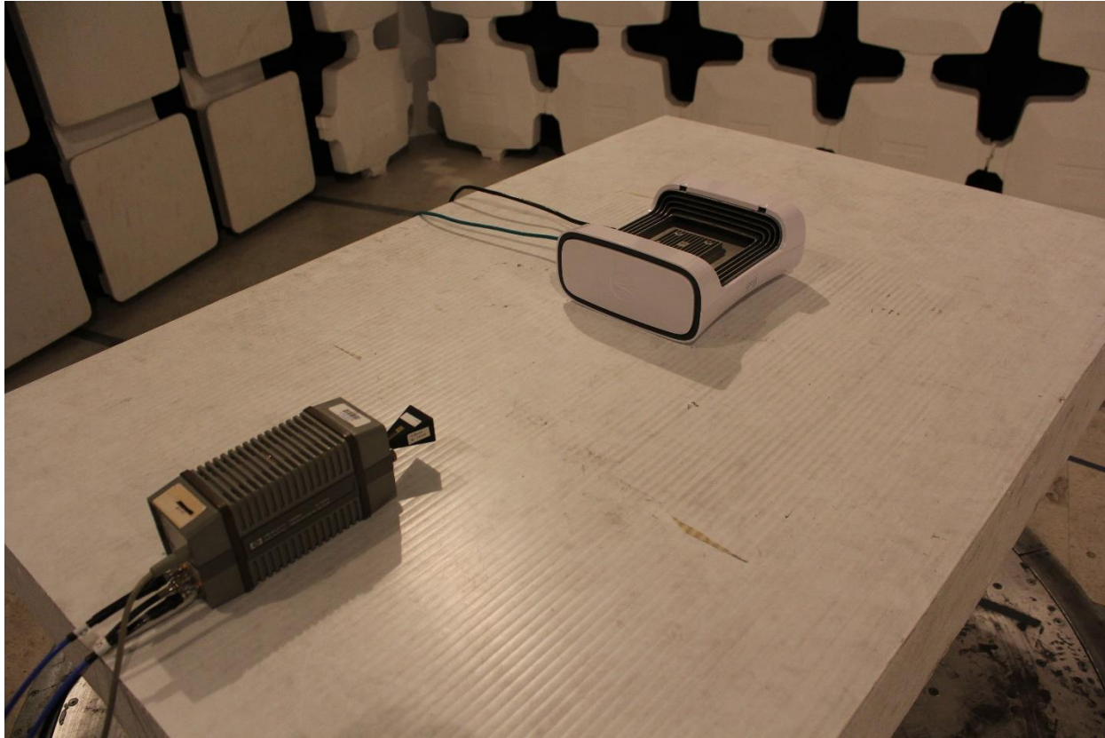
60 GHz Test Setup 0.4m distance
