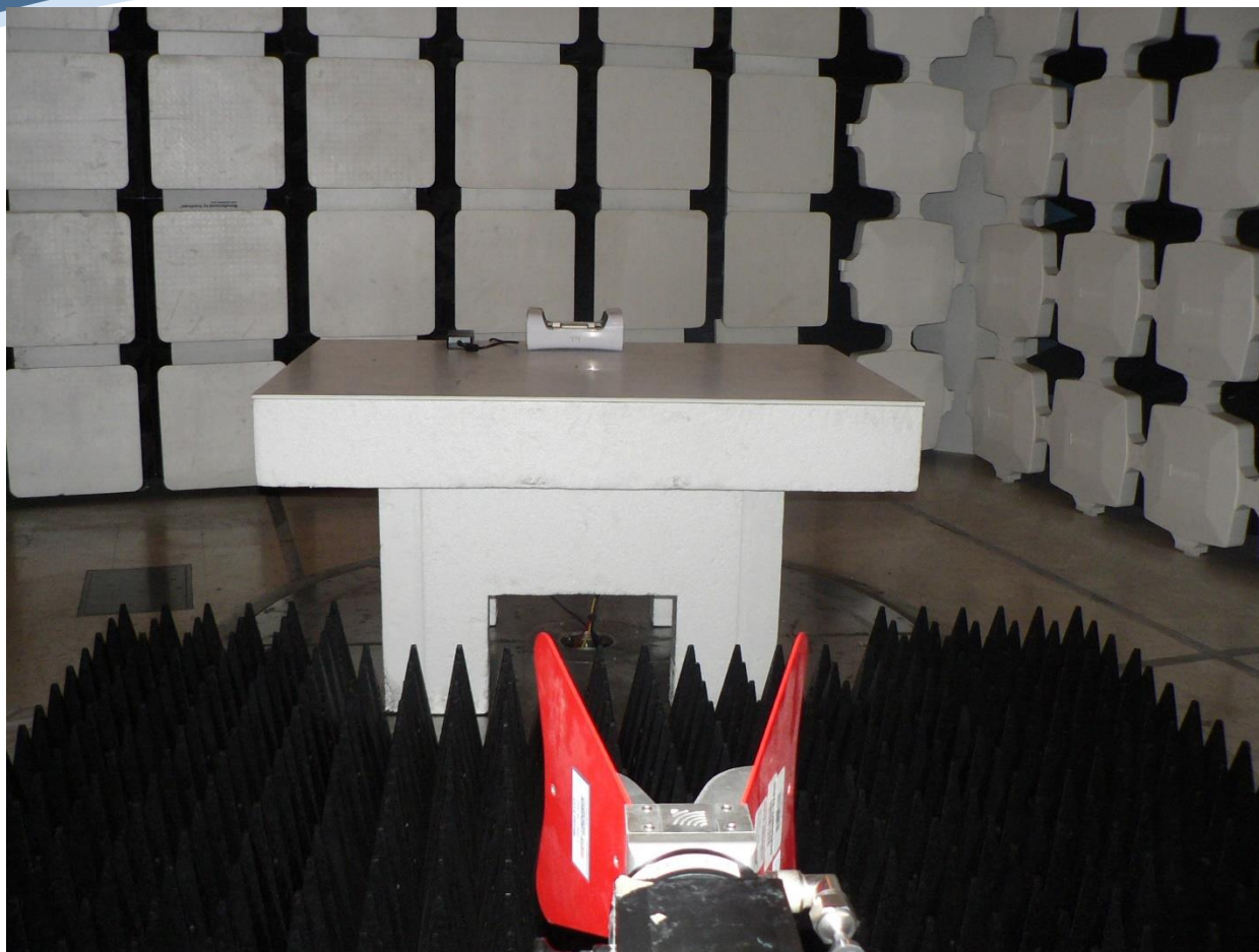
AIRI02 Radiated Emissions 1-18GHz
