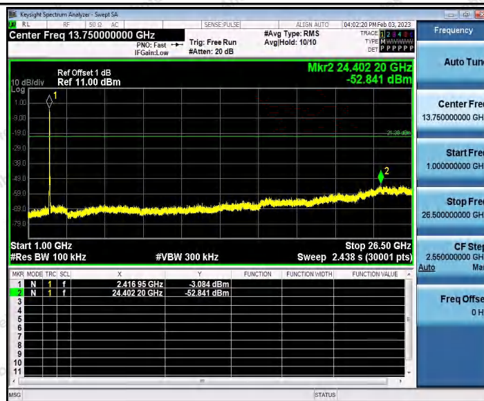
11AX40_Ant2_2422_0~Reference
