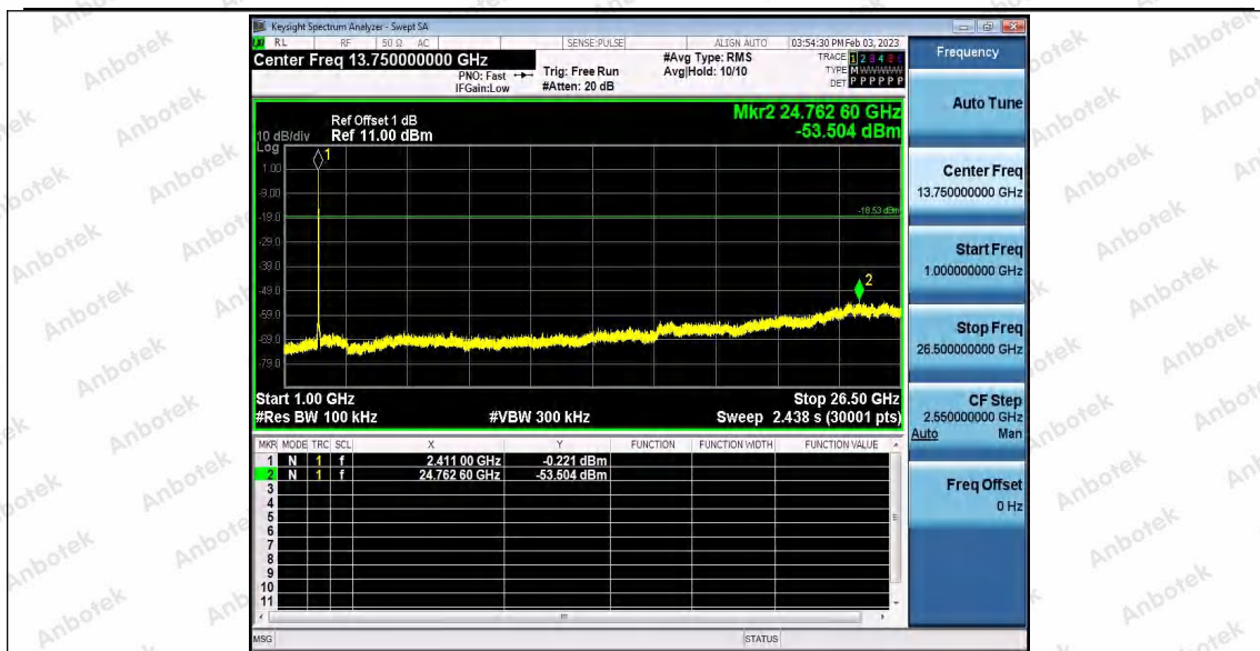
11AX20_Ant2_2412_0~Reference
