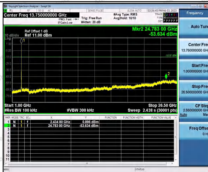
11AX20_Ant2_2437_0~Reference
