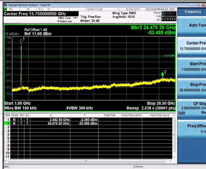
11N40_Ant1_2452_0~Reference
