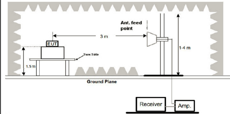
Above 1GHz
