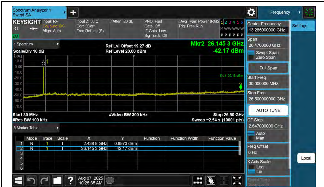
11AX20SISO-An2-2437-30~26500-PASS
