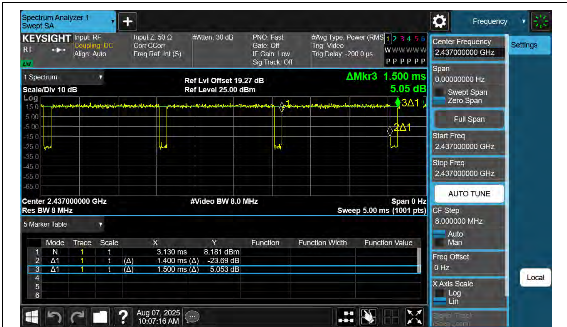
NTNV-11G-An2-2437
