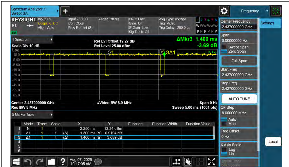
NTNV-11N20SISO-An2-2437
