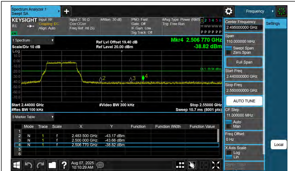
11G-An2-2462-PASS
