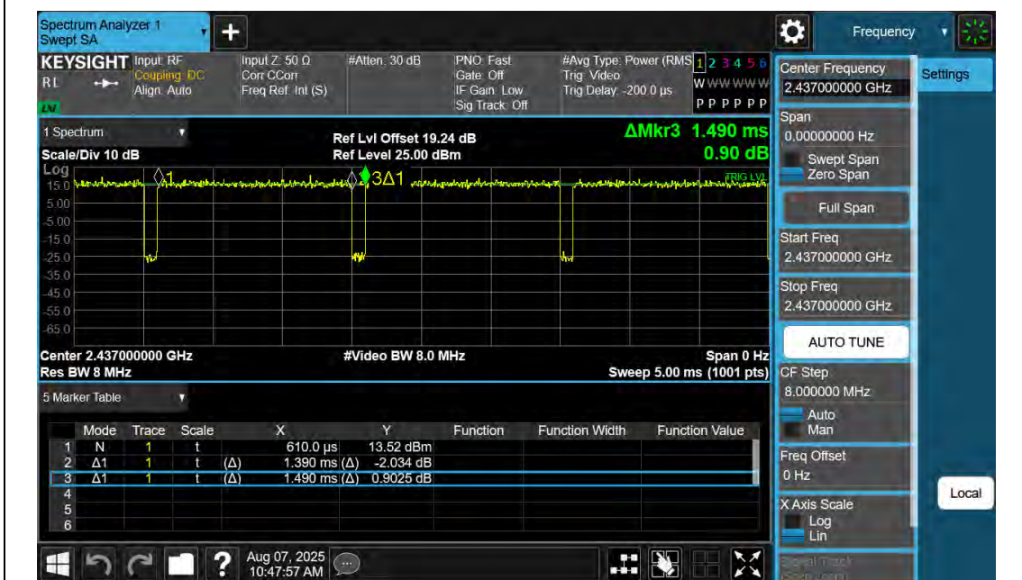
NTNV-11N20SISO-Ant1-2437
