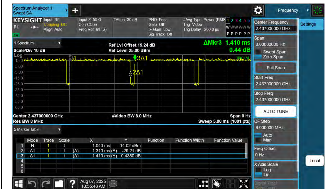
NTNV-11AX20SISO-Ant1-2437
