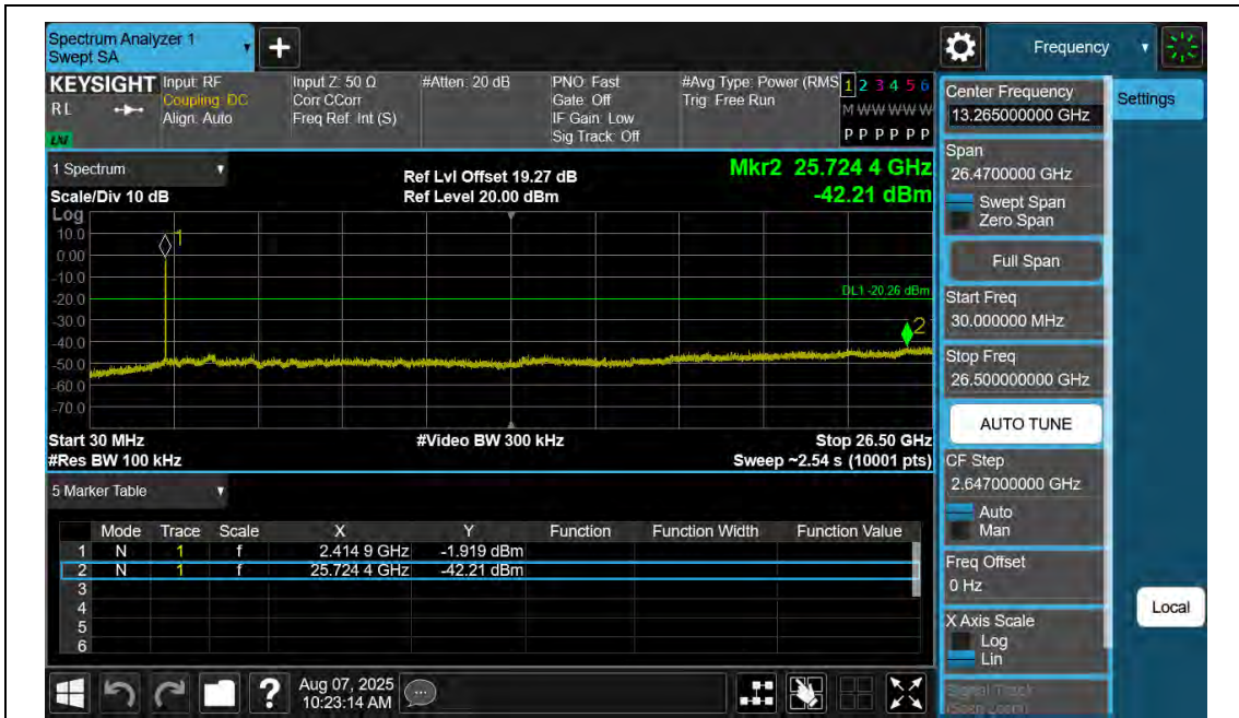
11AX20SISO-An2-2412-30~26500-PASS
