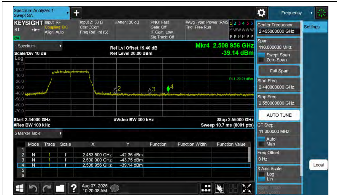
11N20SISO-An2-2462-PASS
