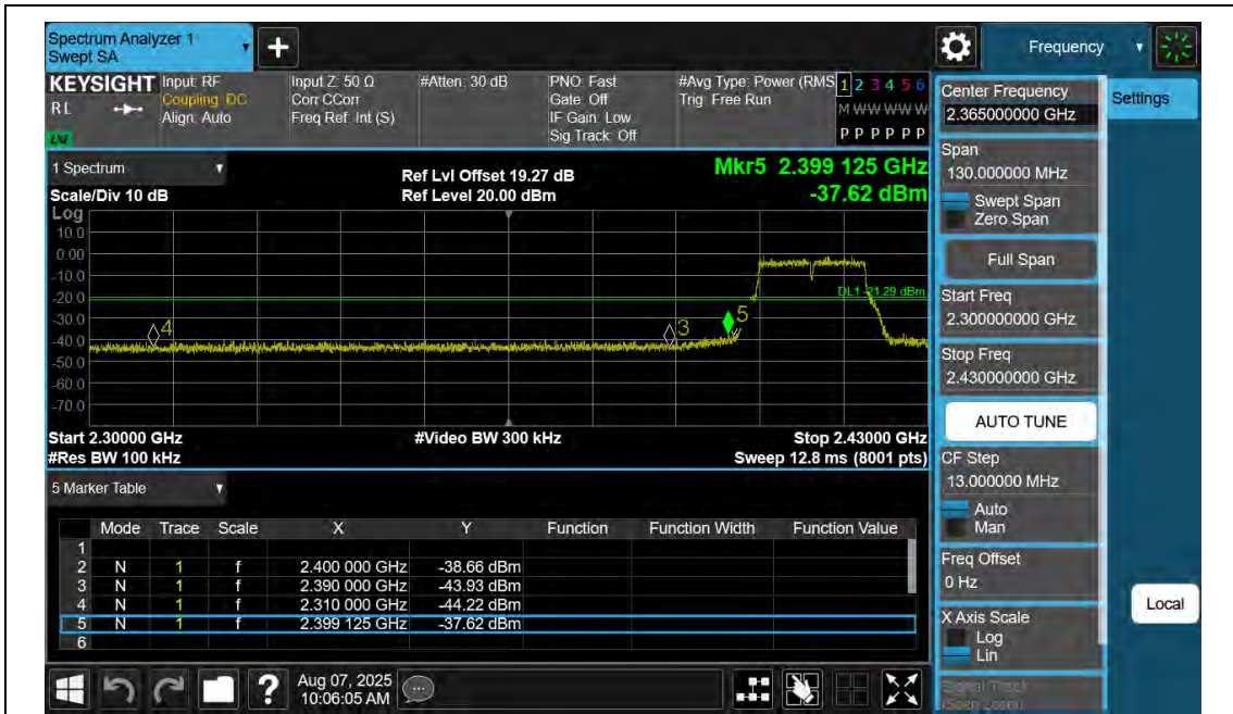
11G-An2-2412-PASS
