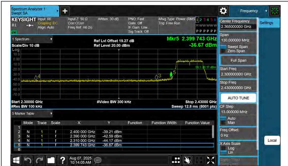
11N20SISO-An2-2412-PASS
