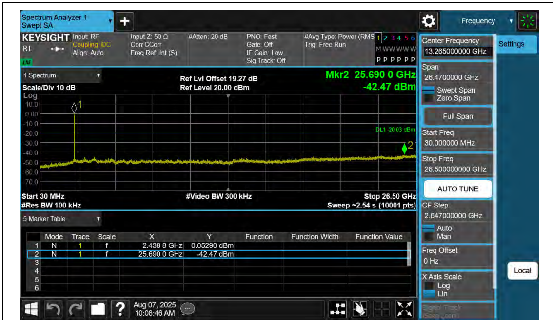
11G-An2-2437-30~26500-PASS
