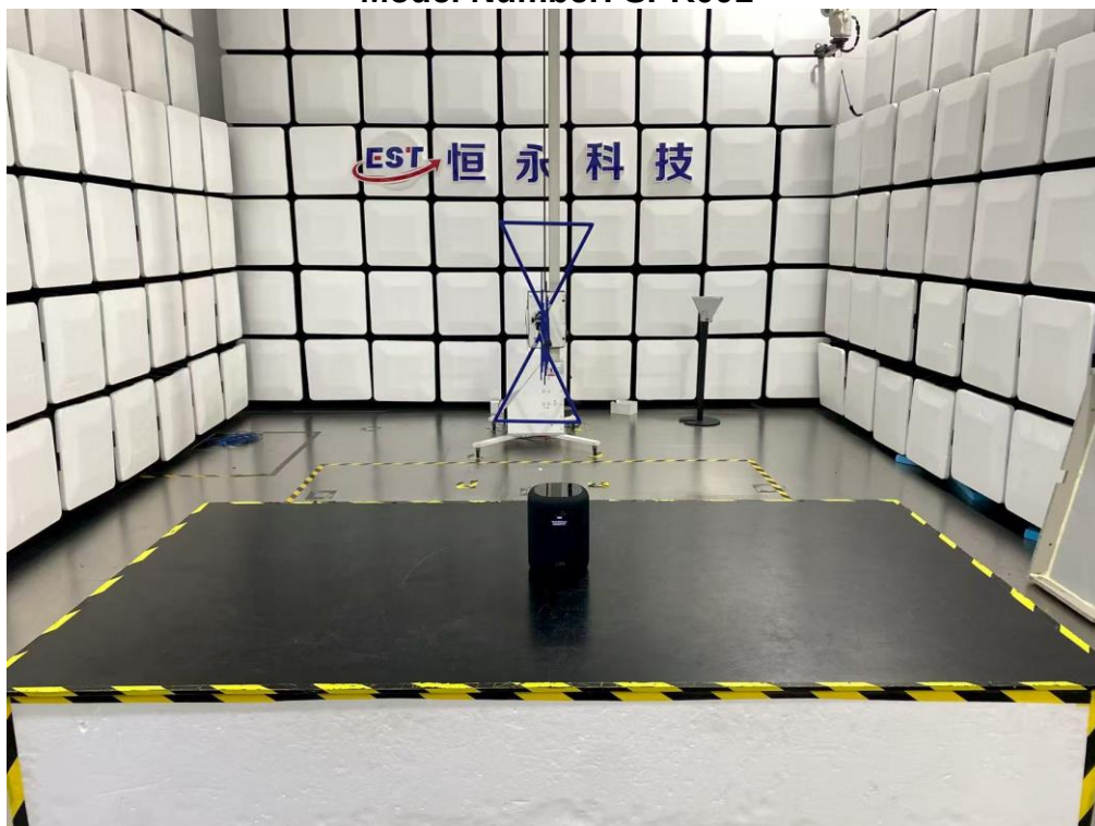
Radiated Test (Below 1GHz) Model Number: SPK001
