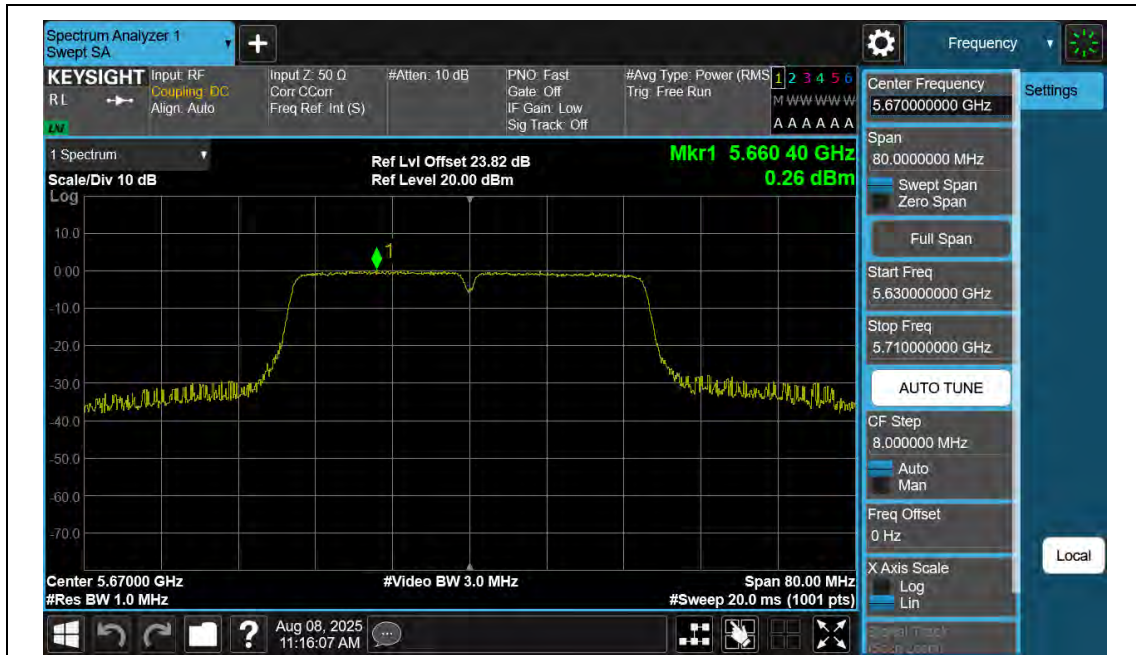
11AC40SISO-Ant2-5670-PASS
