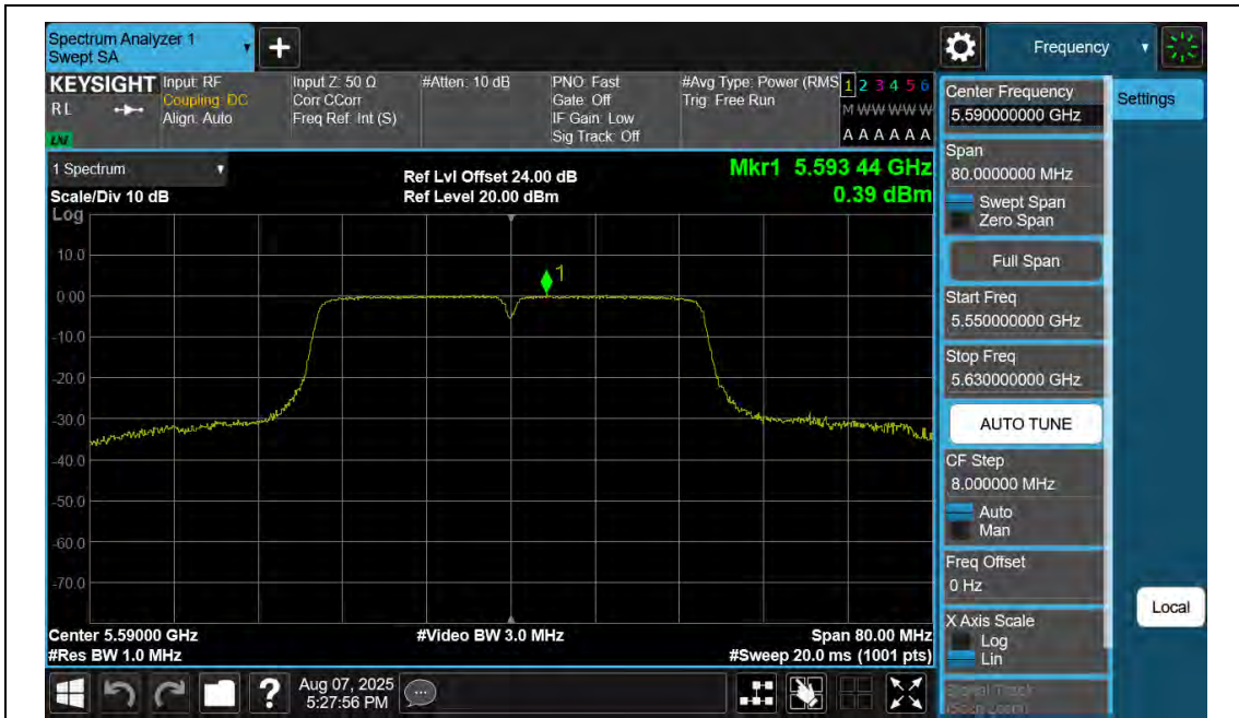
11N40SISO-Ant2-5590-PASS
