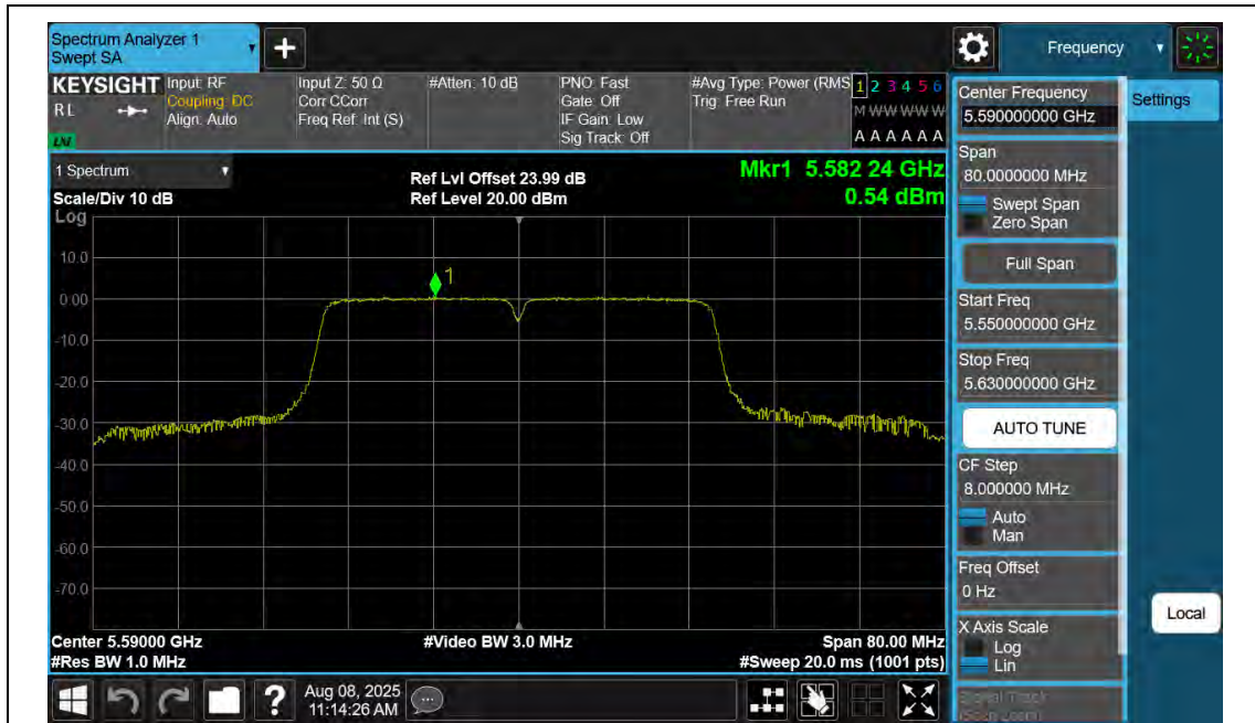
11AC40SISO-Ant2-5590-PASS
