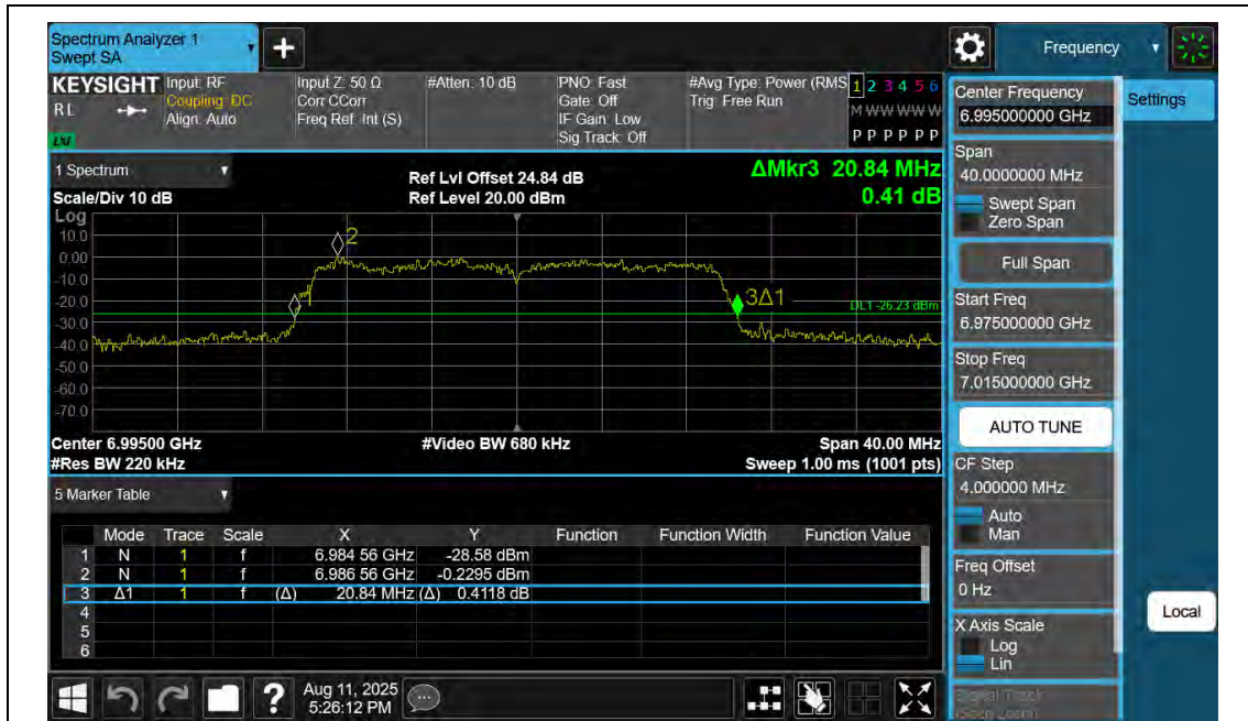
11AX20SISO-Ant2-6995
