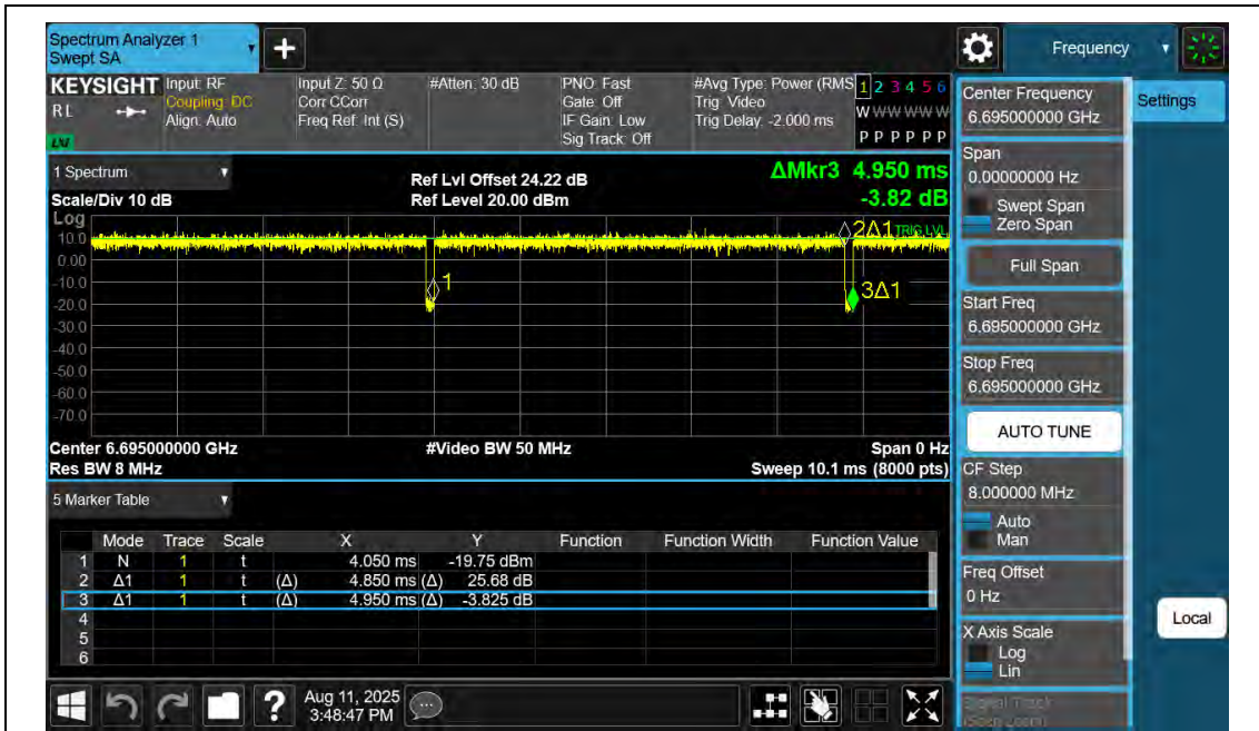
NTNV-11AX20SISO-Ant2-6695
