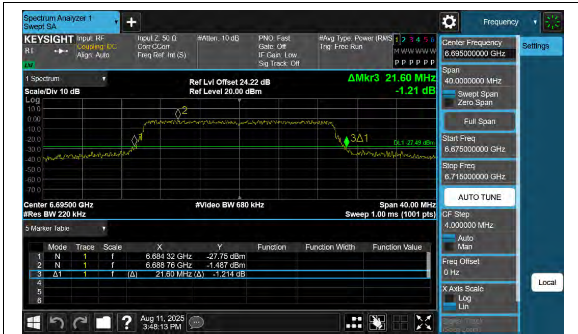
11AX20SISO-Ant2-6695
