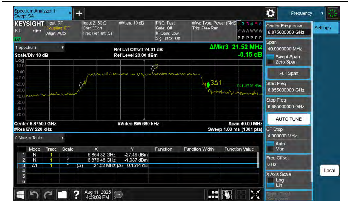
11AX20SISO-Ant2-6875
