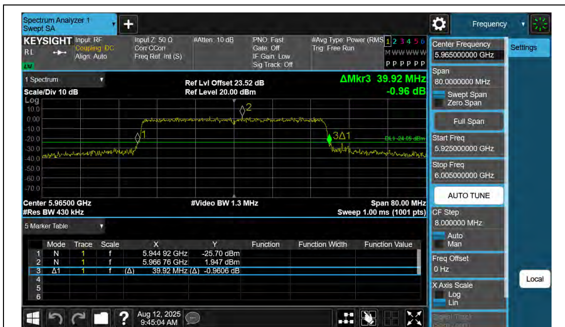
11AX40SISO-Ant2-5965
