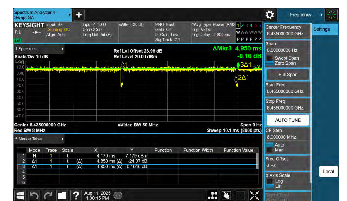
NTNV-11AX20SISO-Ant2-6435
