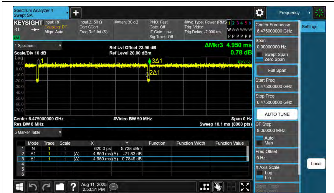
NTNV-11AX20SISO-Ant2-6475
