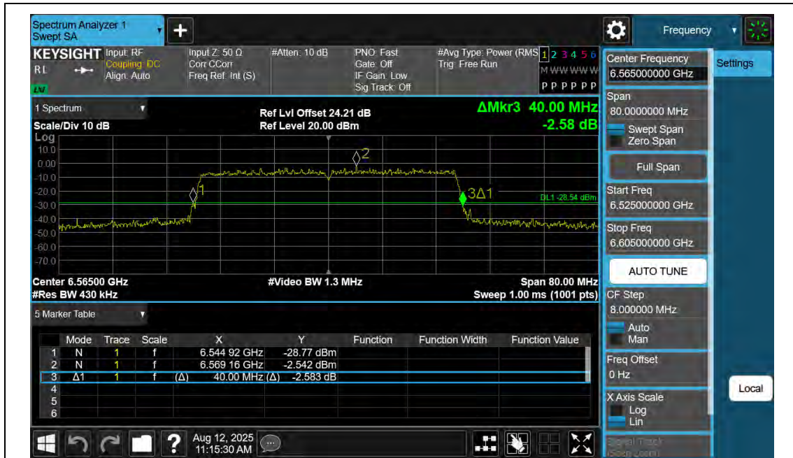
11AX40SISO-Ant2-6565
