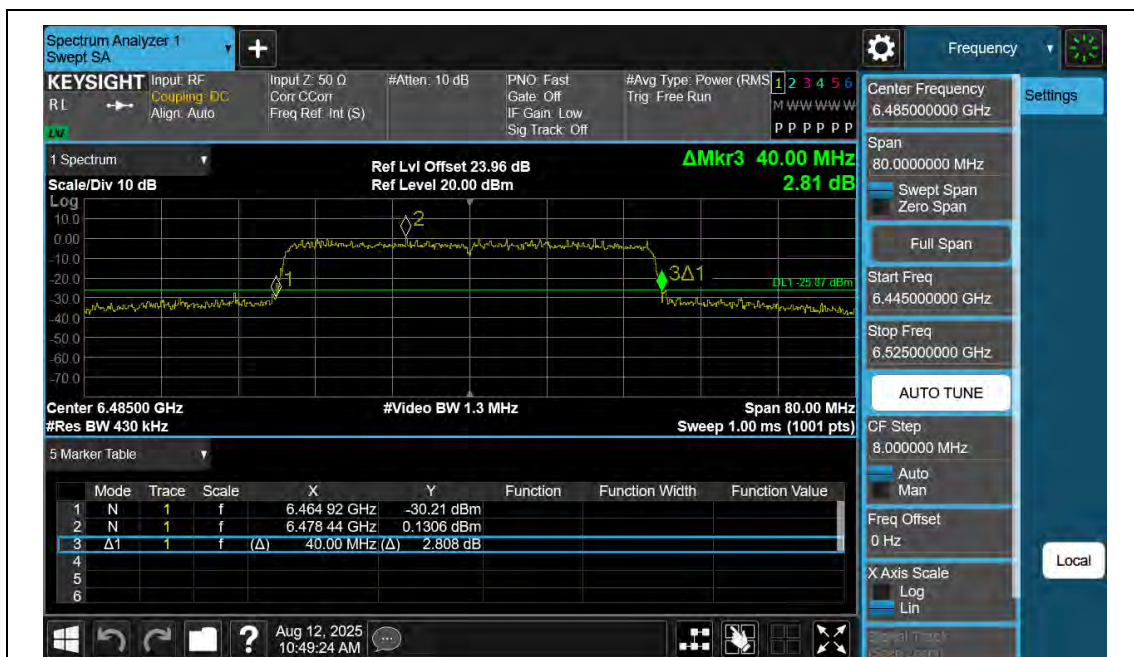
11AX40SISO-Ant2-6485
