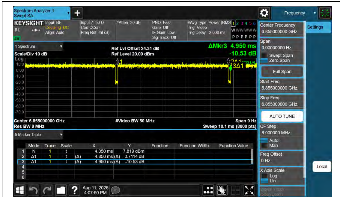
NTNV-11AX20SISO-Ant2-6855
