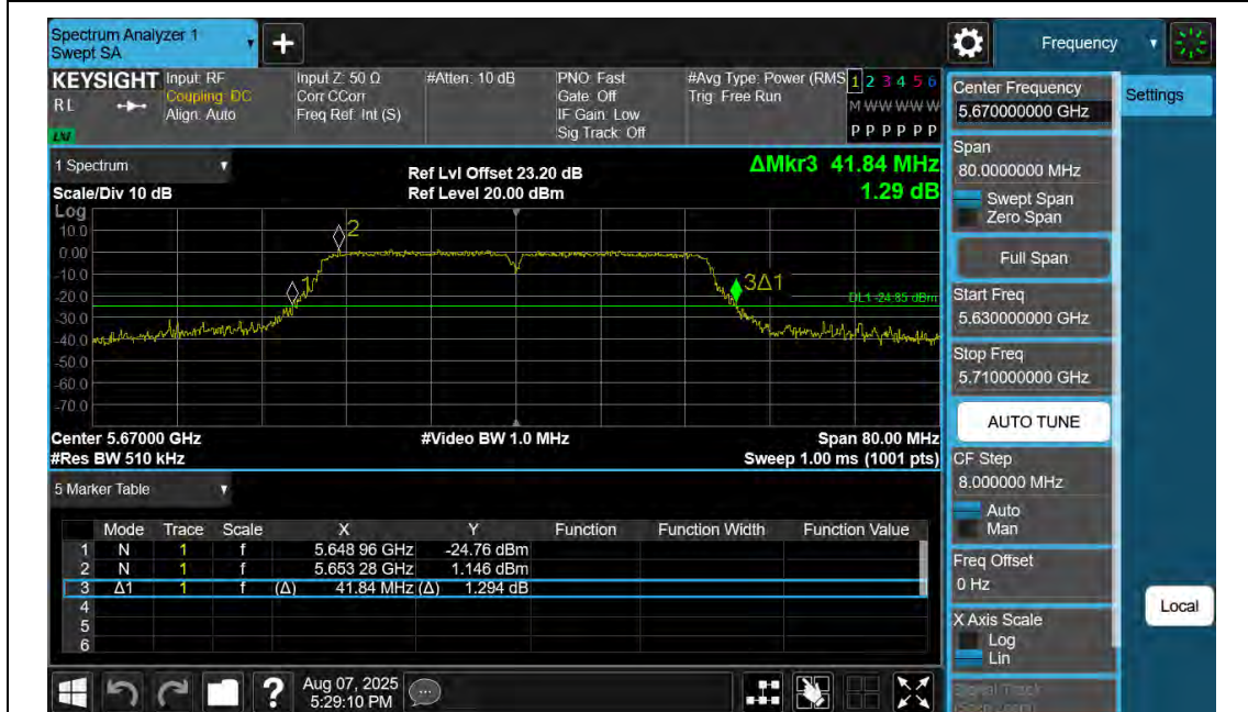
11N40SISO-Ant2-5670
