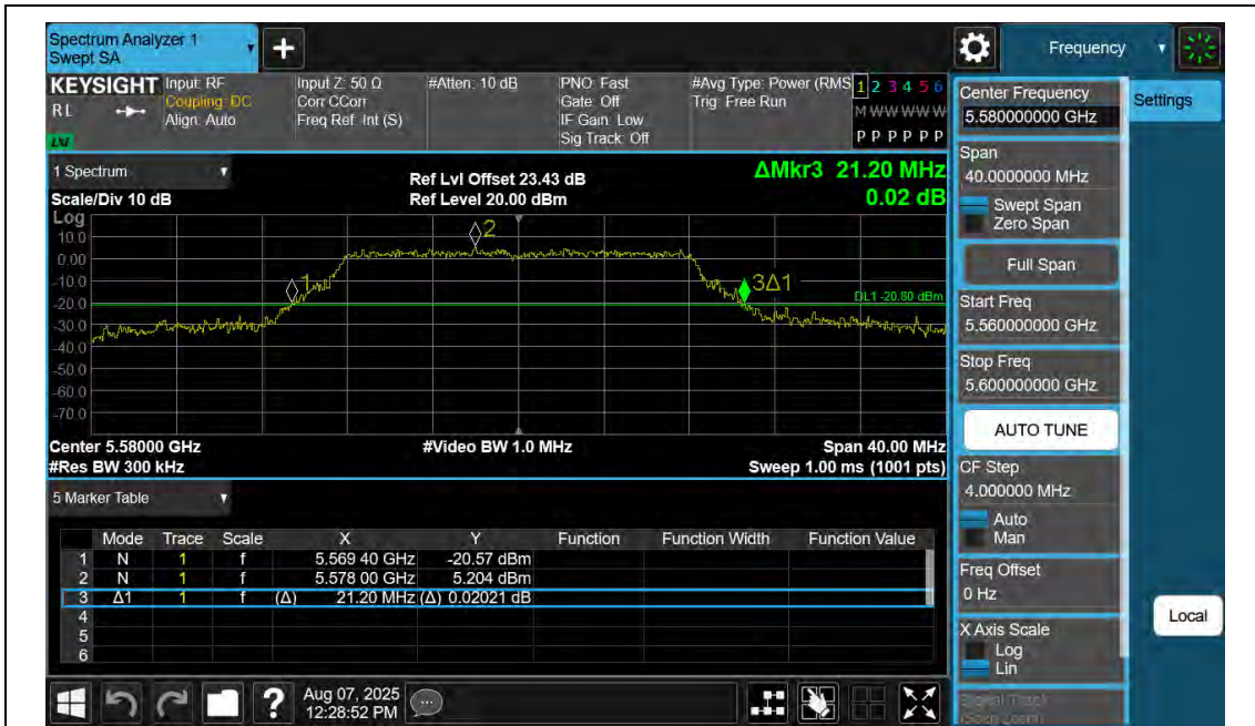
11A-Ant2-5580
