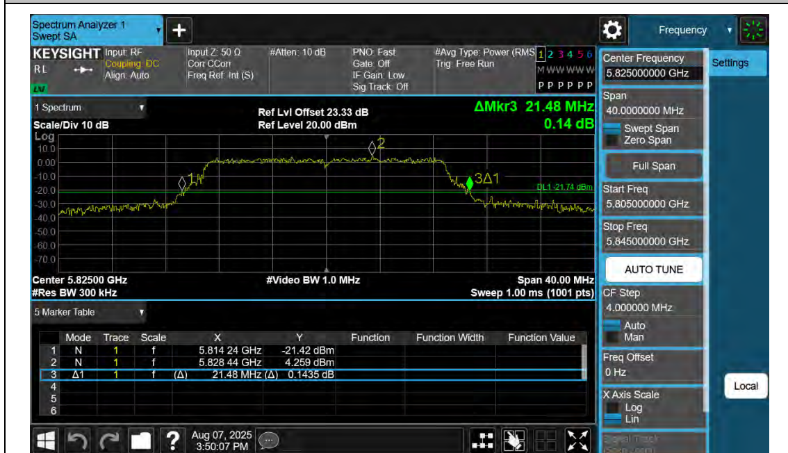
11N20SISO-Ant2-5825
