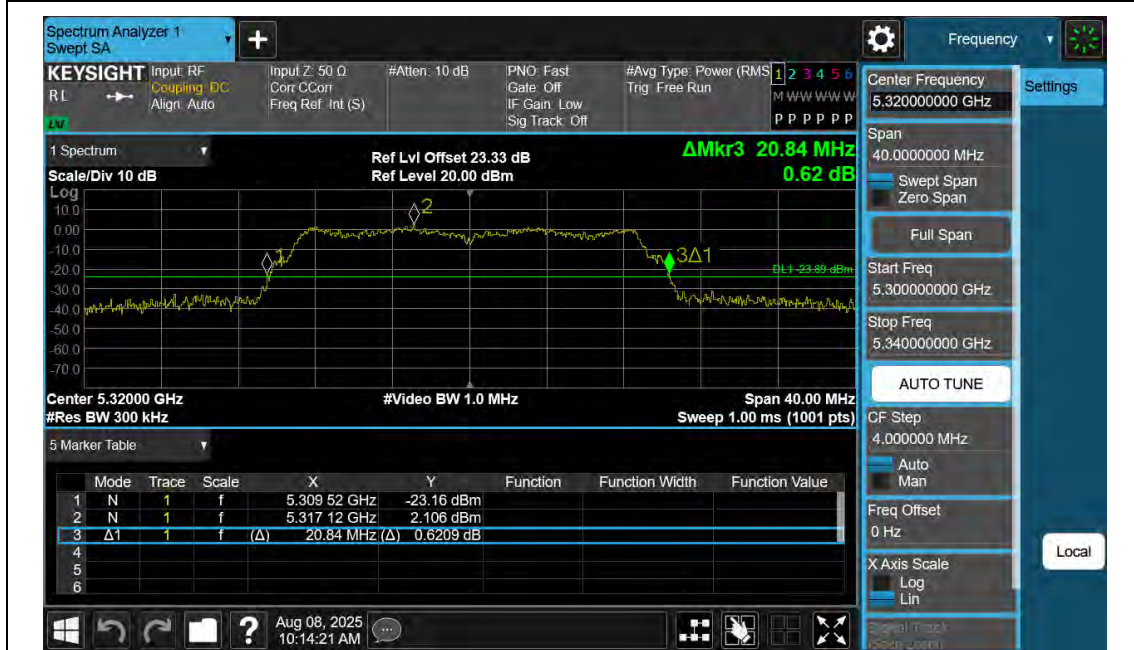
11AC20SISO-Ant2-5320
