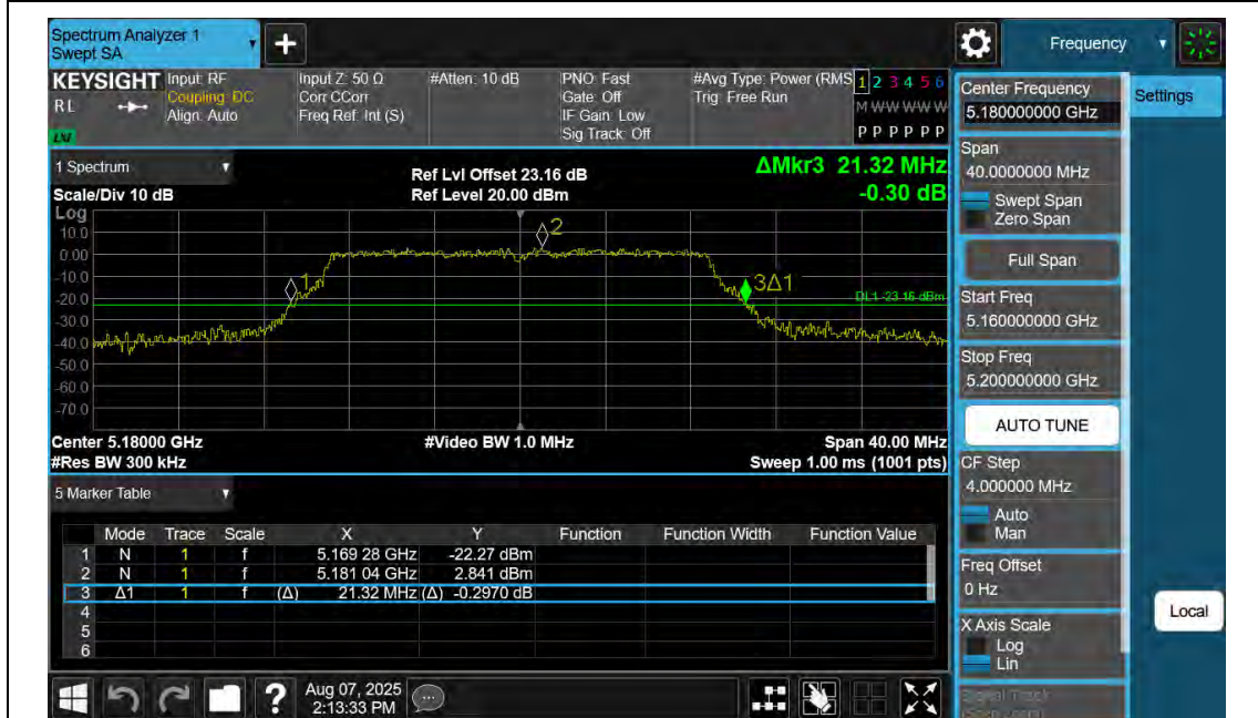
11N20SISO-Ant2-5180
