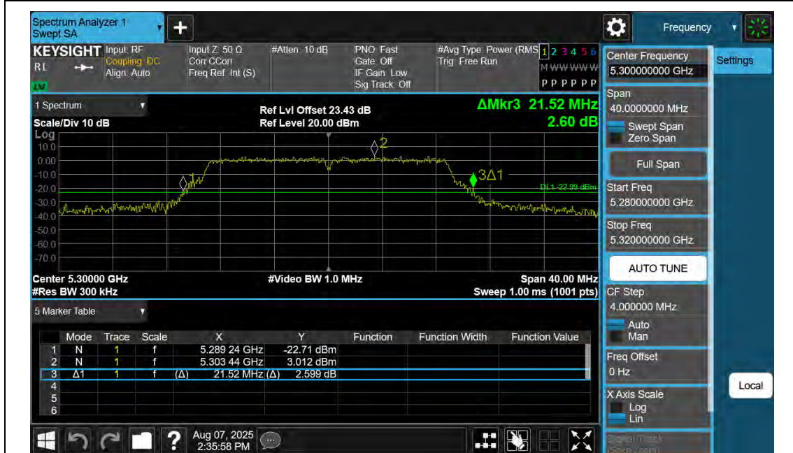
11N20SISO-Ant2-5300
