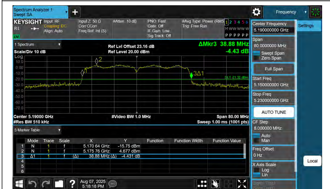
11N40SISO-Ant2-5190
