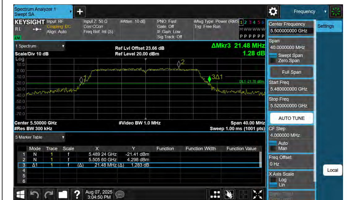
11N20SISO-Ant2-5500
