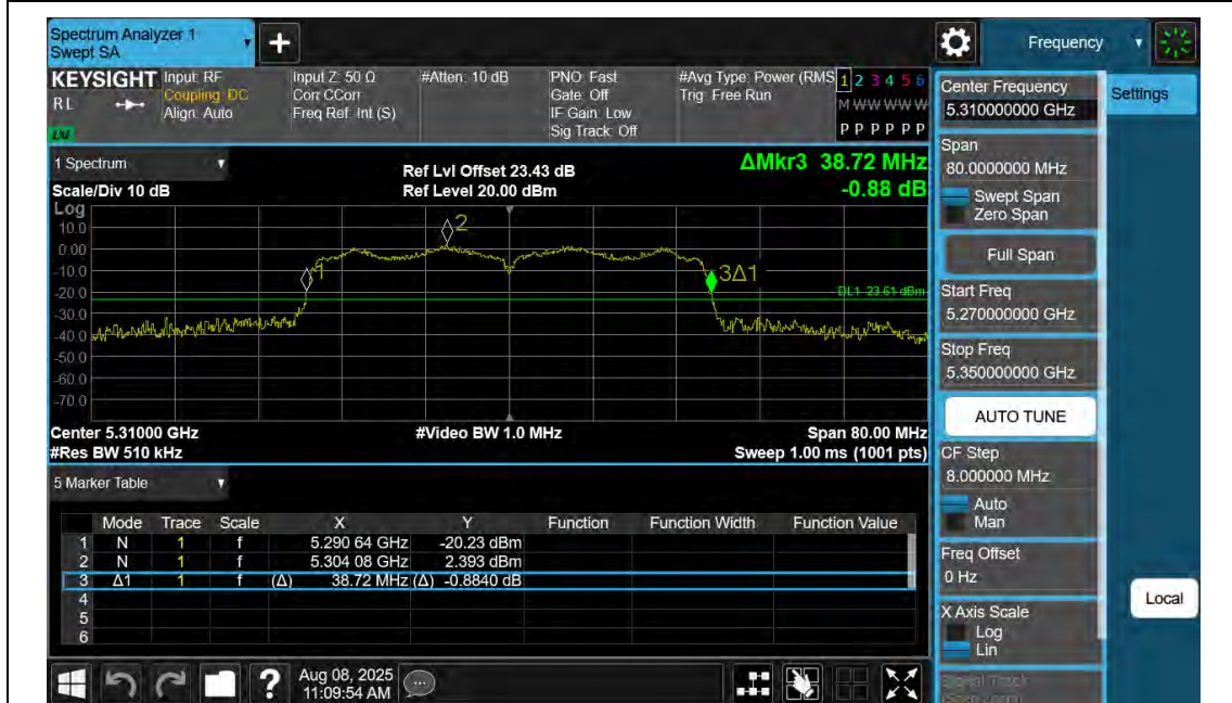
11AC40SISO-Ant2-5310
