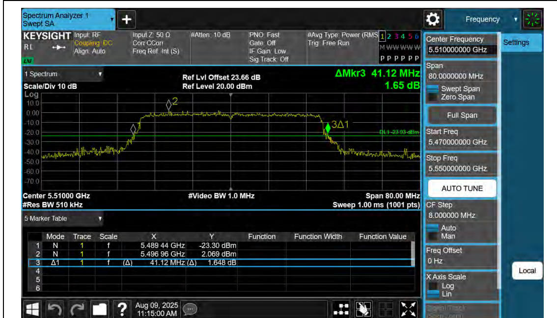
11AX40SISO-Ant2-5510
