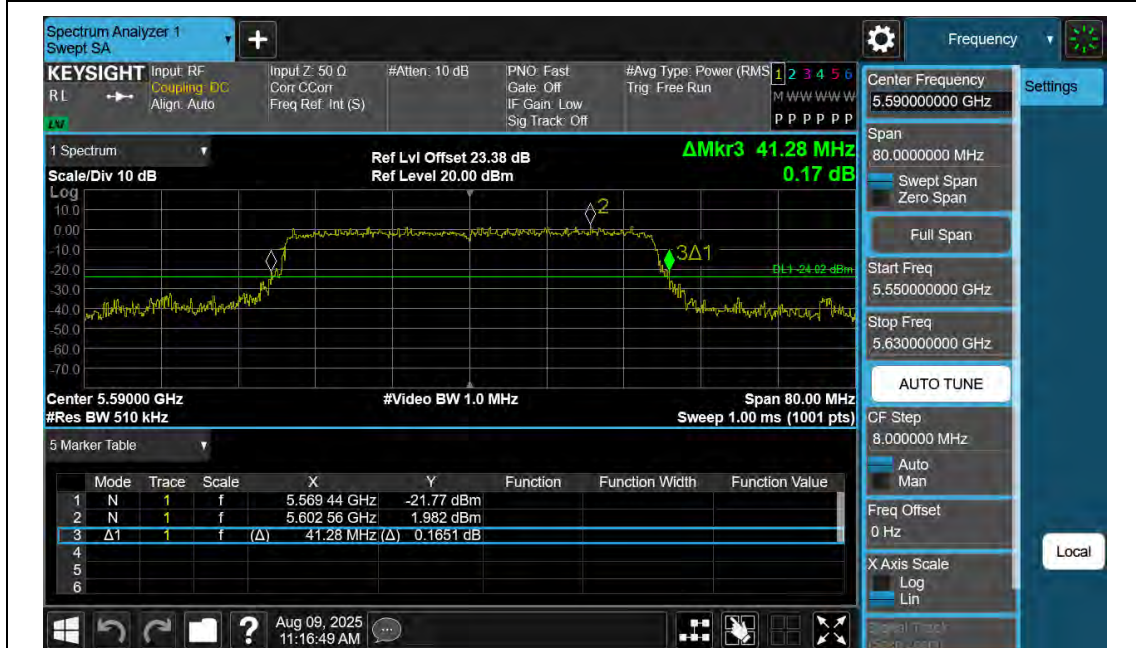
11AX40SISO-Ant2-5590
