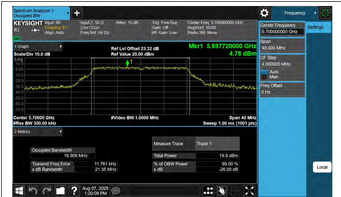
11A-Ant2-5700
