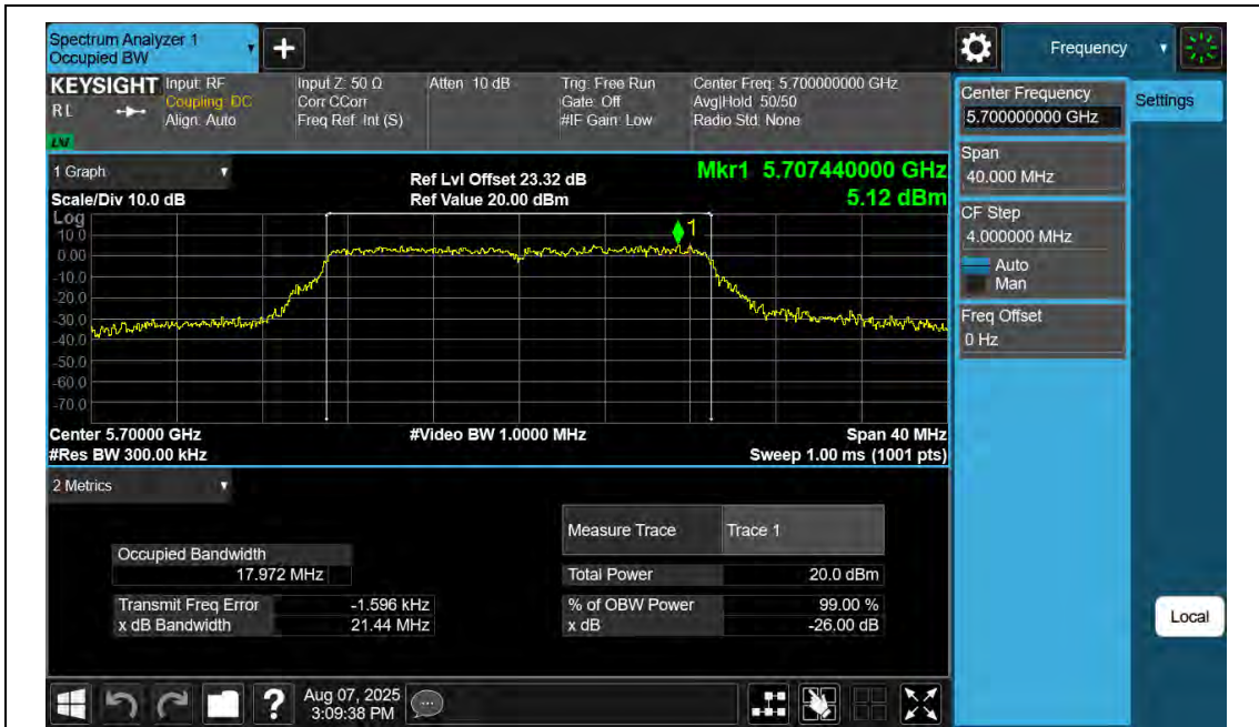
11N20SISO-Ant2-5700
