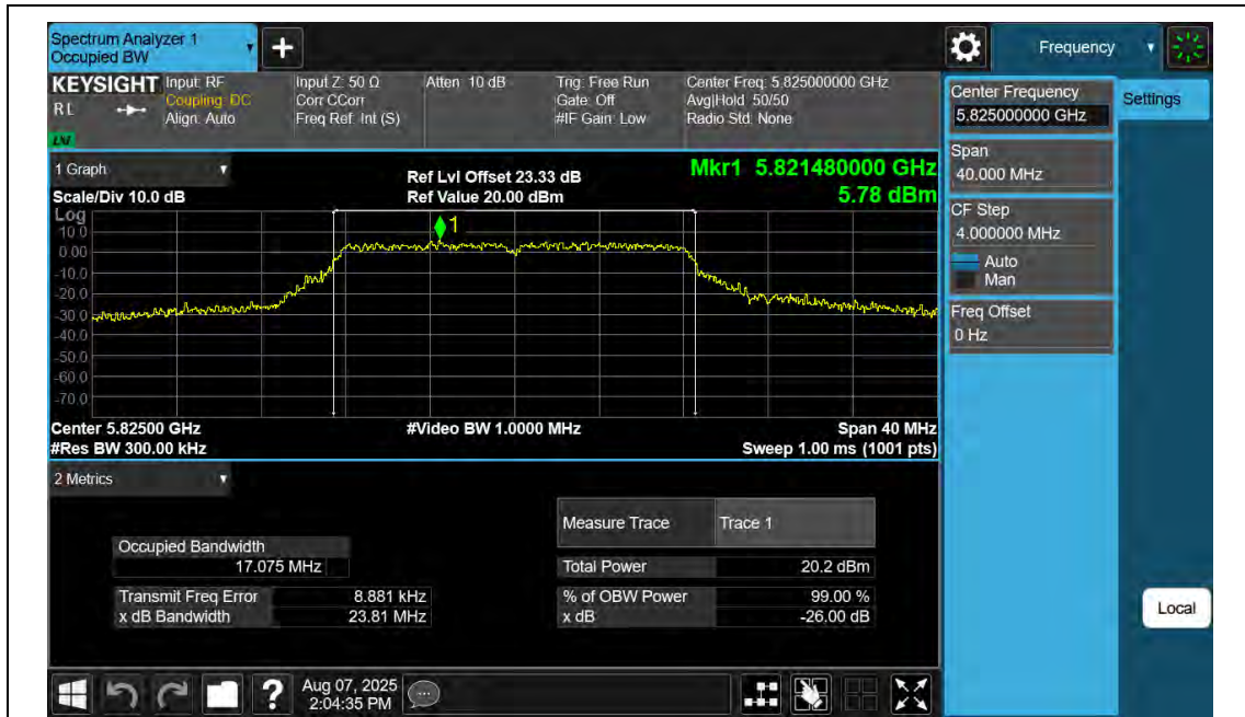
11A-Ant2-5825
