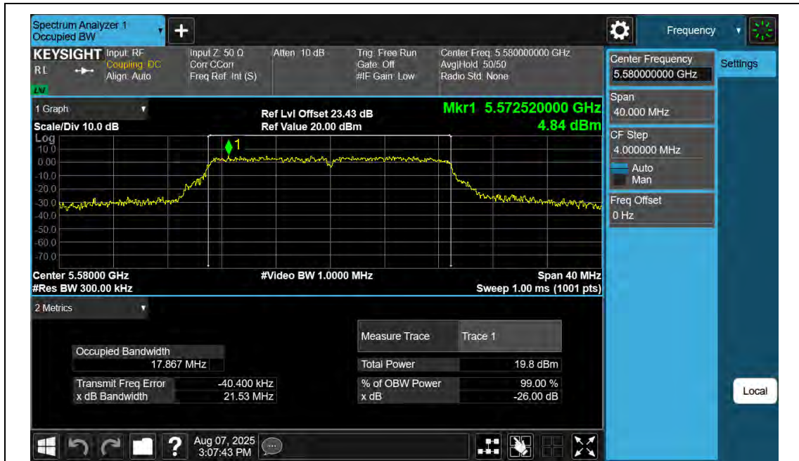
11N20SISO-Ant2-5580
