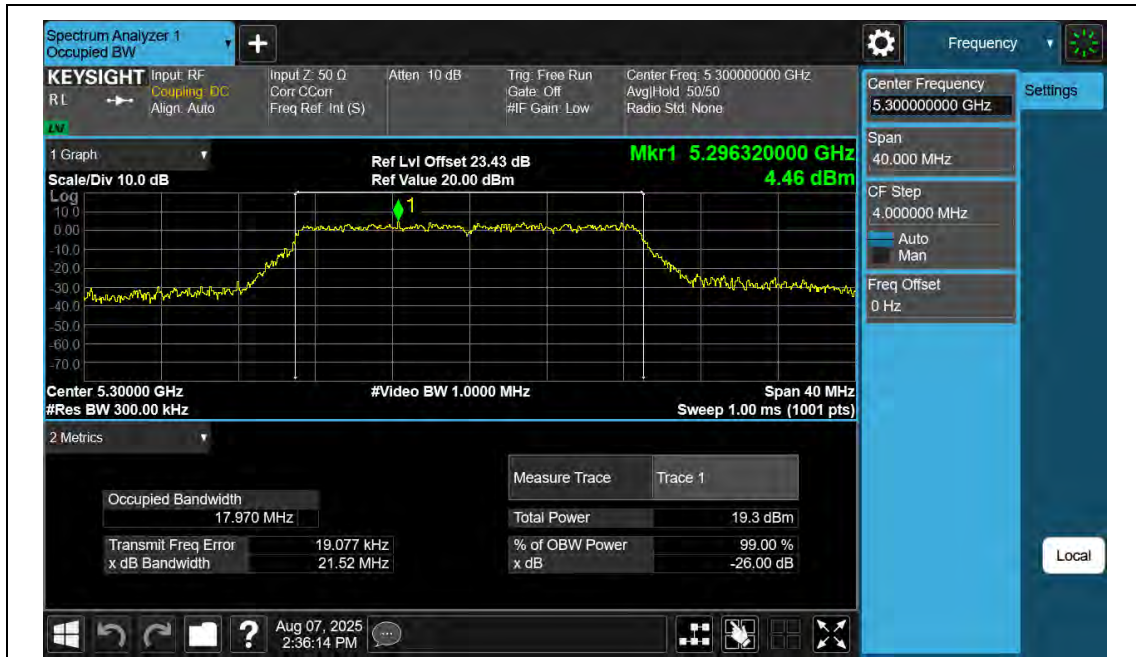
11N20SISO-Ant2-5300
