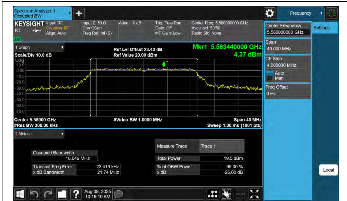
11AC20SISO-Ant2-5580
