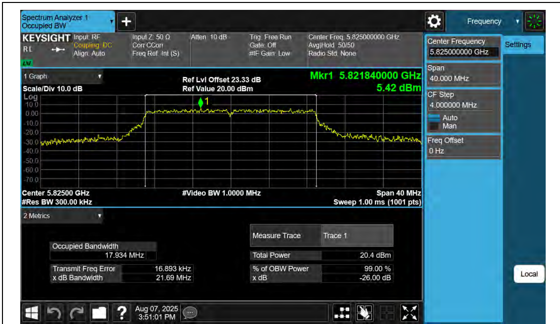
11N20SISO-Ant2-5825
