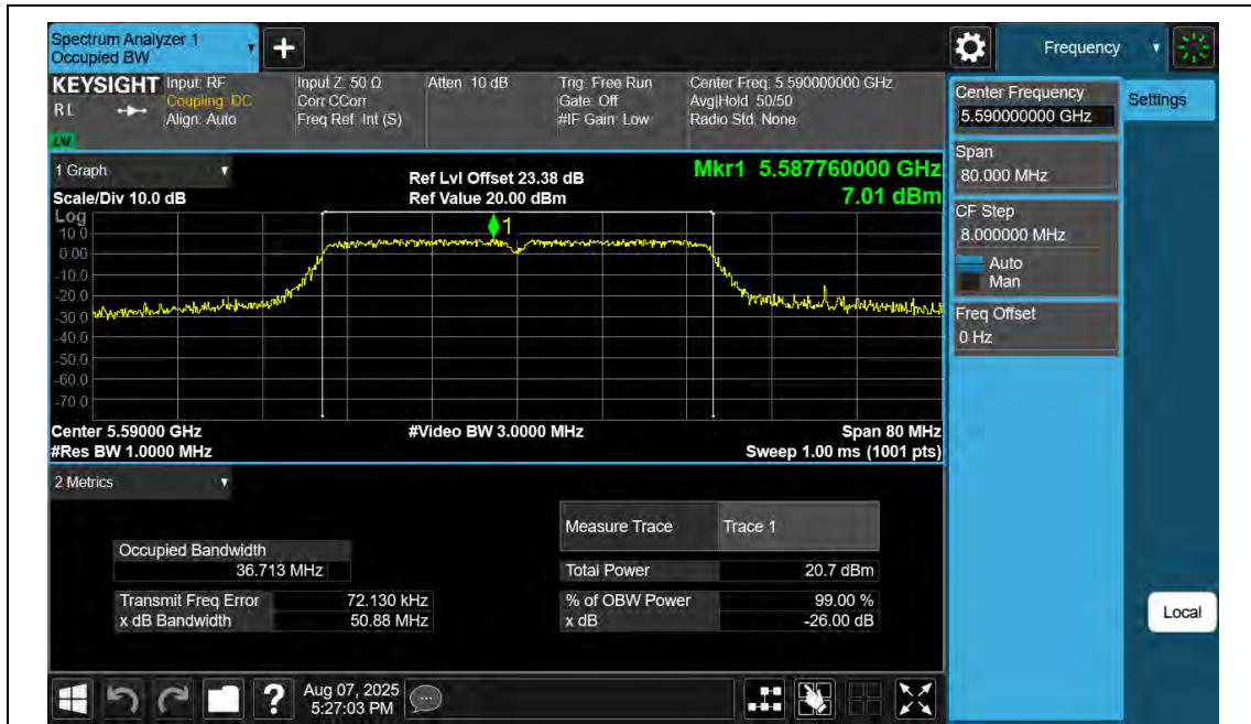
11N40SISO-Ant2-5590
