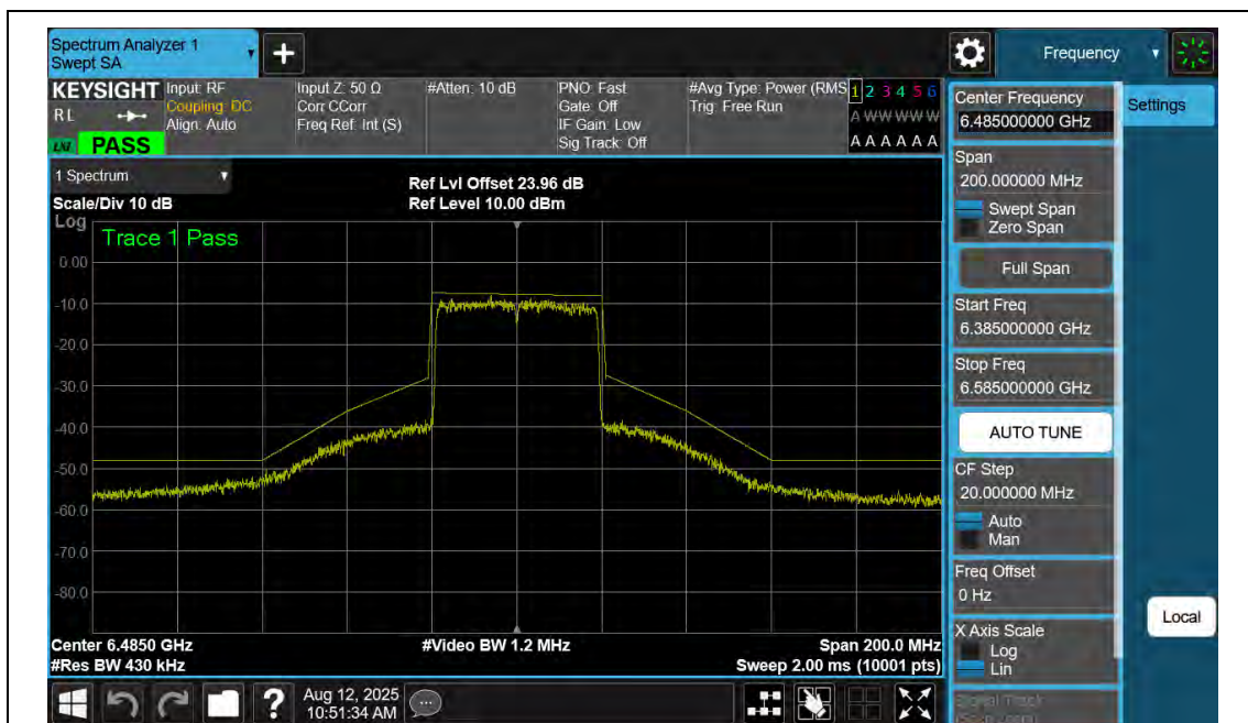
NTNV-11AX40SISO-Ant2-6485-PASS
