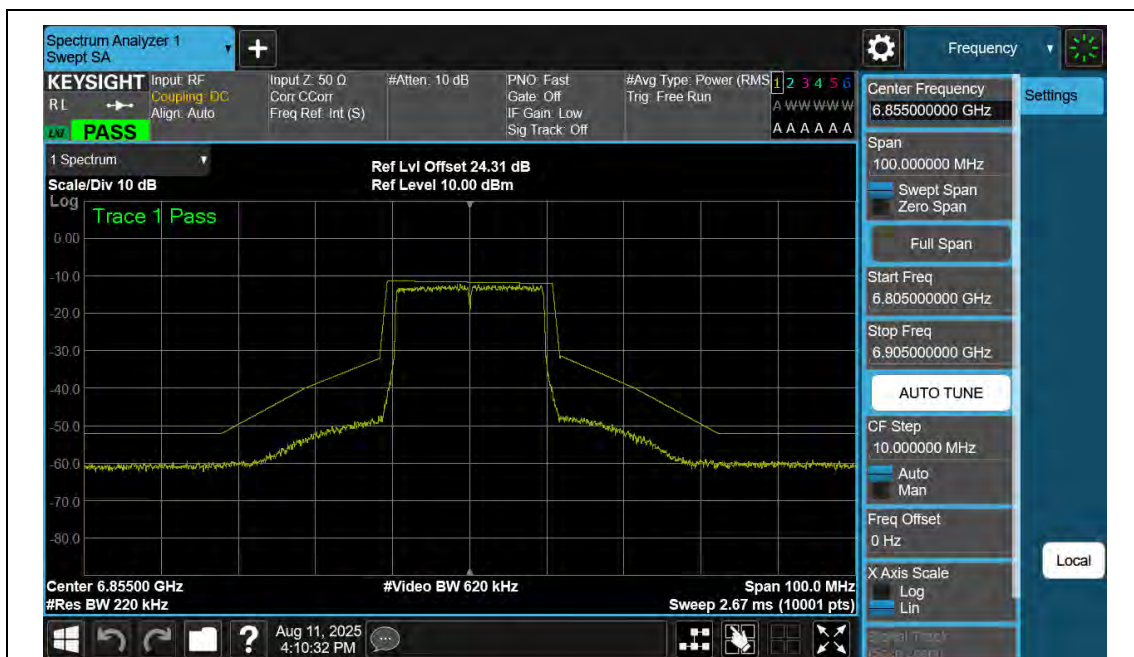
NTNV-11AX20SISO-Ant2-6855-PASS
