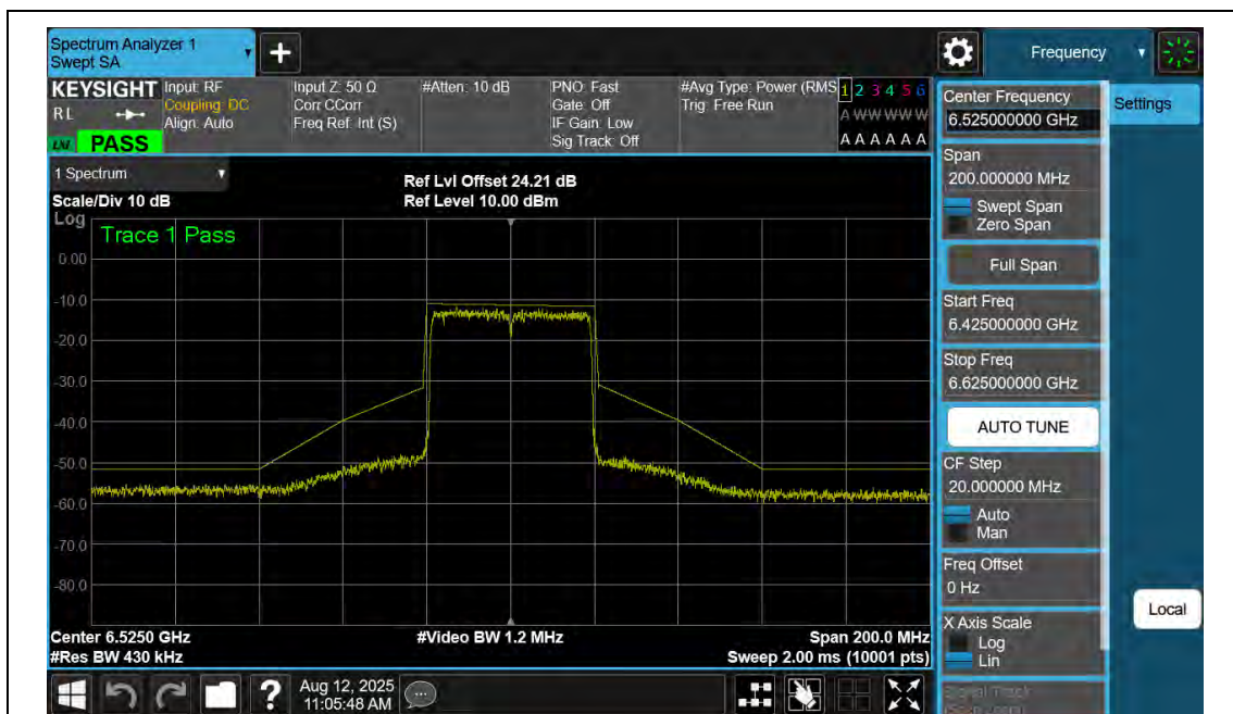
NTNV-11AX40SISO-Ant2-6525-PASS
