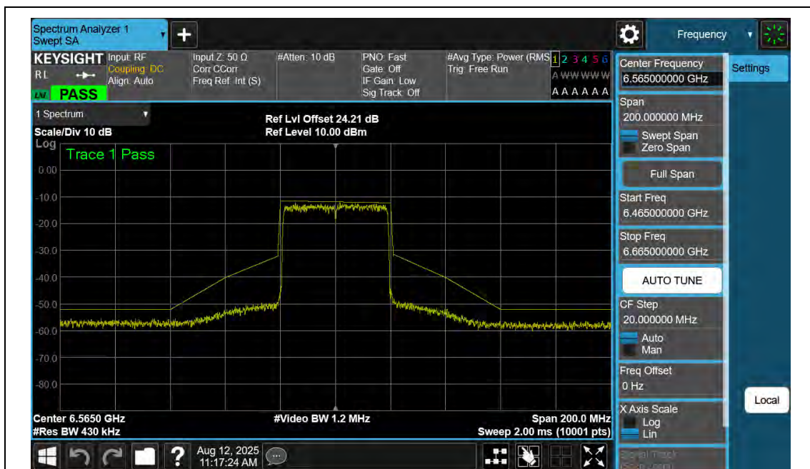
NTNV-11AX40SISO-Ant2-6565-PASS
