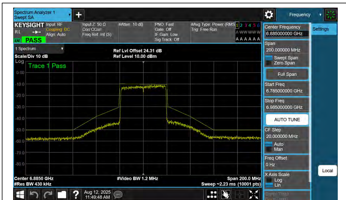
NTNV-11AX40SISO-Ant2-6885-PASS
