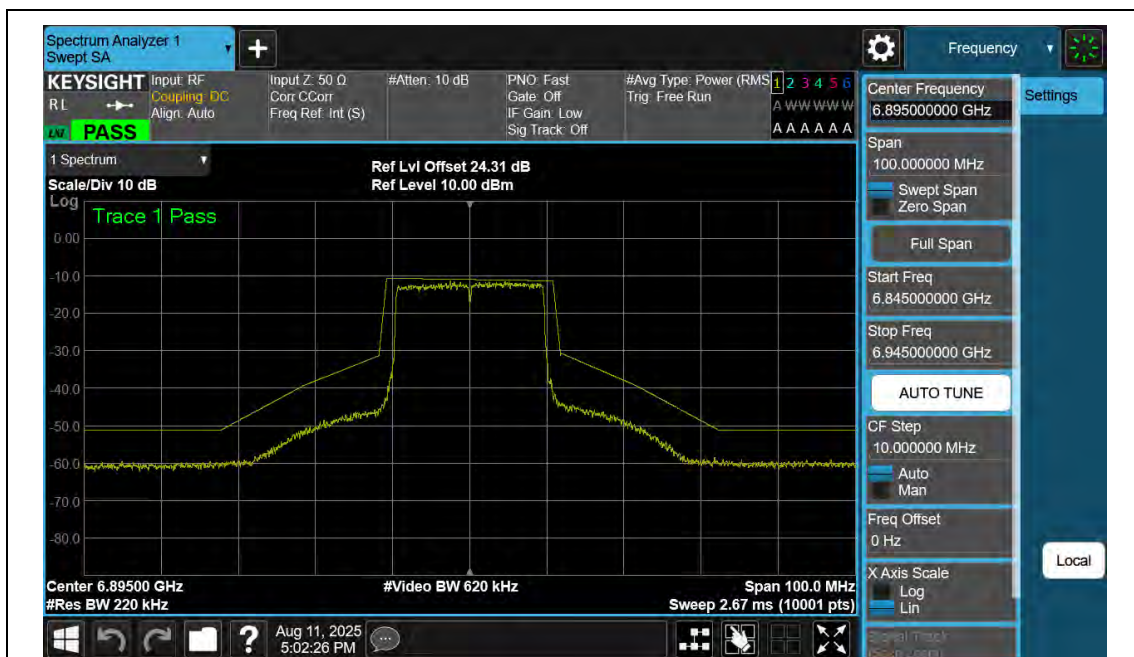
NTNV-11AX20SISO-Ant2-6895-PASS
