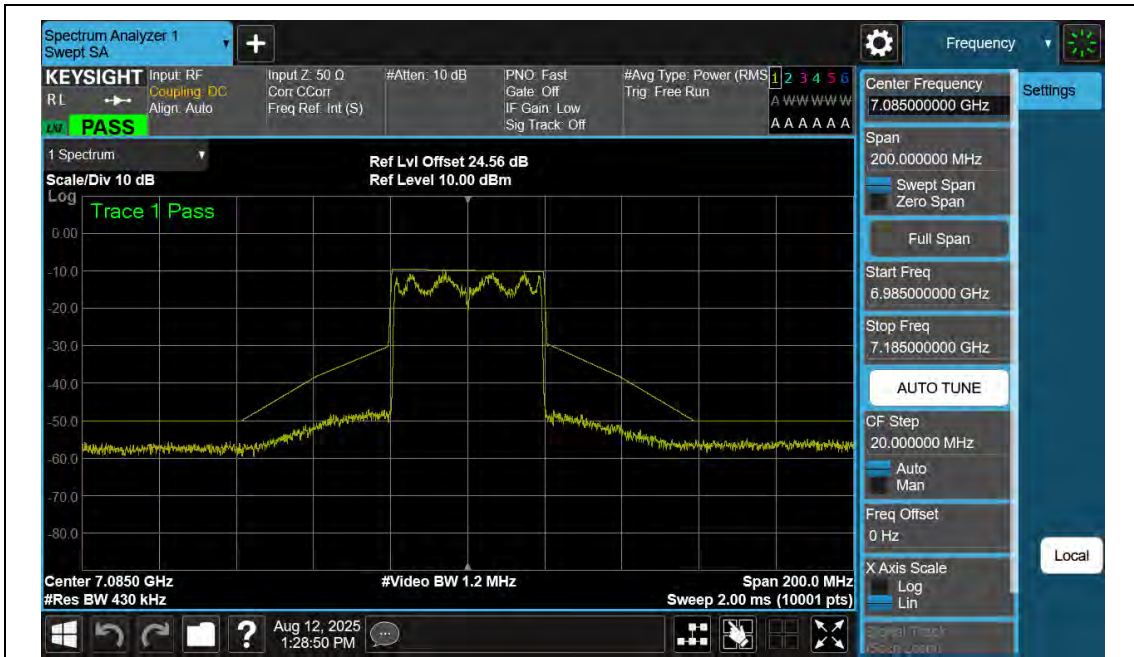
NTNV-11AX40SISO-Ant2-7085-PASS
