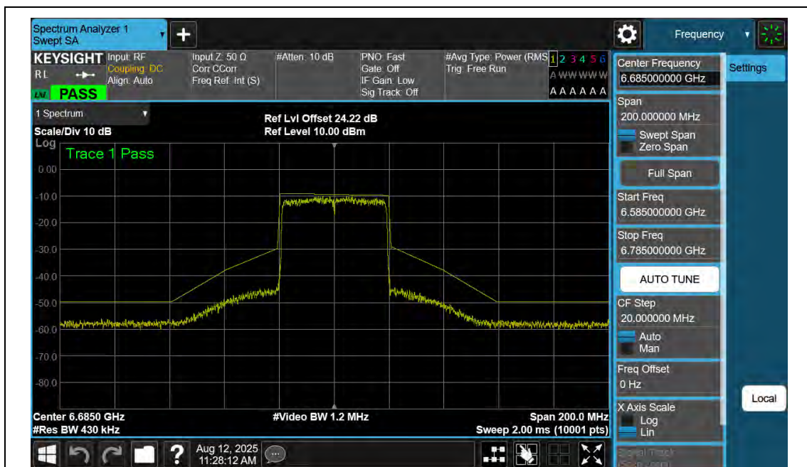
NTNV-11AX40SISO-Ant2-6685-PASS
