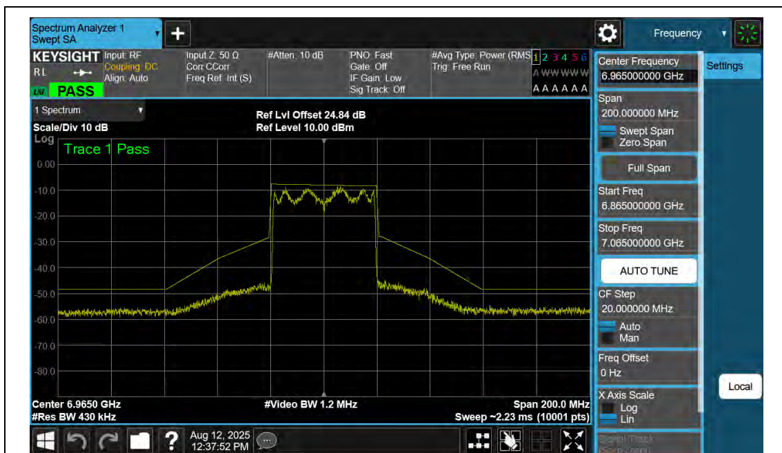
NTNV-11AX40SISO-Ant2-6965-PASS
