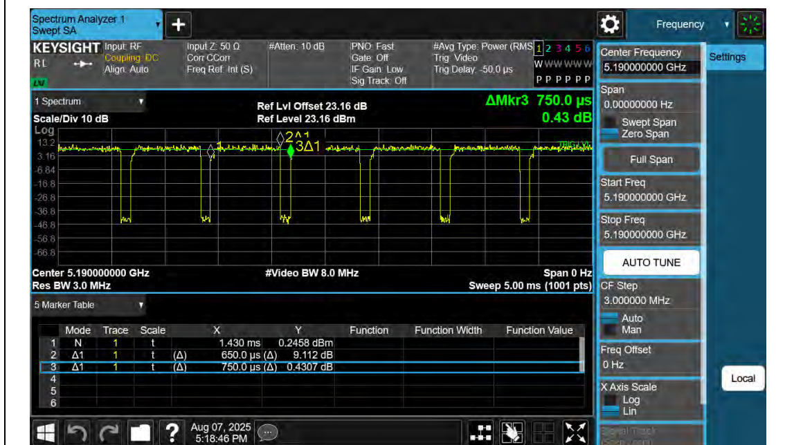
NTNV-11N40SISO-Ant2-5190
