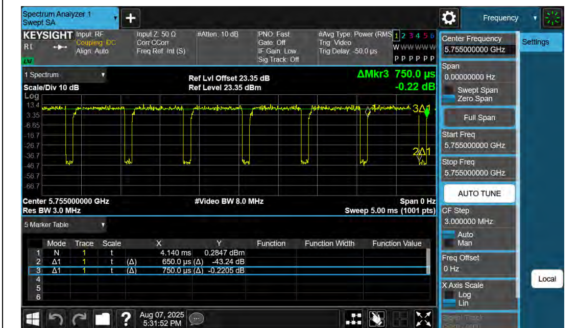
NTNV-11N40SISO-Ant2-5755
