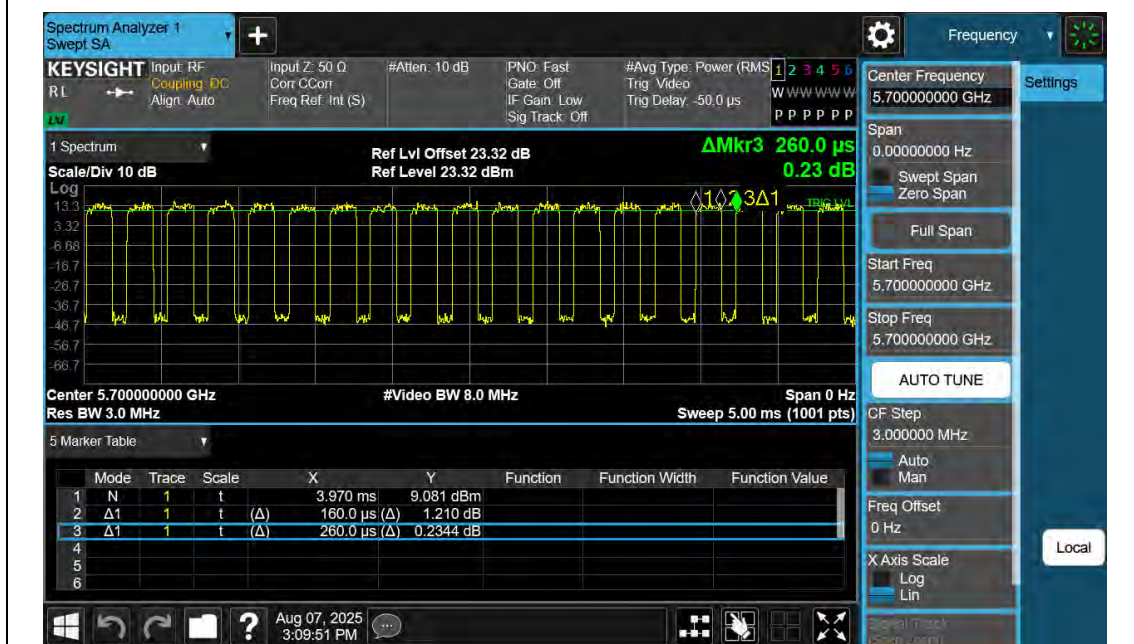
NTNV-11N20SISO-Ant2-5700
