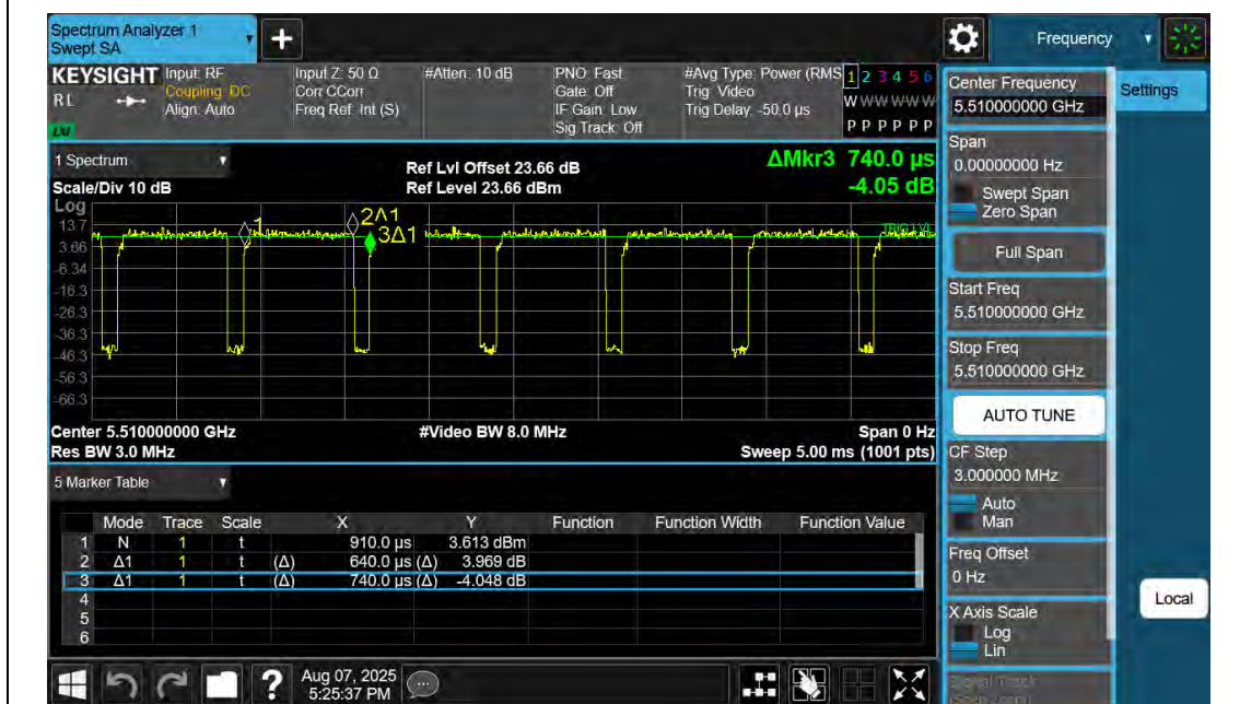
NTNV-11N40SISO-Ant2-5510
