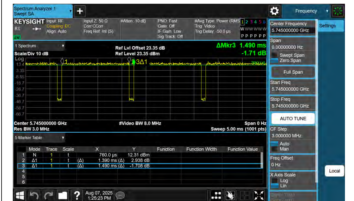
NTNV-11A-Ant2-5745
