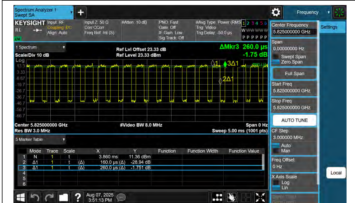
NTNV-11N20SISO-Ant2-5825
