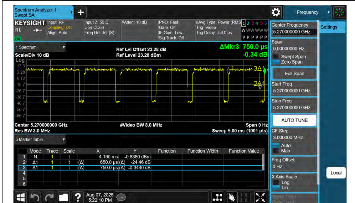
NTNV-11N40SISO-Ant2-5270
