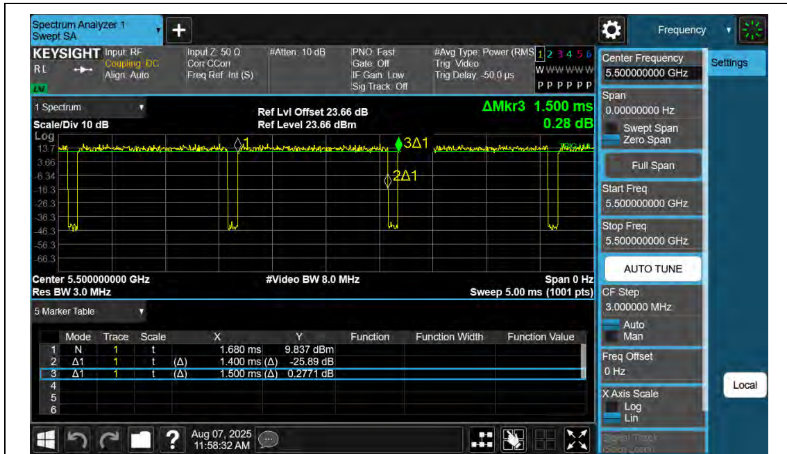
NTNV-11A-Ant2-5500
