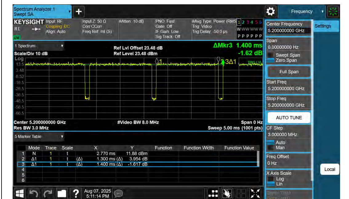
NTNV-11N20SISO-Ant2-5200
