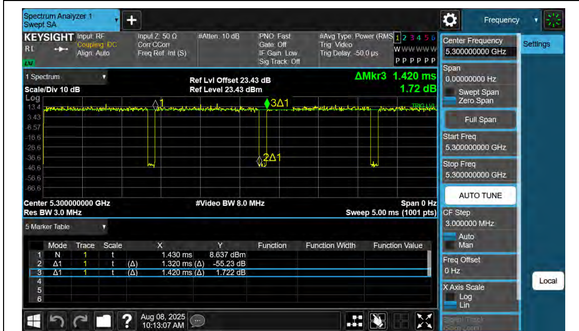
NTNV-11AC20SISO-Ant2-5300
