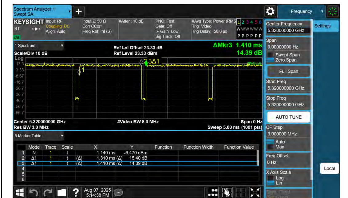
NTNV-11N20SISO-Ant2-5320
