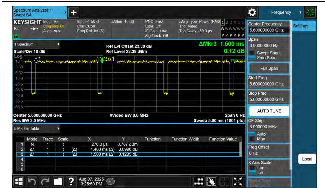
NTNV-11A-Ant2-5600
