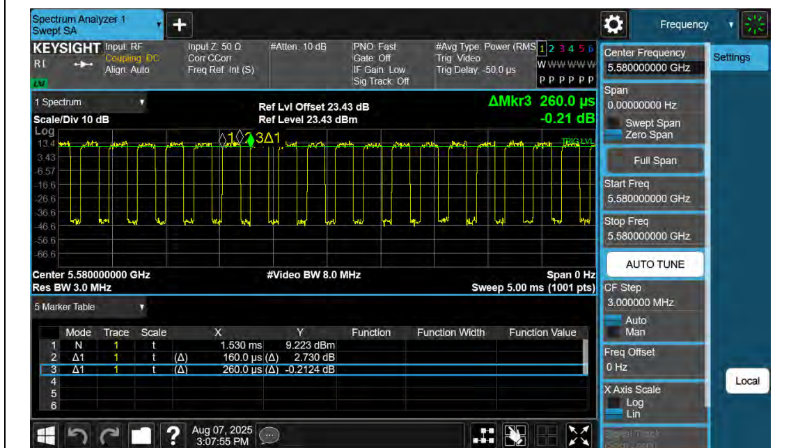
NTNV-11N20SISO-Ant2-5580
