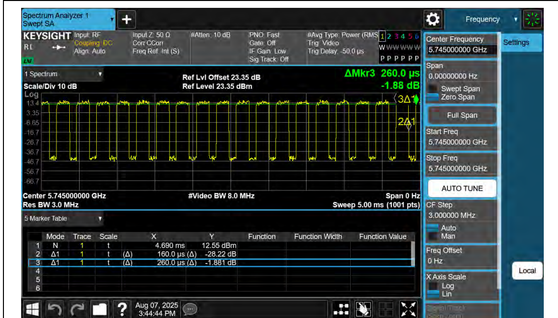
NTNV-11N20SISO-Ant2-5745
