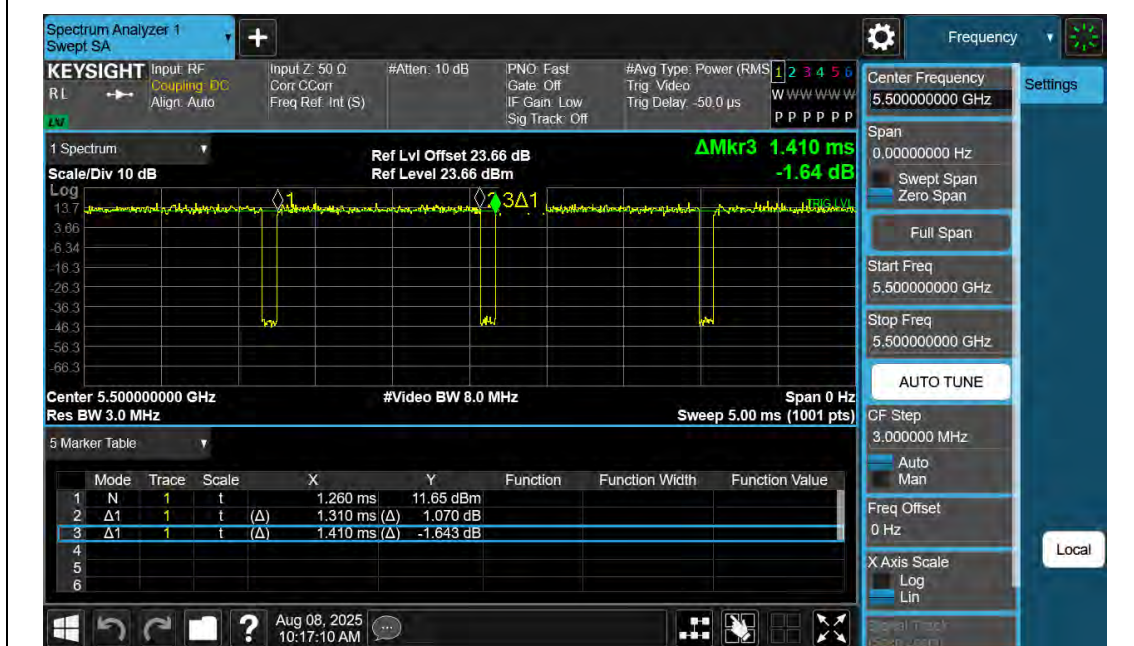
NTNV-11AC20SISO-Ant2-5500
