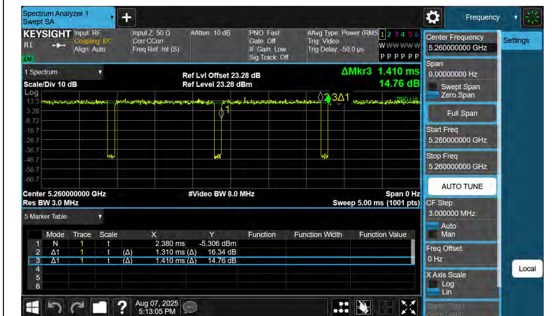
NTNV-11N20SISO-Ant2-5260
