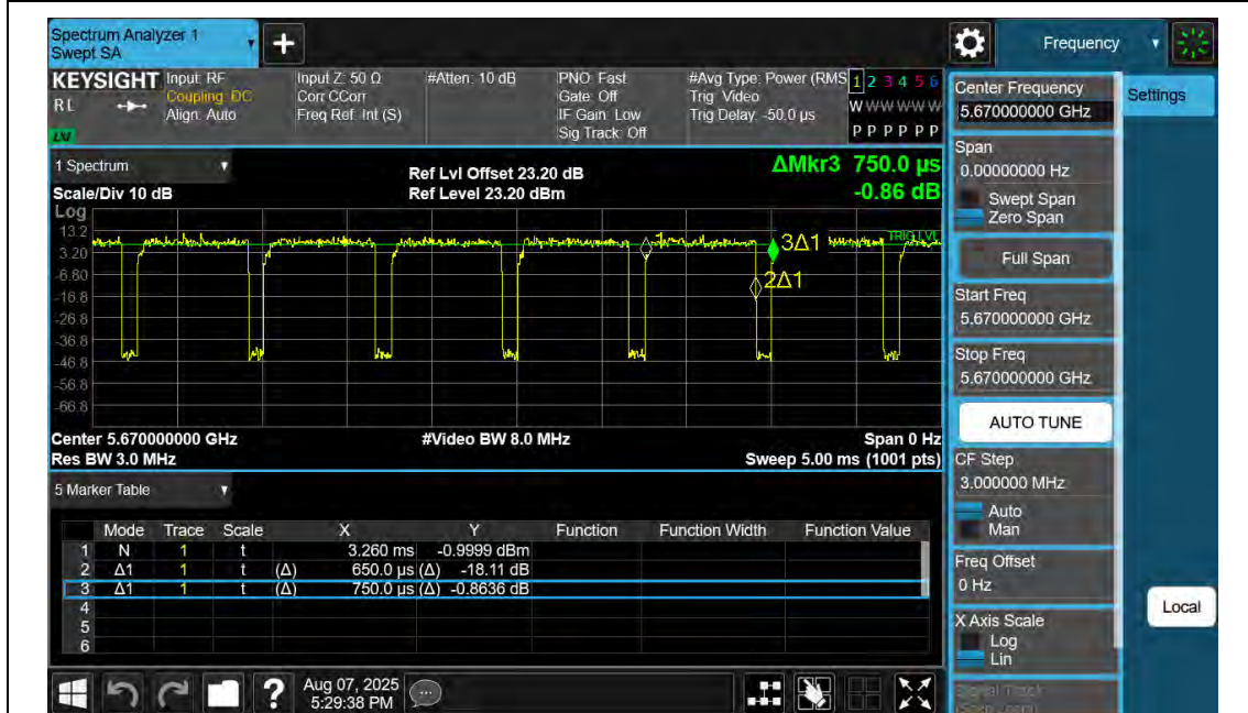
NTNV-11N40SISO-Ant2-5670
