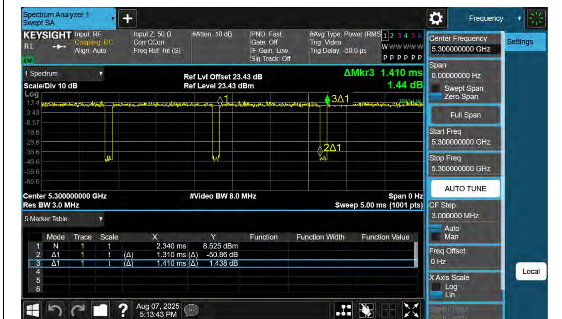
NTNV-11N20SISO-Ant2-5300
