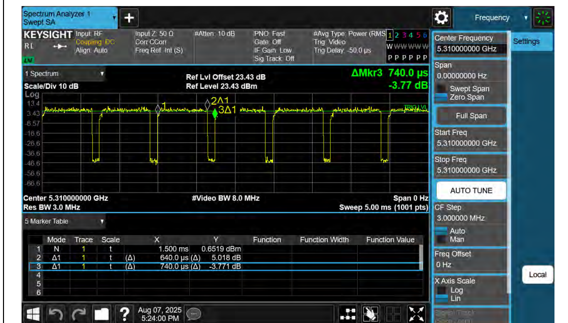
NTNV-11N40SISO-Ant2-5310
