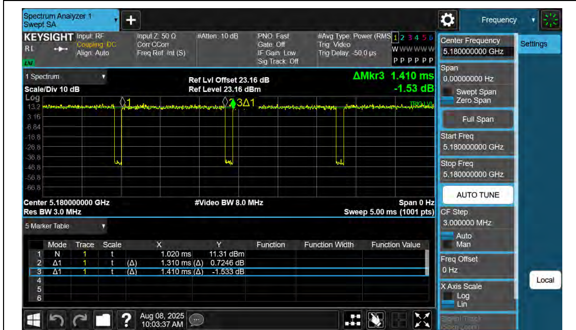
NTNV-11AC20SISO-Ant2-5180
