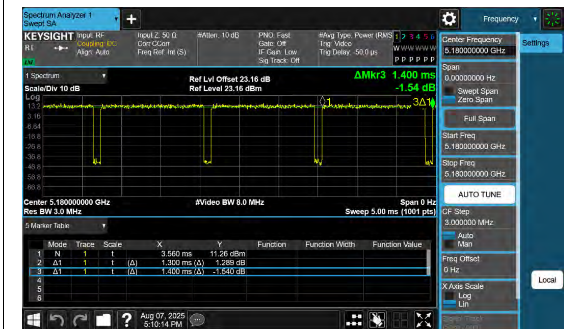
NTNV-11N20SISO-Ant2-5180
