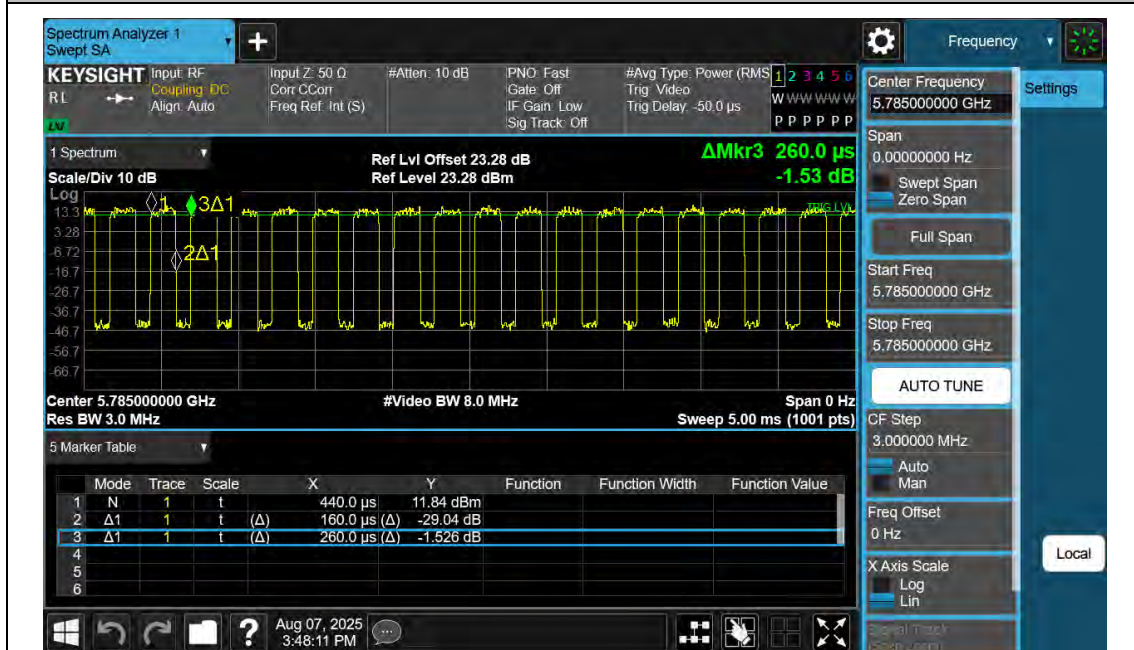
NTNV-11N20SISO-Ant2-5785
