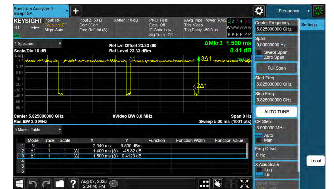
NTNV-11A-Ant2-5825
