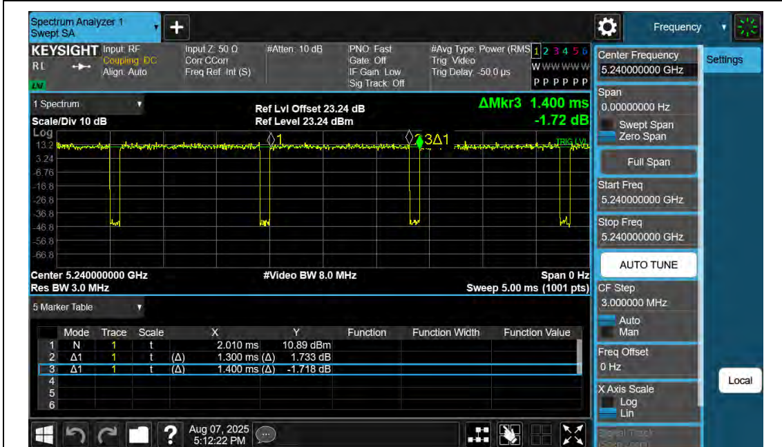
NTNV-11N20SISO-Ant2-5240
