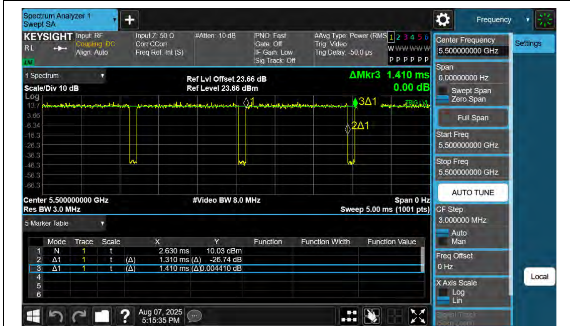
NTNV-11N20SISO-Ant2-5500
