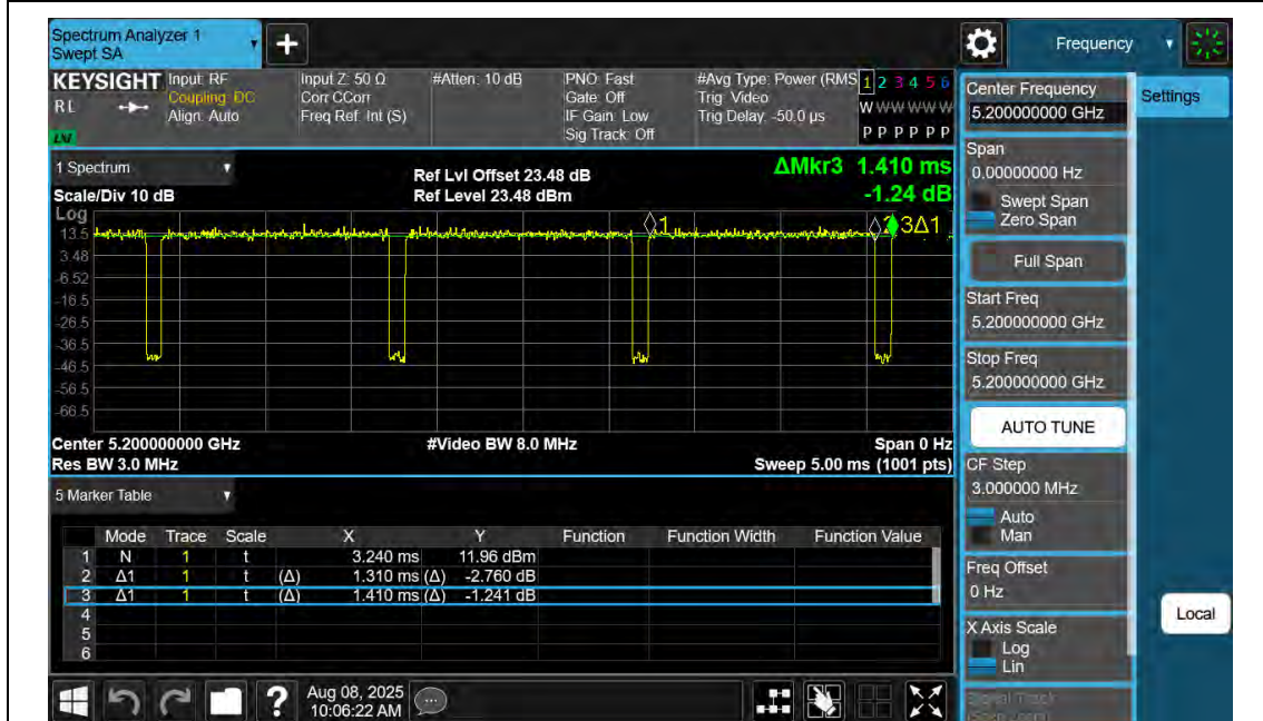
NTNV-11AC20SISO-Ant2-5200
