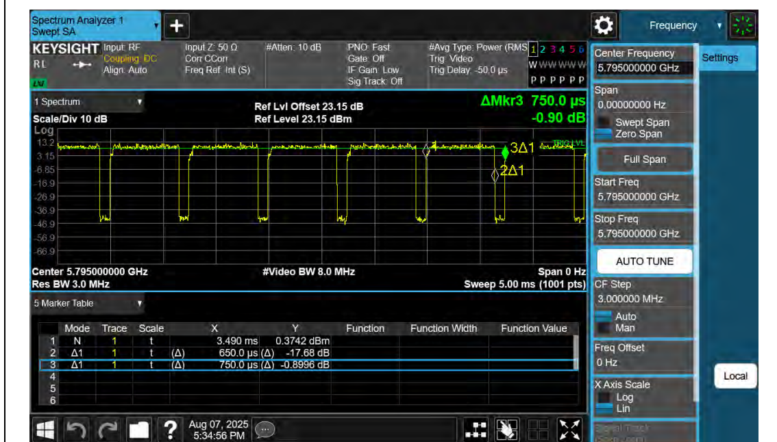
NTNV-11N40SISO-Ant2-5795
