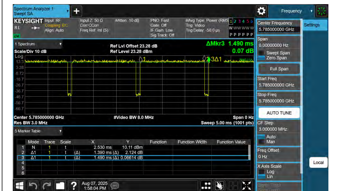
NTNV-11A-Ant2-5785
