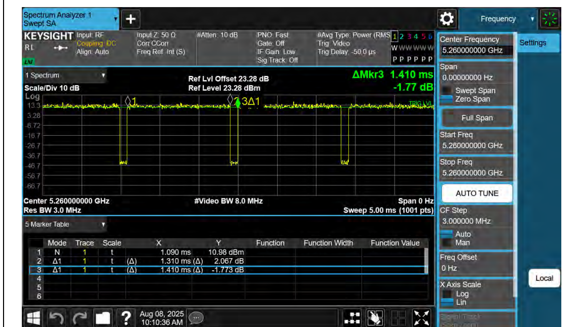
NTNV-11AC20SISO-Ant2-5260
