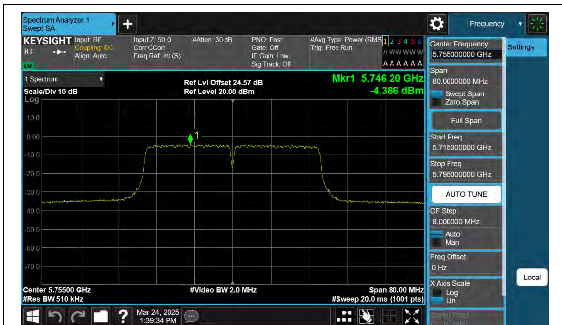
11AC40SISO-Ant2-5755-PASS
