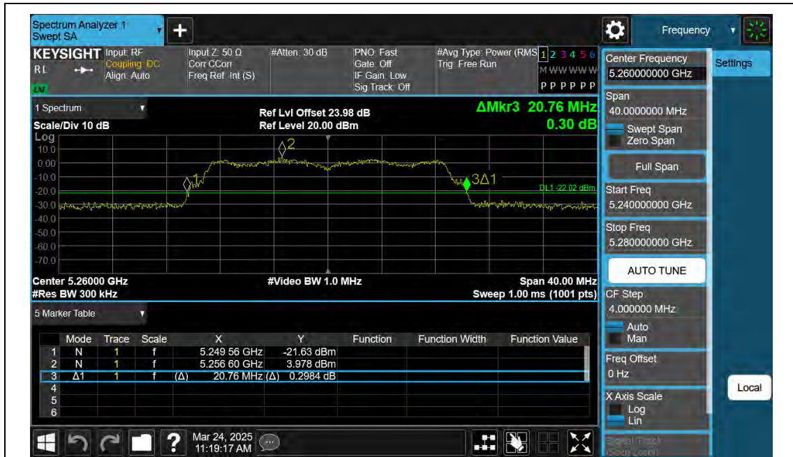
11AC20SISO-Ant2-5260
