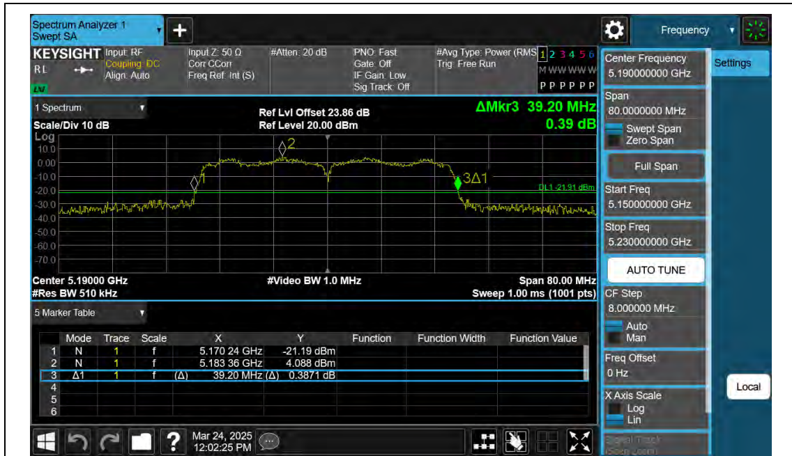
11AC40SISO-Ant2-5190
