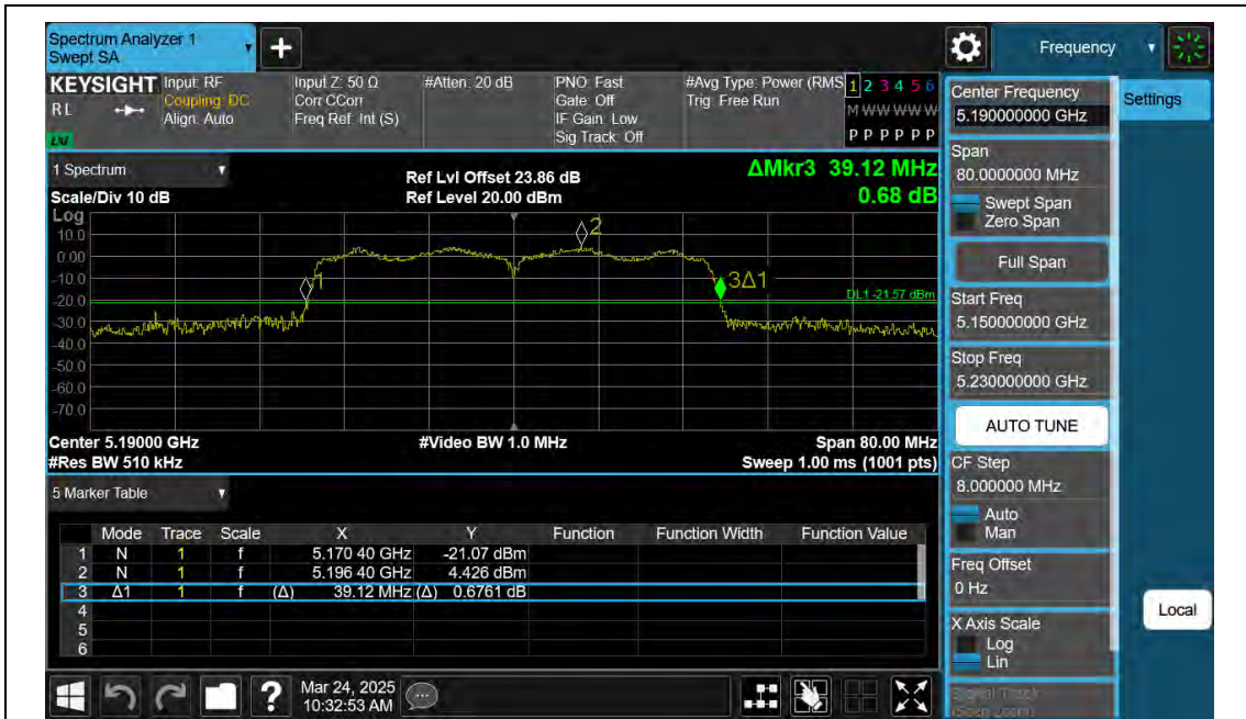
11N40SISO-Ant2-5190
