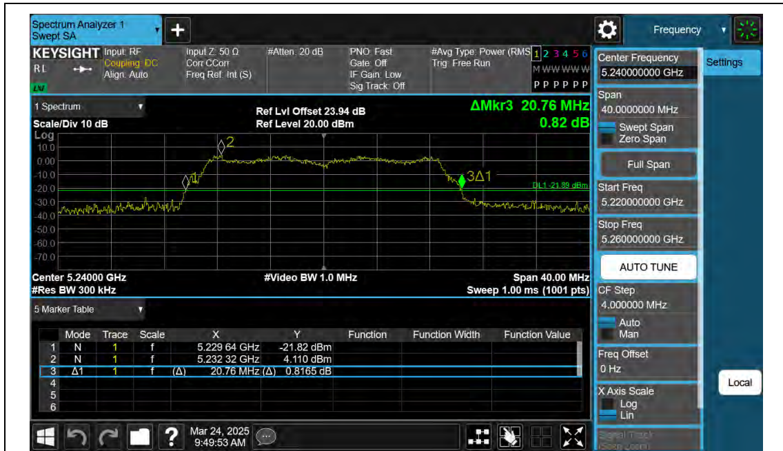
11N20SISO-Ant2-5240
