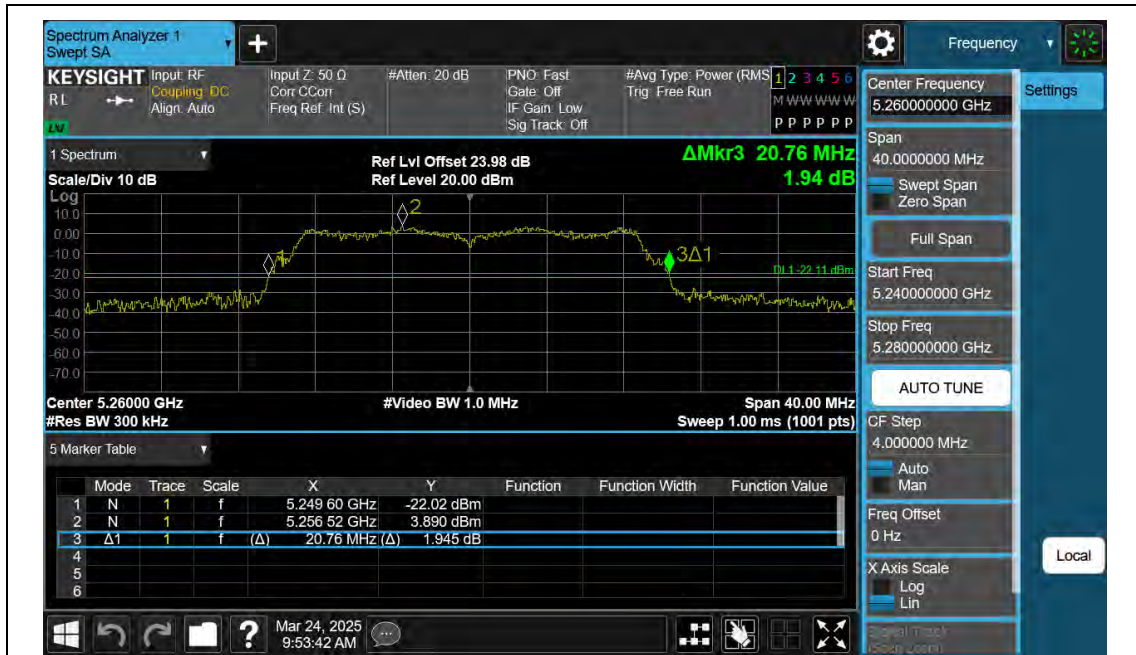
11N20SISO-Ant2-5260
