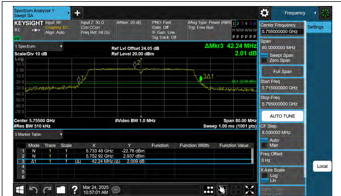
11N40SISO-Ant2-5755
