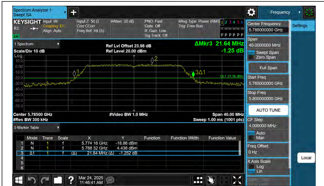
11AC20SISO-Ant2-5785
