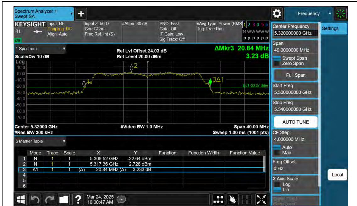
11N20SISO-Ant2-5320
