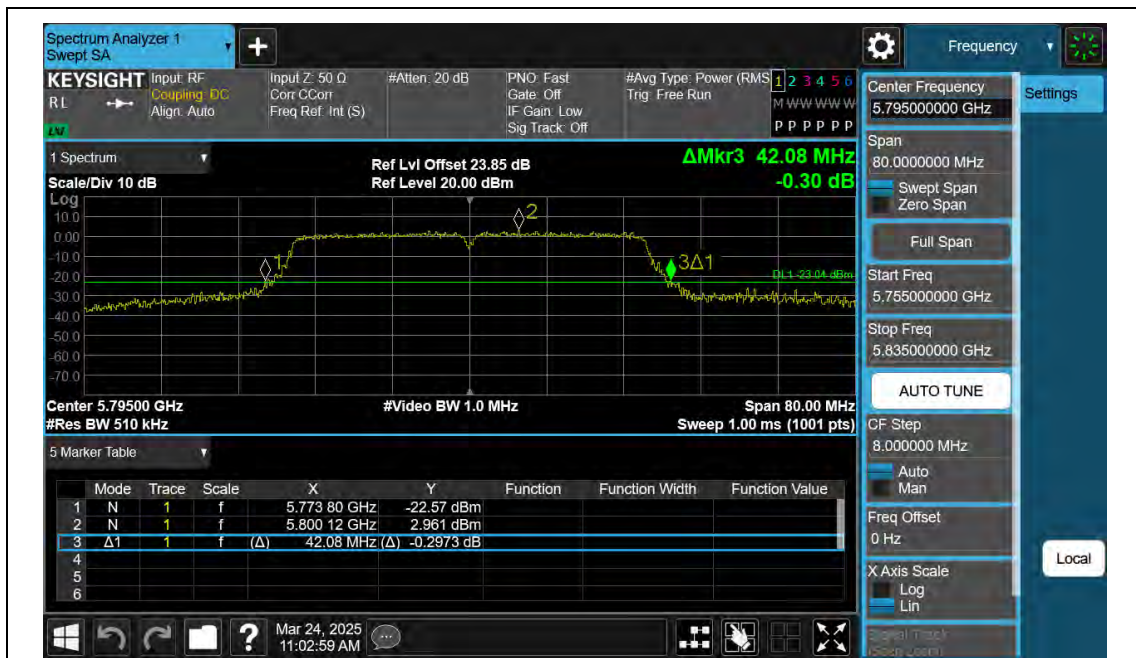
11N40SISO-Ant2-5795
