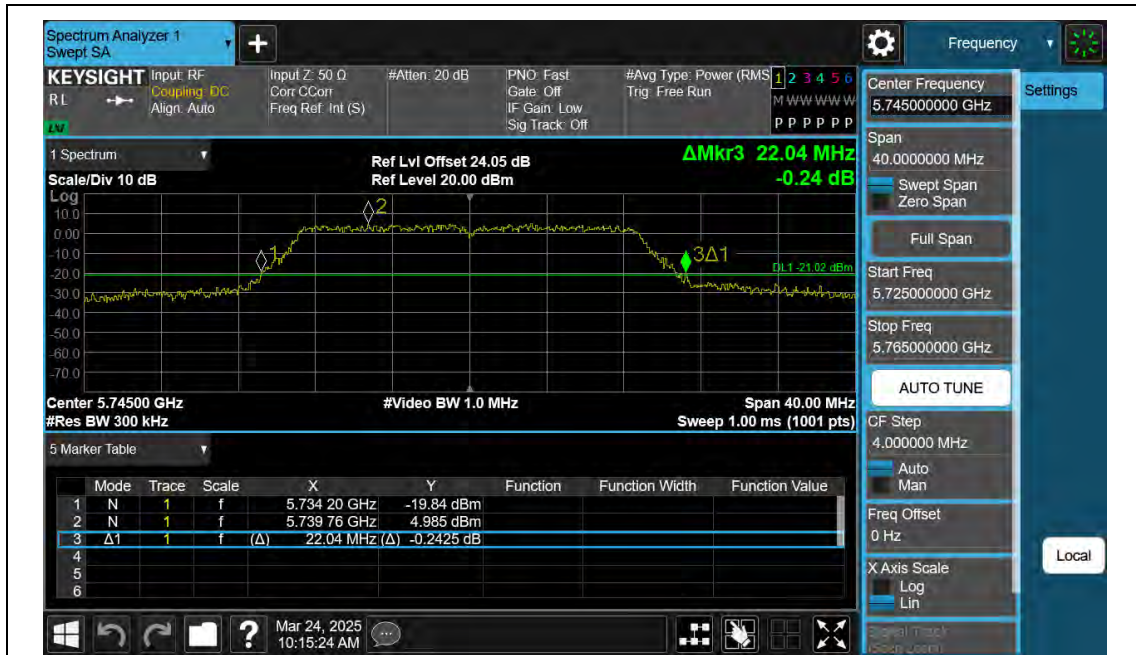
11N20SISO-Ant2-5745
