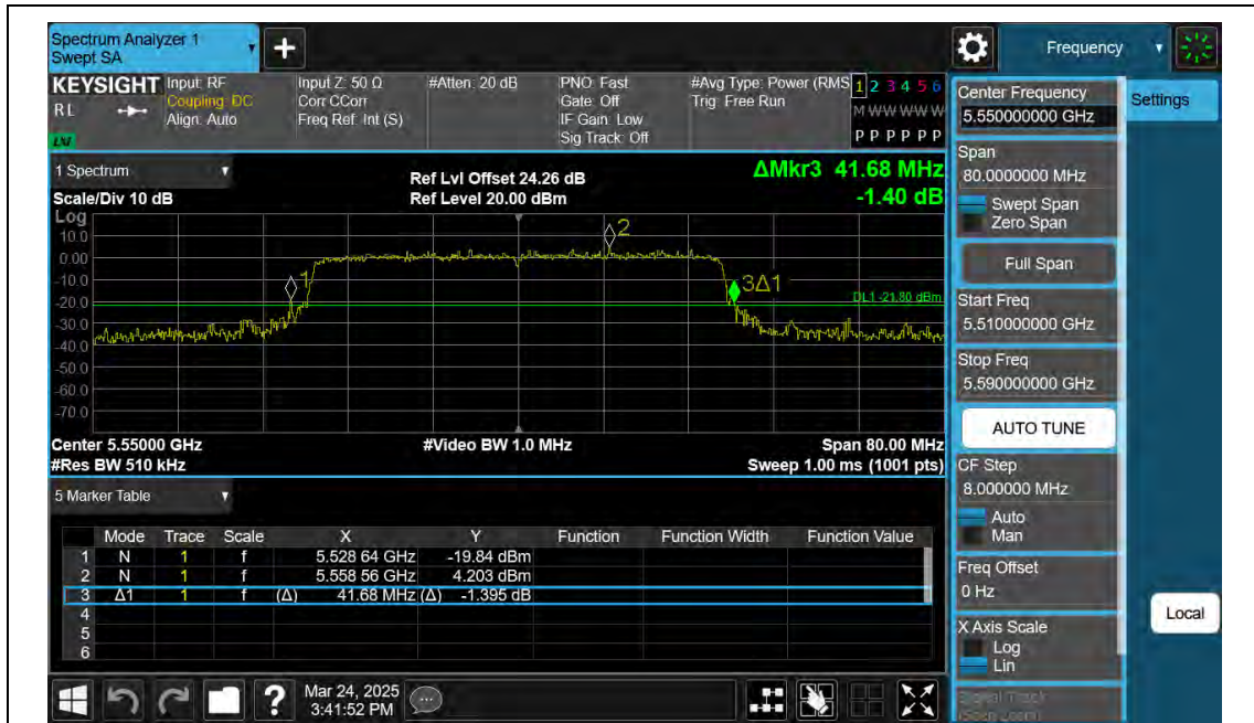
11AX40SISO-Ant2-5550
