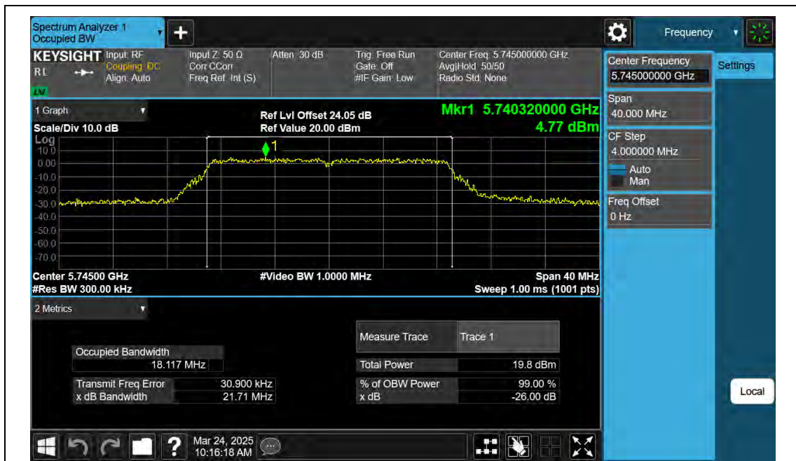
11N20SISO-Ant2-5745
