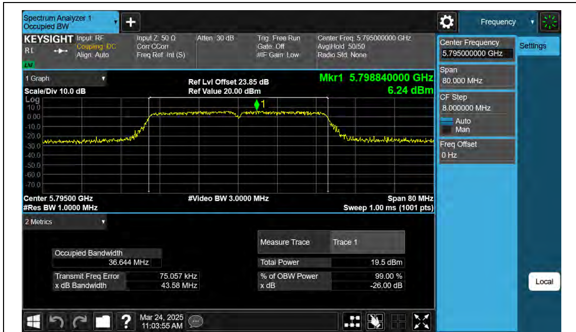
11N40SISO-Ant2-5795
