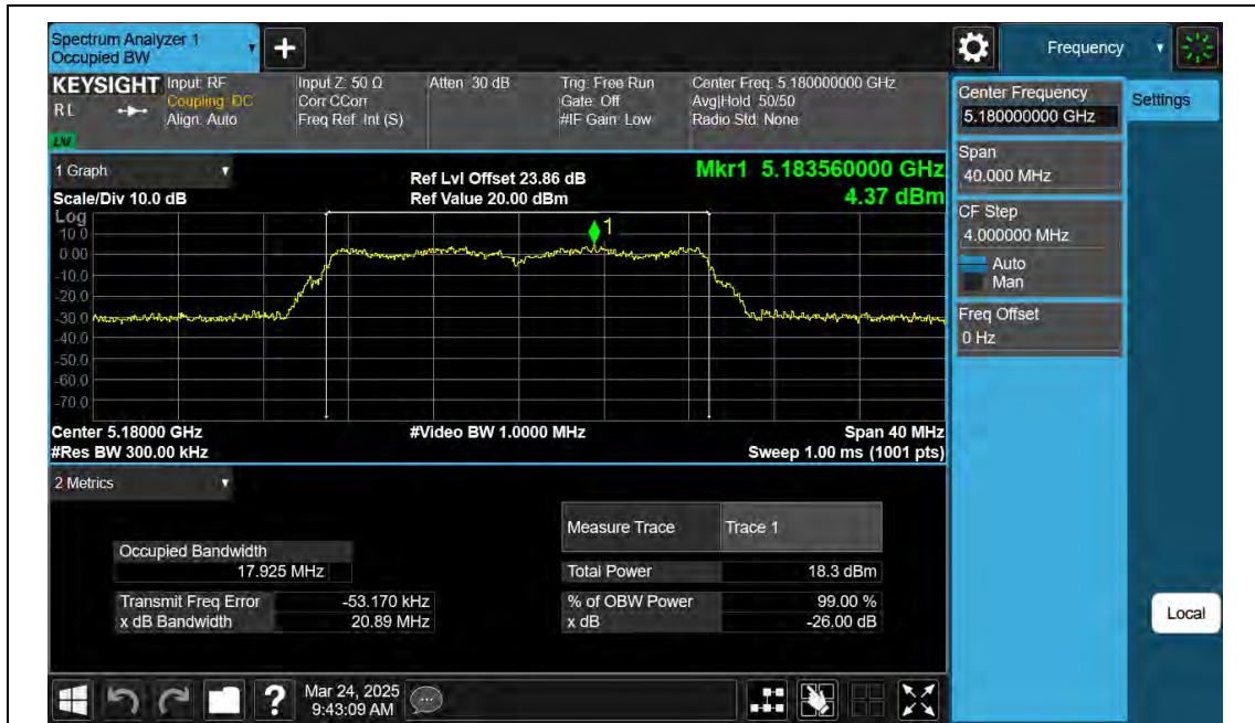
11N20SISO-Ant2-5180
