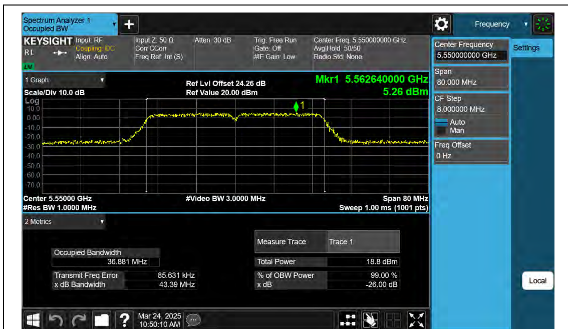
11N40SISO-Ant2-5550
