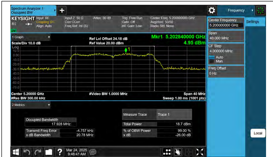
11N20SISO-Ant2-5200
