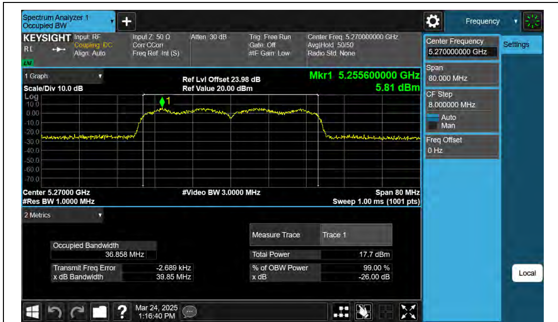
11AC40SISO-Ant2-5270
