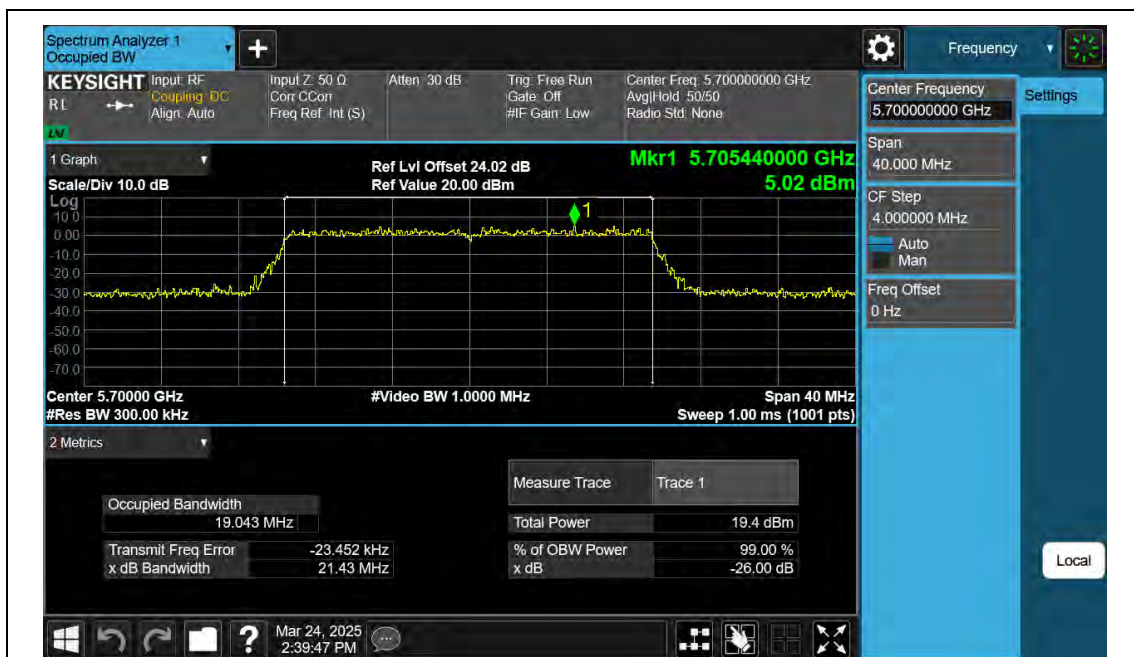
11AX20SISO-Ant2-5700
