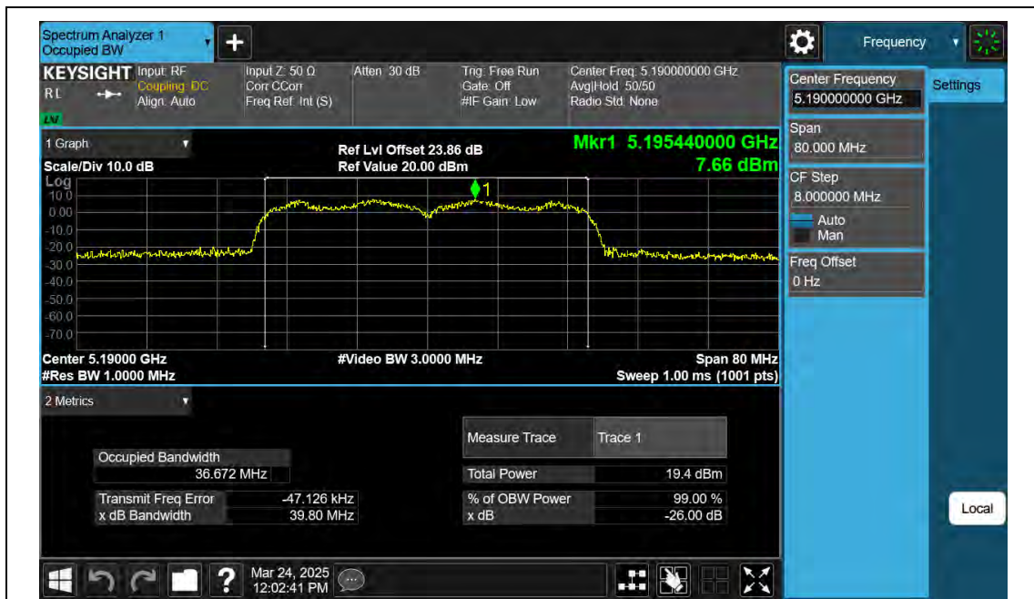
11AC40SISO-Ant2-5190
