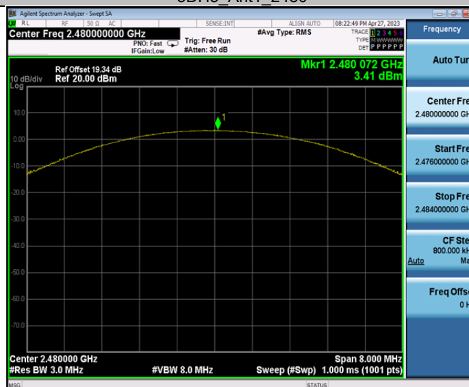
3DH5_Ant1_2480
