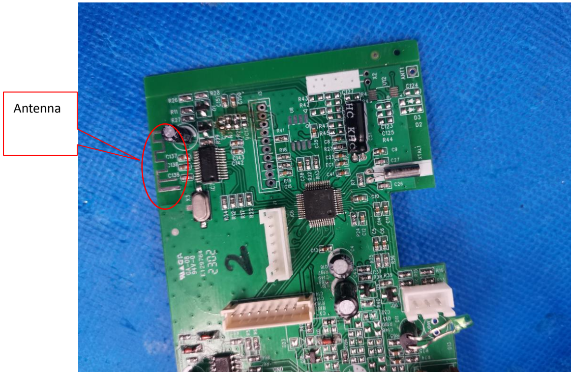
INTERNAL VIEW OF EUT (FIGURE 8)
