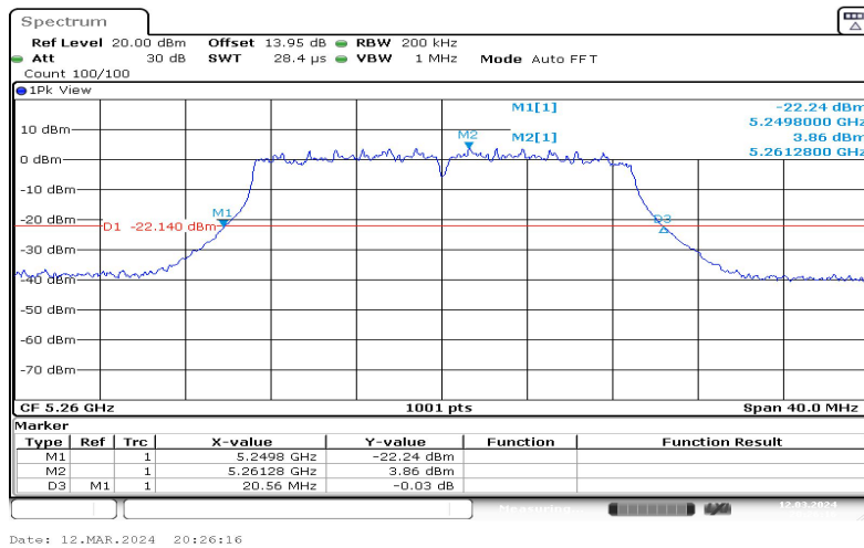
11N20SISO-Ant1-5260
