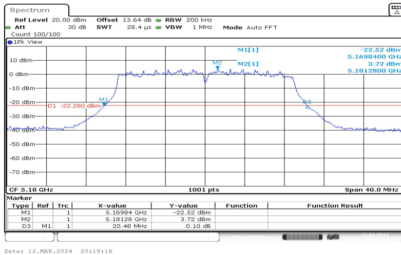
11N20SISO-Ant1-5180
