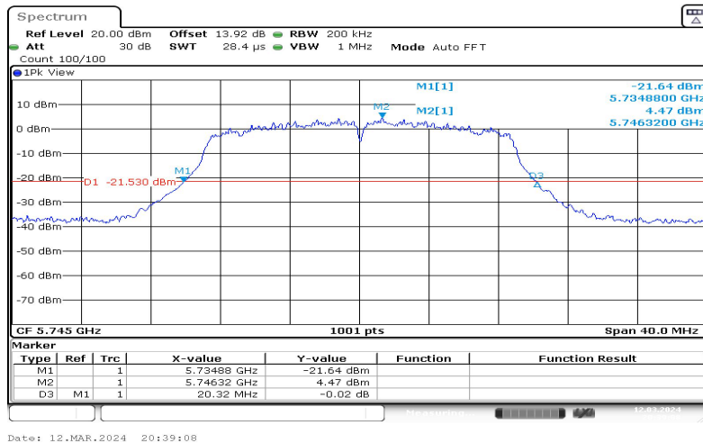
11N20SISO-Ant1-5745
