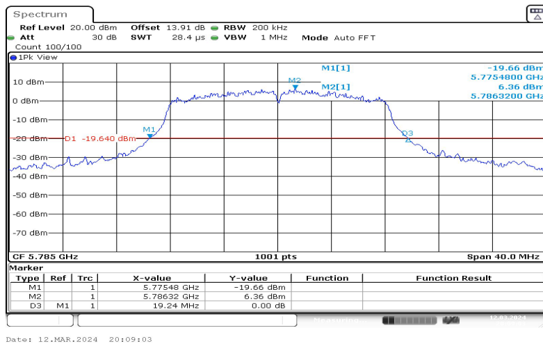
11A-Ant1-5785
