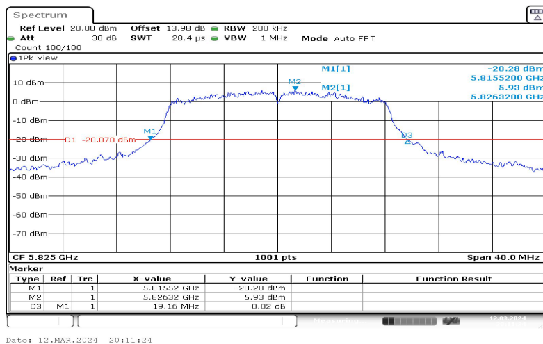
11A-Ant1-5825
