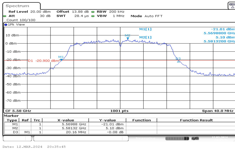
11N20SISO-Ant1-5580
