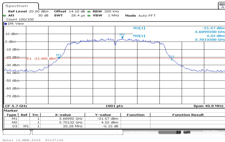
11N20SISO-Ant1-5700
