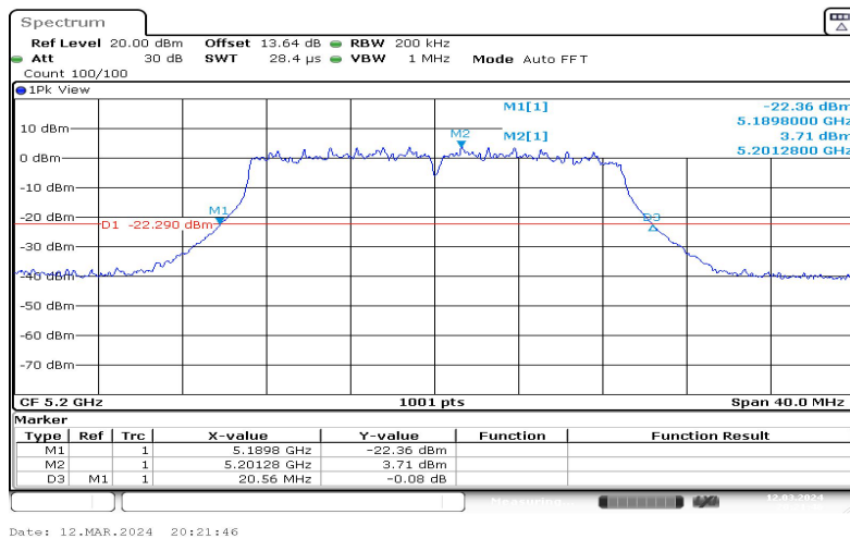
11N20SISO-Ant1-5200
