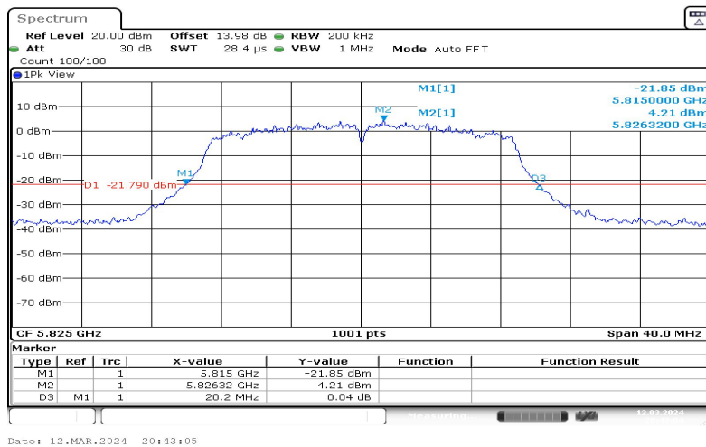
11N20SISO-Ant1-5825
