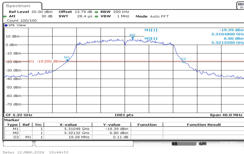
11A-Ant1-5320
