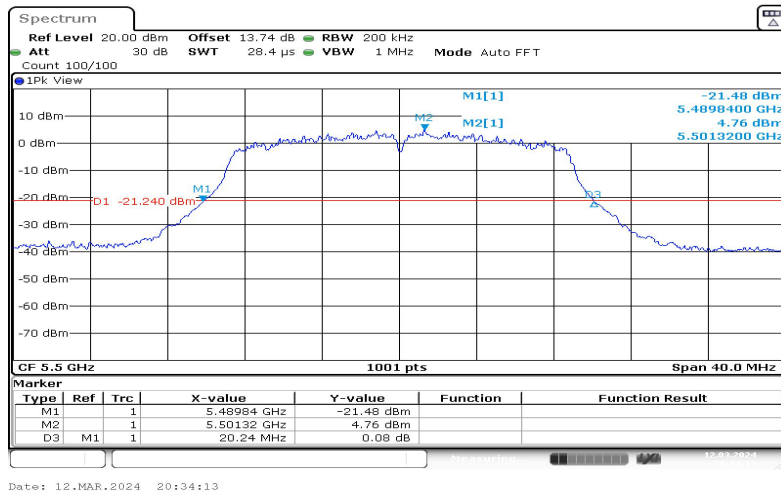
11N20SISO-Ant1-5500
