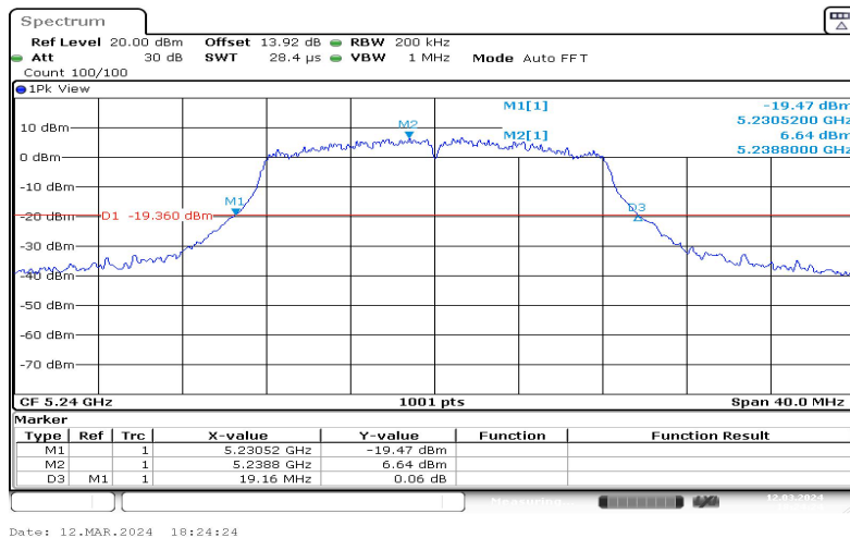
11A-Ant1-5240
