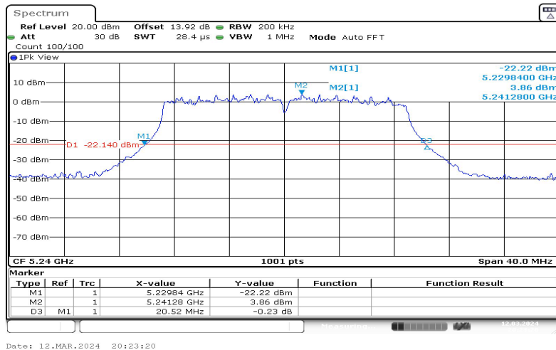
11N20SISO-Ant1-5240
