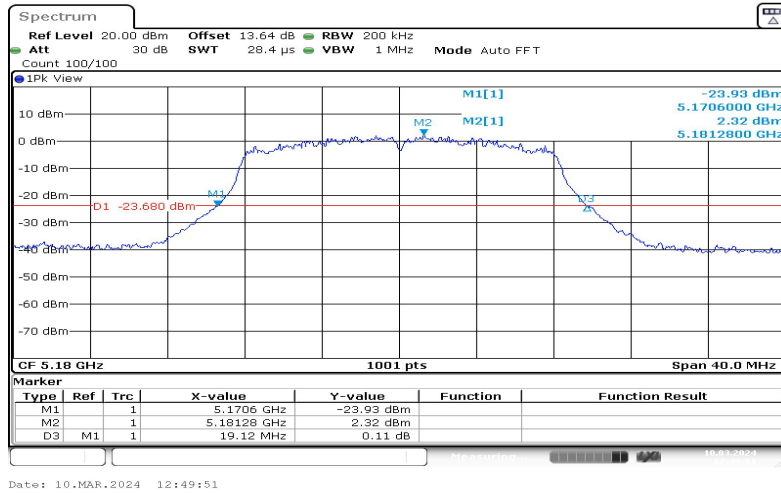
11A-Ant1-5180
