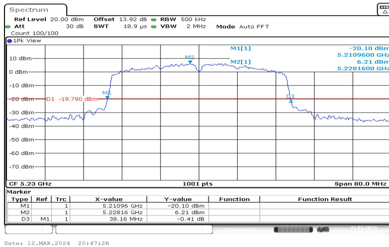
11N40SISO-Ant1-5230
