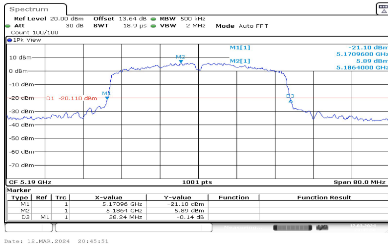
11N40SISO-Ant1-5190
