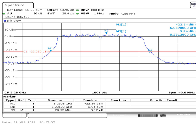
11N20SISO-Ant1-5280
