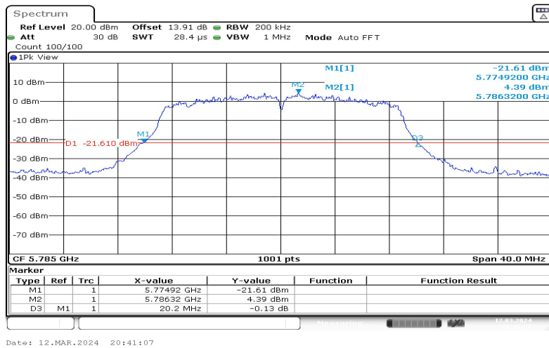
11N20SISO-Ant1-5785
