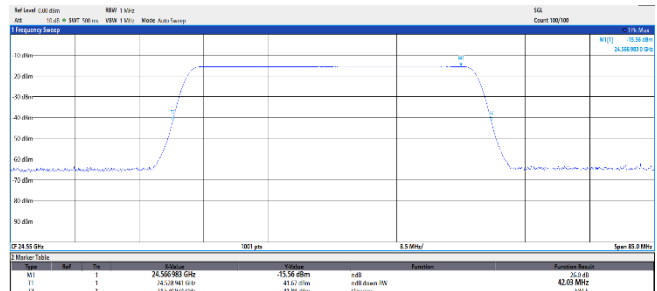
Figure 8.2-2: 26 dB OBW Middle channel: 24.55 GHz 16.67 μs with 43MHz authorized Bandwidth
