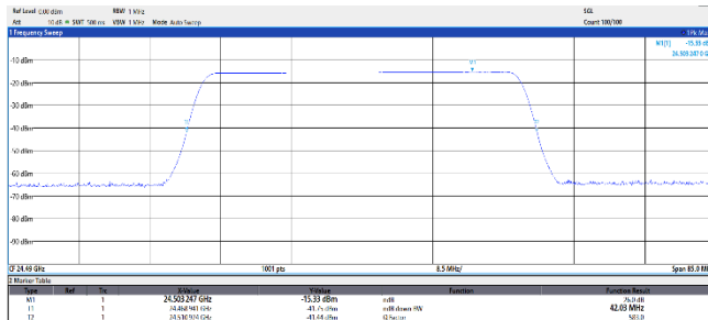
Figure 8.2-1: 26 dB OBW Low channel: 24.49 GHz 16.67 μs with 43MHz authorized Bandwidth
