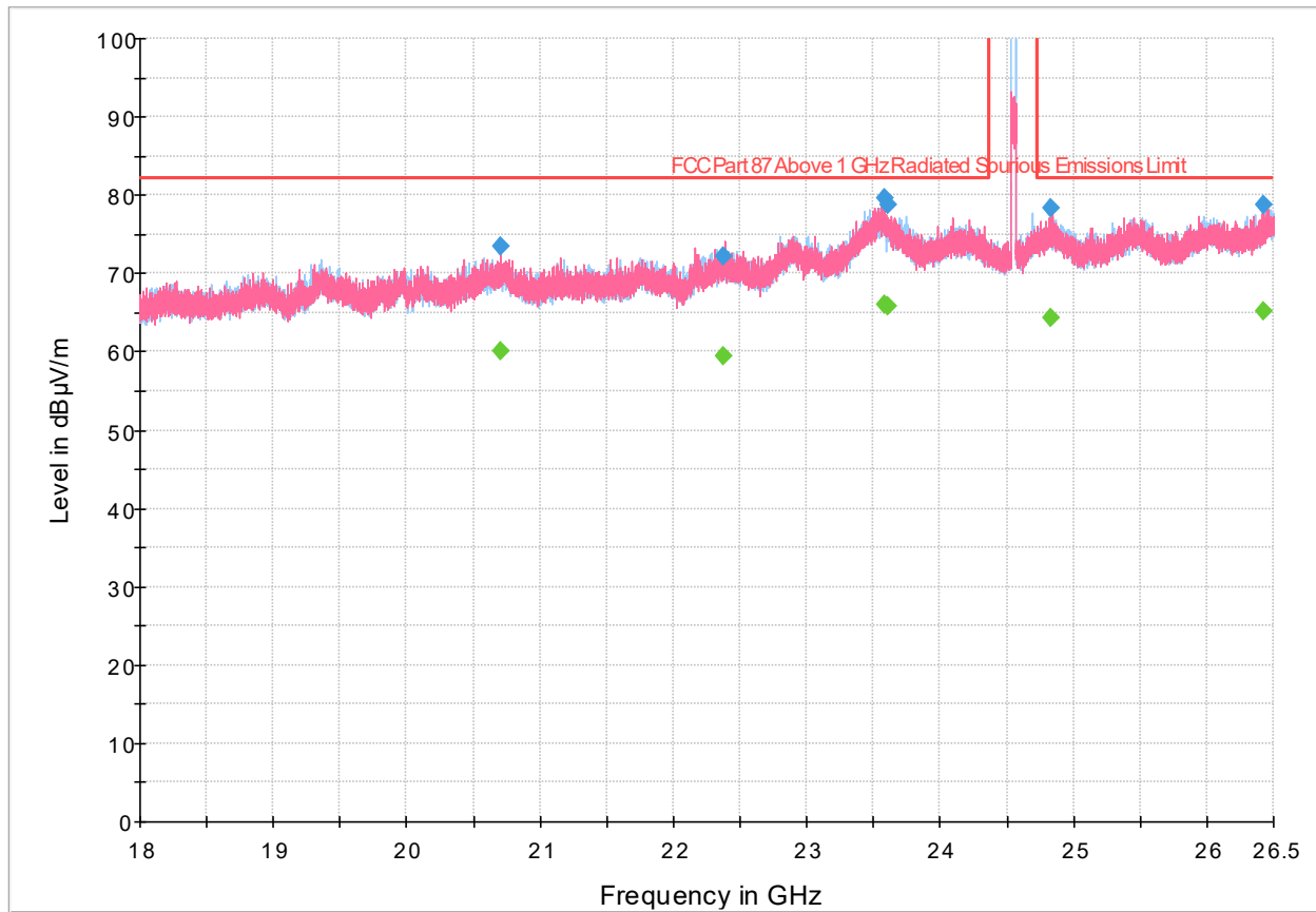
Figure 8.5-8: Radiated emissions spectral plot (18 GHz - 26.5 GHz) 24.55GHz Middle channel with 43MHz authorized Bandwidth
