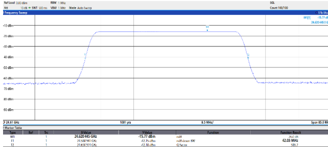
Figure 8.2-3: 26 dB OBW High channel: 24.61 GHz 16.67 μs with 43MHz authorized Bandwidth
