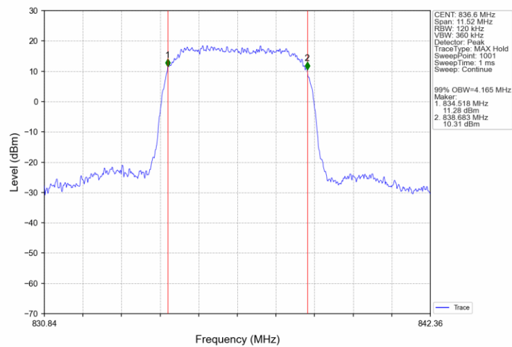
Band5_RMC_MCH_836.6MHz_12.2kbps RMC_NTNV
