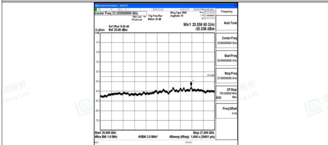
Band7_20MHz_16QAM_20850_1RB#0_20000~27000_20000~27000
