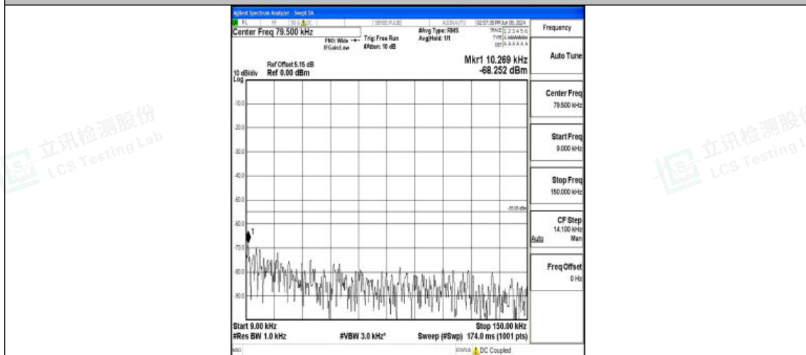
Band7_10MHz_QPSK_21100_1RB#0_0.009~0.15_0.009~0.15
