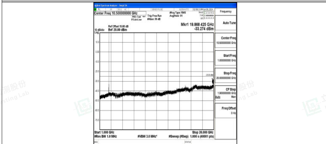
Band7_10MHz_16QAM_21100_1RB#0_1000~20000_1000~20000
