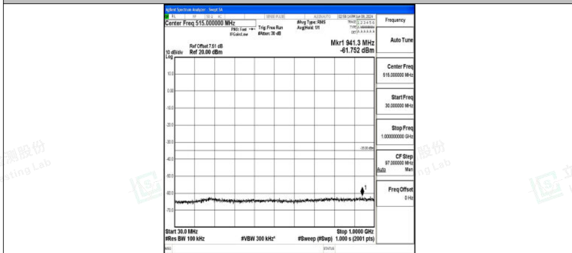
Band7_10MHz_16QAM_21400_1RB#0_30~1000_30~1000
