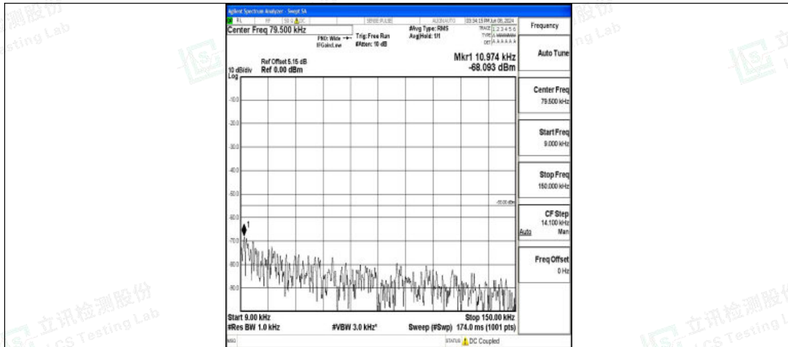
Band7_20MHz_16QAM_20850_1RB#0_0.009~0.15_0.009~0.15
