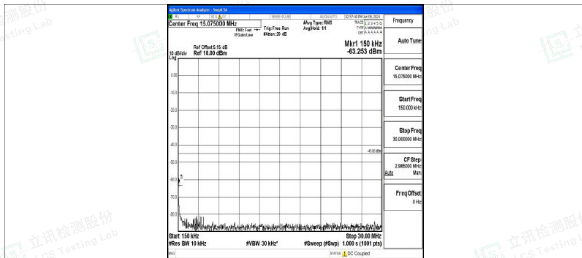
Band7_10MHz_QPSK_21100_1RB#0_0.15~30_0.15~30
