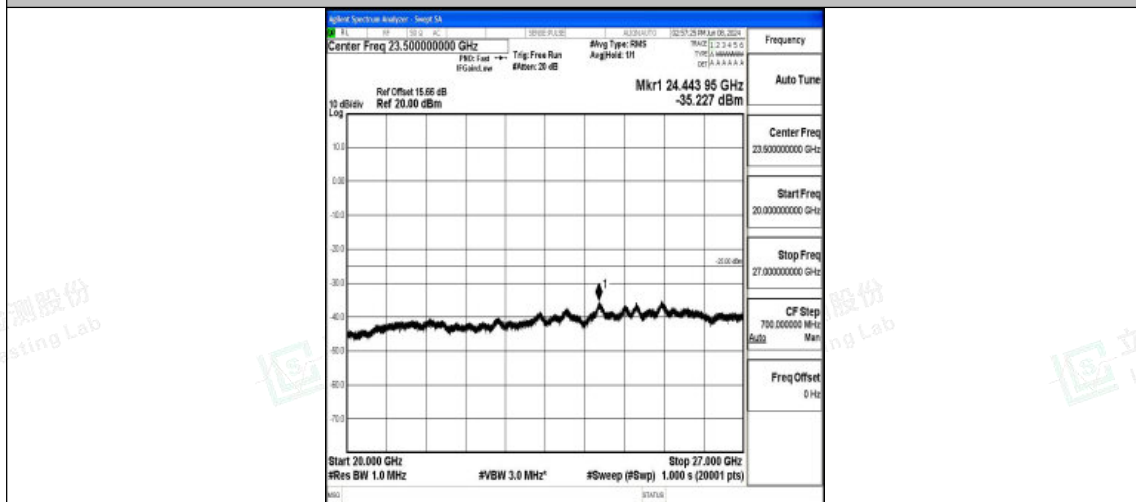
Band7_10MHz_16QAM_20800_1RB#0_20000~27000_20000~27000
