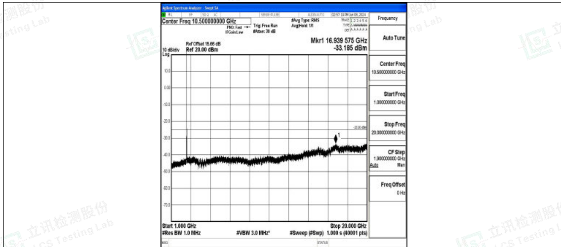
Band7_10MHz_16QAM_20800_1RB#0_1000~20000_1000~20000
