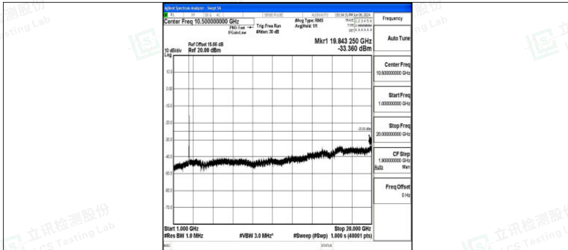
Band7_20MHz_16QAM_20850_1RB#0_1000~20000_1000~20000
