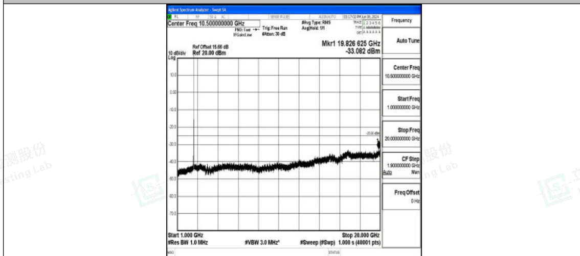
Band7_15MHz_16QAM_21100_1RB#0_1000~20000_1000~20000
