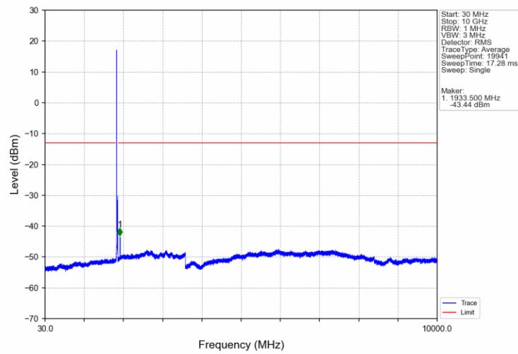
Band2_15MHz_16QAM_LCH_1857.5MHz_RB_1_0_NTNV
