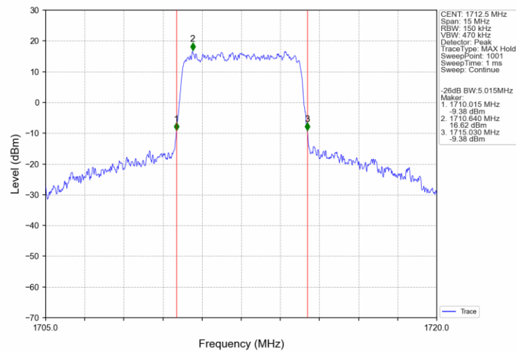
Band4 5MHz 16QAM LCH 1712.5MHz RB 25 0 NTN
