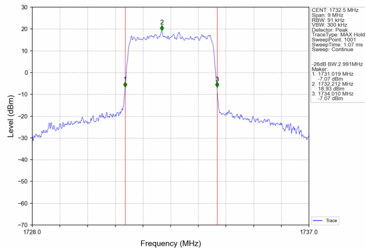
Band4 3MHz QPSK MCH 1732.5MHz RB 15 0 NTNV
