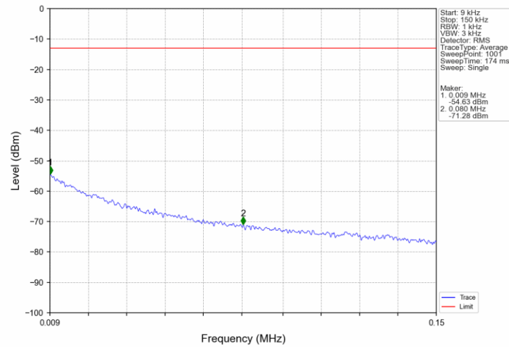
Band4 5MHz 16QAM MCH 1732.5MHz RB 1 0 NTNV
