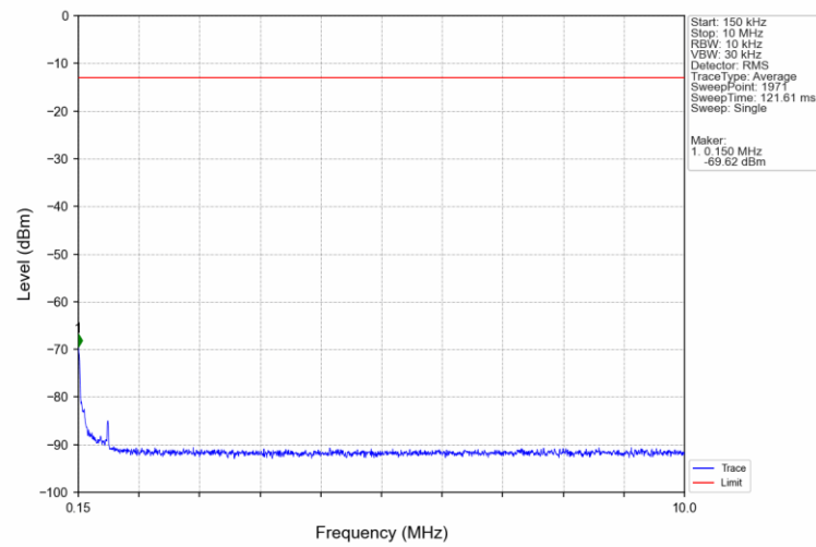
Band4 5MHz 16QAM MCH 1732.5MHz RB 1 0 NTNV
