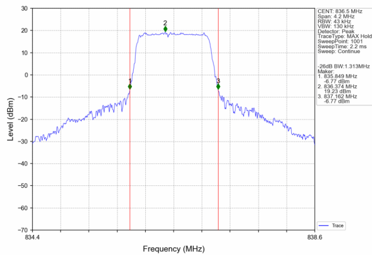
Band5 1.4MHz QPSK MCH 836.5MHz RB 6 0 NTN
