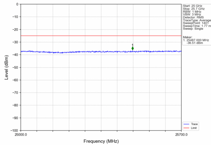
Band7 5MHz QPSK MCH 2535MHz RB 1 0 NTNV
