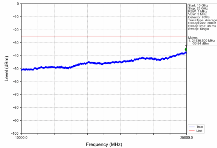
Band7 5MHz QPSK MCH 2535MHz RB 1 0 NTNV
